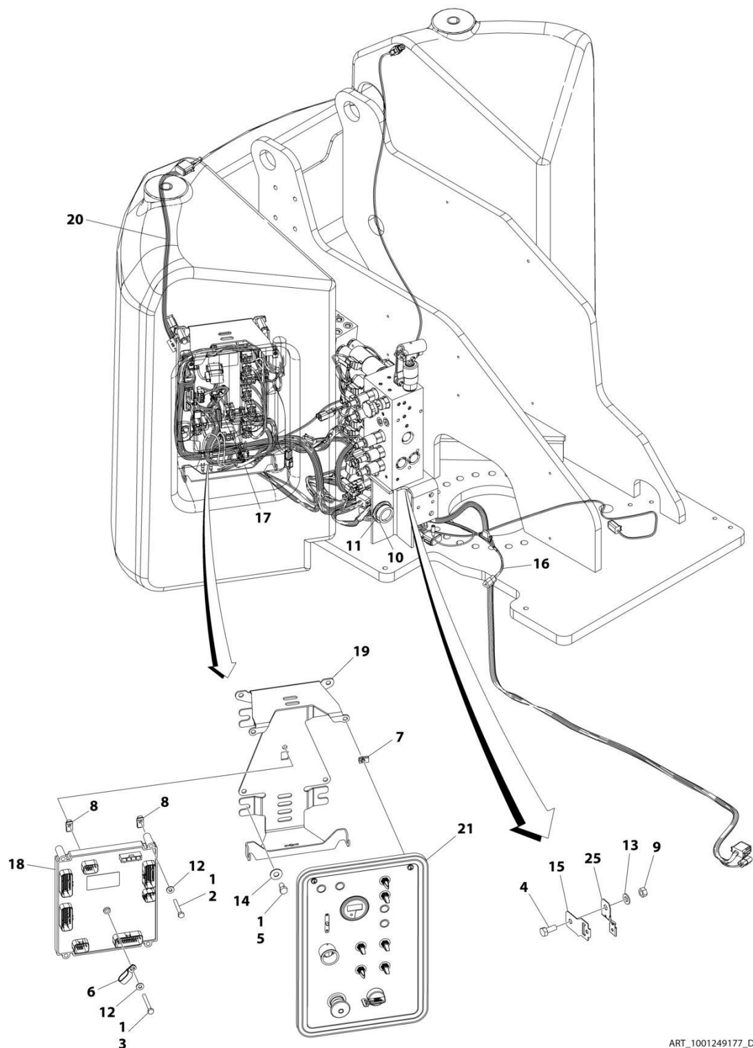
FIGURE 2-15. GROUND CONTROL BOX INSTALLATION - E400ANARROW (CE & UK CA SPEC) (SN 0300298643 to Present)
