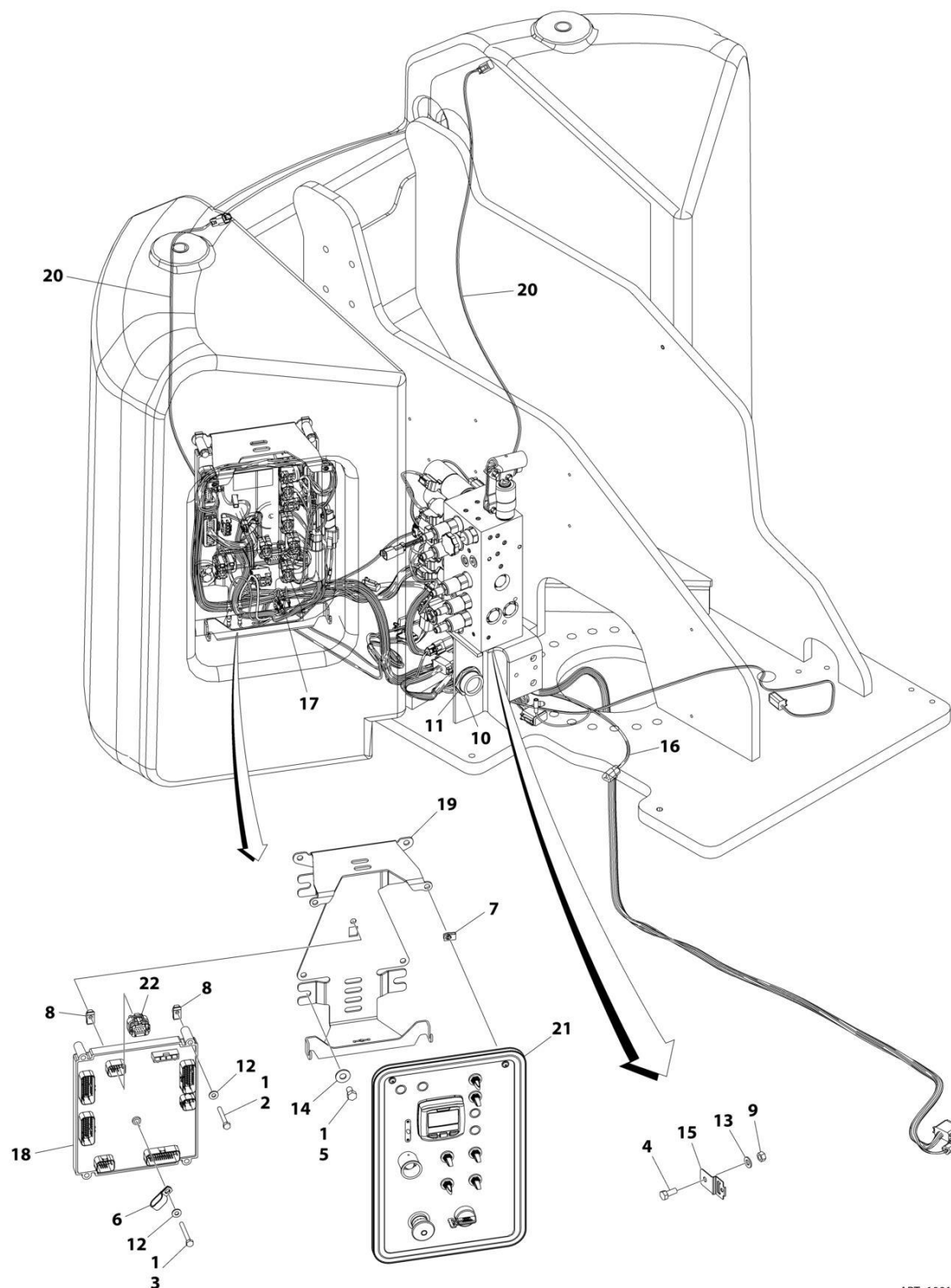
FIGURE 2-14. GROUND CONTROL BOX INSTALLATION - E400ANARROW (CE & UK CA SPEC) (Prior to SN 0300298643)
