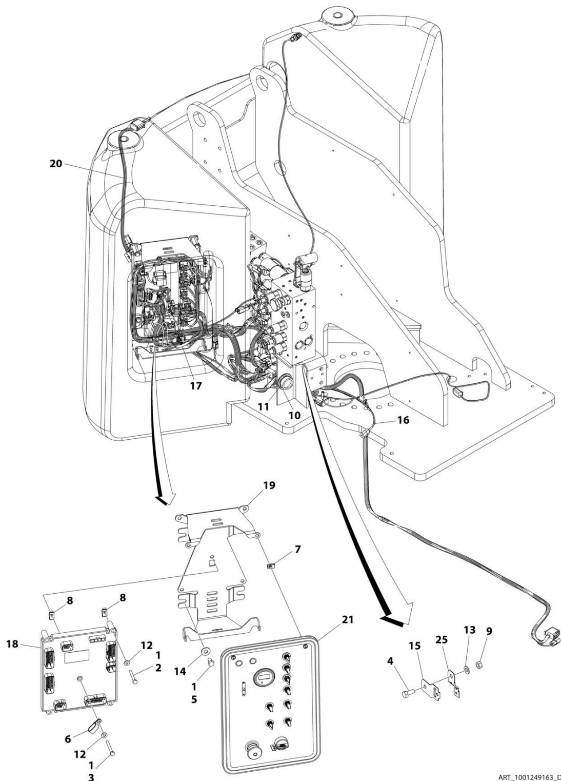
FIGURE 2-17. GROUND CONTROL BOX INSTALLATION - E400AJPNARROW (ALL SPECS EXCEPT CE & UK CA SPEC) (SN 0300298643 to Present)
