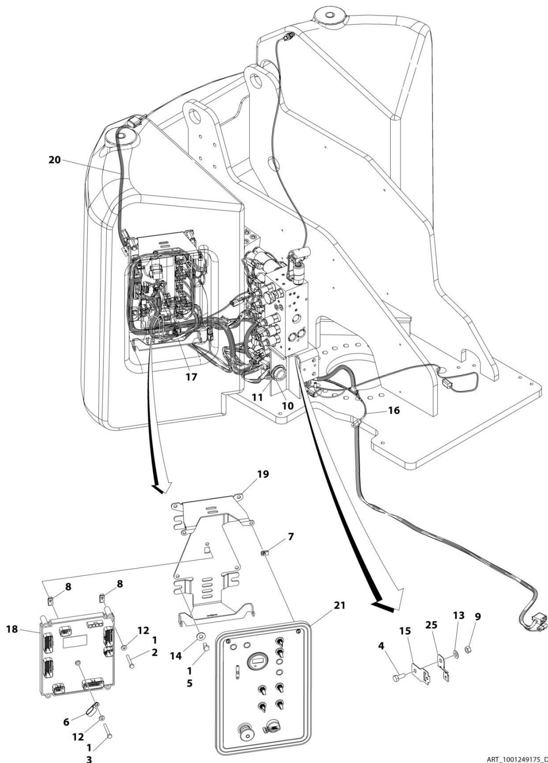
FIGURE 2-13. GROUND CONTROL BOX INSTALLATION - E400ANARROW (ALL SPECS EXCEPT AUSTRALIAN, CE & UK CA SPECS) (SN 0300298643 to Present)
