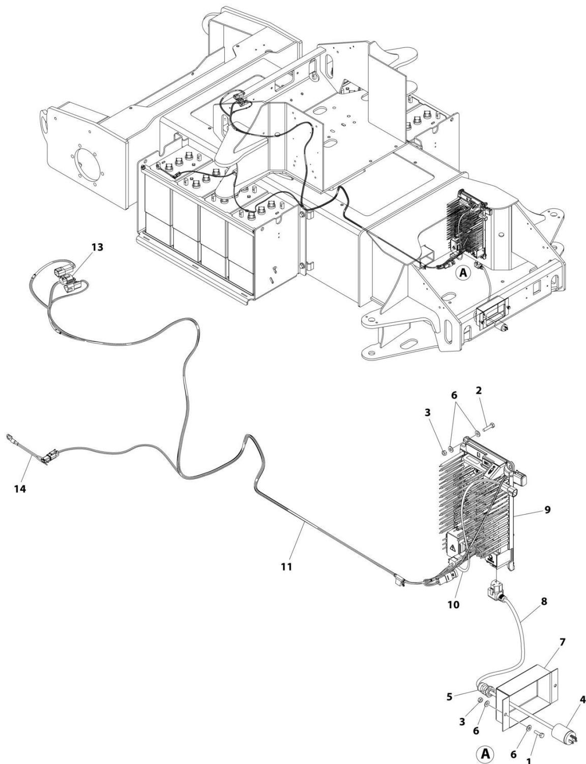
FIGURE 1-23. BATTERY CHARGER INSTALLATION (ALL SPECS EXCEPT AUSTRALIAN, CE & UK CA SPECS) (SN 0300298643 to Present)
