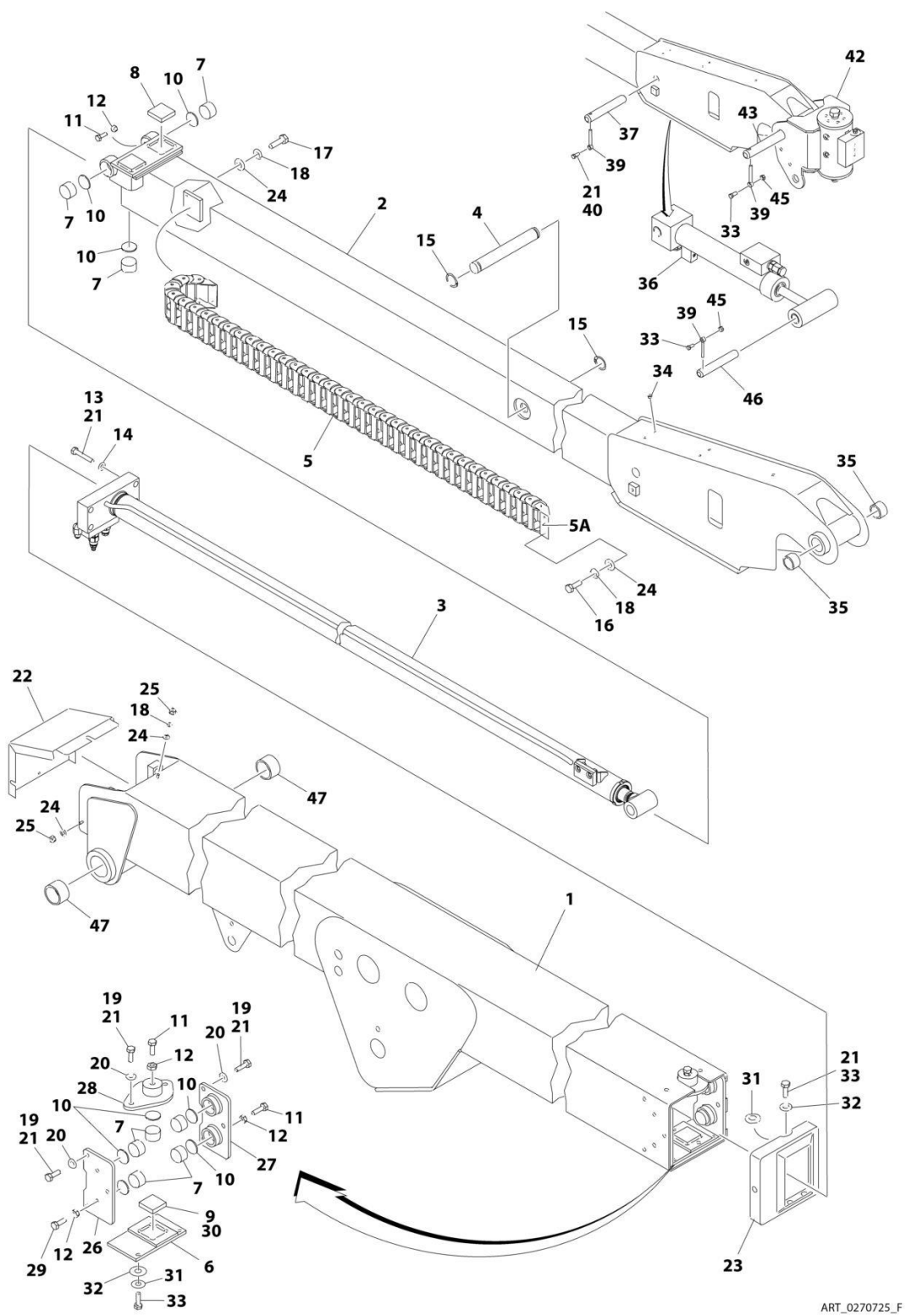
FIGURE 3-3. MAIN BOOM ASSEMBLY - E400ANARROW
