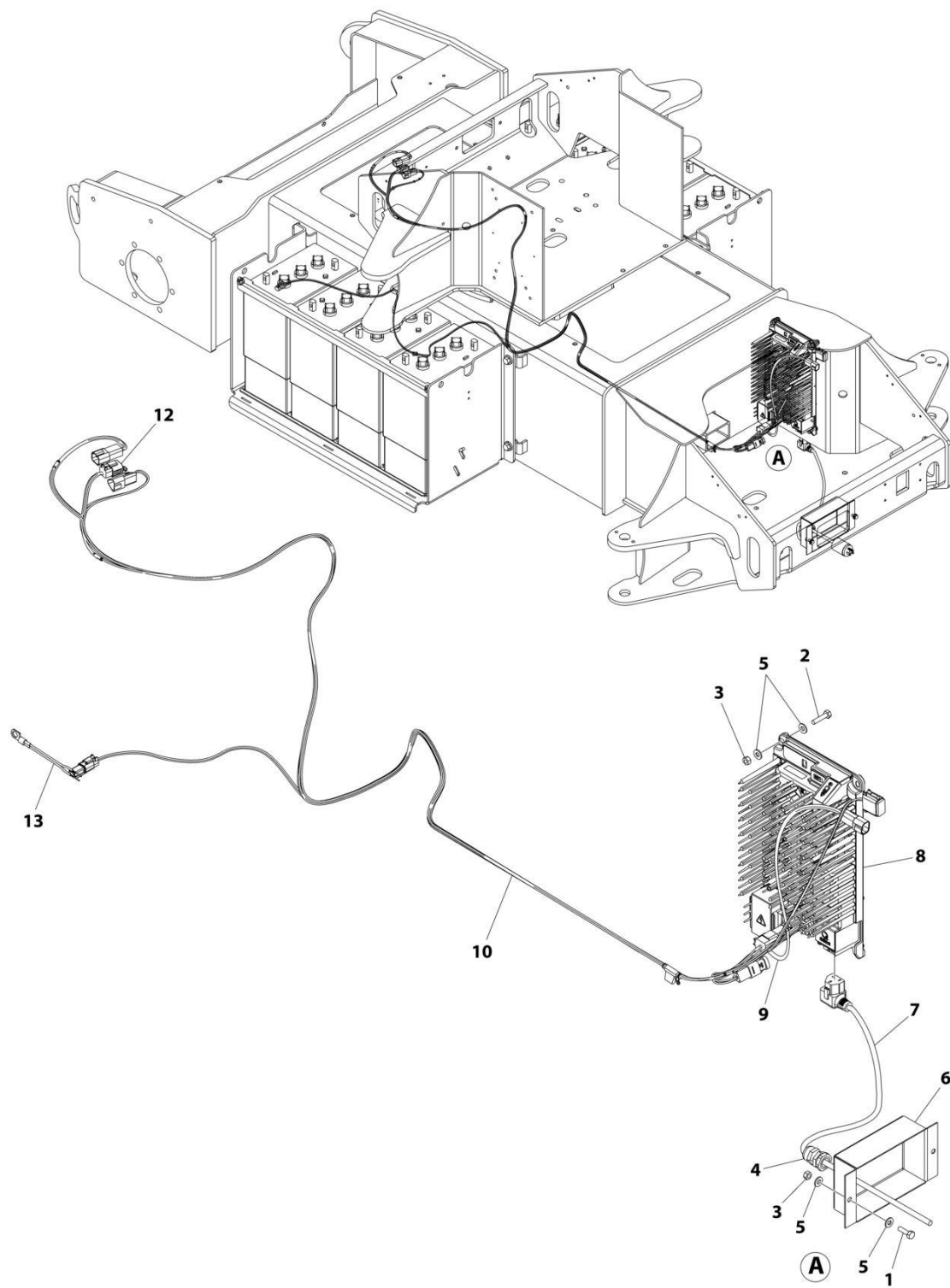
FIGURE 1-27. BATTERY CHARGER INSTALLATION (ANSI EXPORT, CE, CHINA & UK CA SPECS) (SN 0300298643 to Present)
