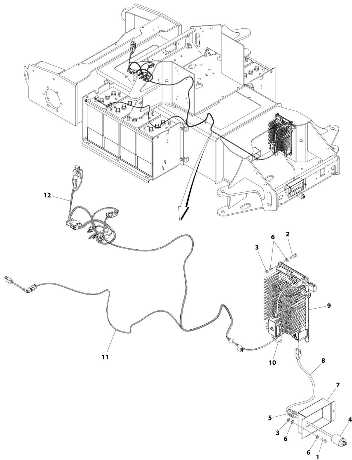
FIGURE 1-22. BATTERY CHARGER INSTALLATION (ALL SPECS EXCEPT AUSTRALIAN, CE & UK CA SPECS) (Prior to SN 0300298643)
