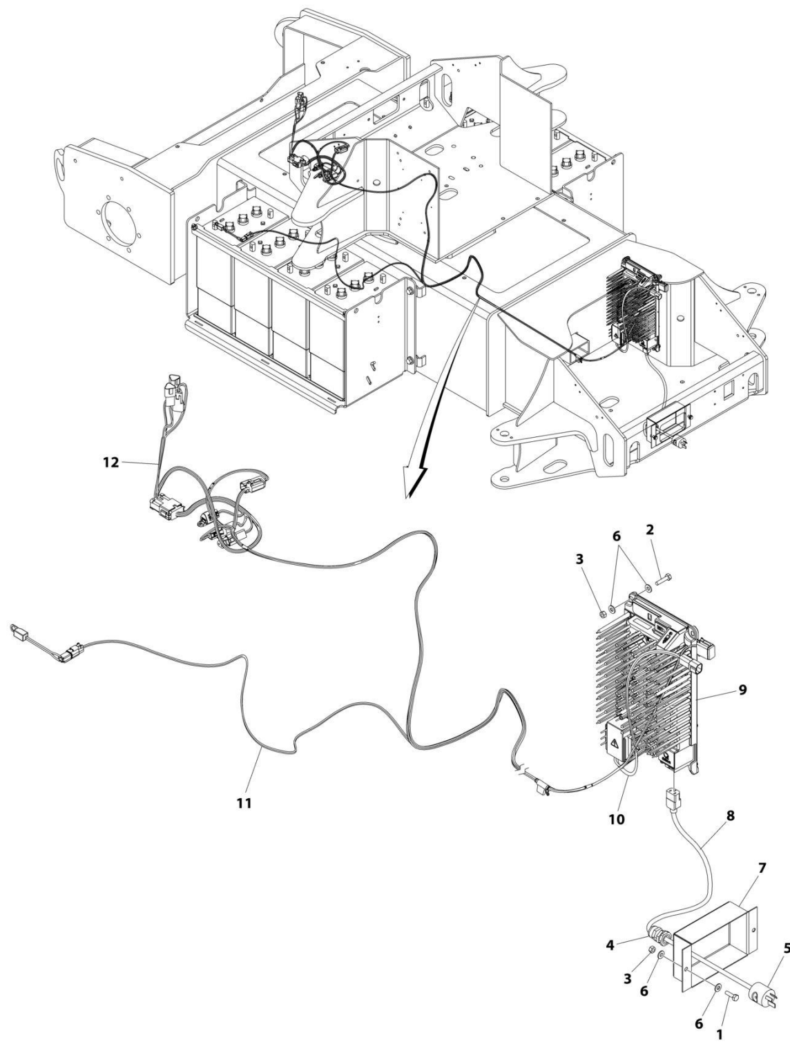
FIGURE 1-24. BATTERY CHARGER INSTALLATION - E400AJPNARROW (AUSTRALIAN SPEC) (Prior to SN 0300298643)
