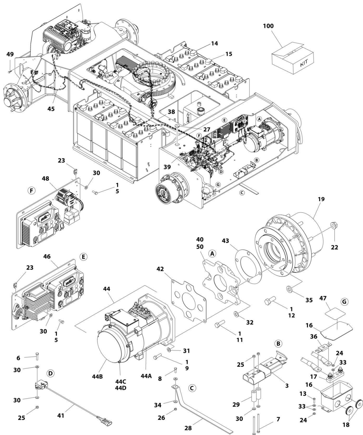
FIGURE 1-5. DRIVE INSTALLATION - UL SPECS
