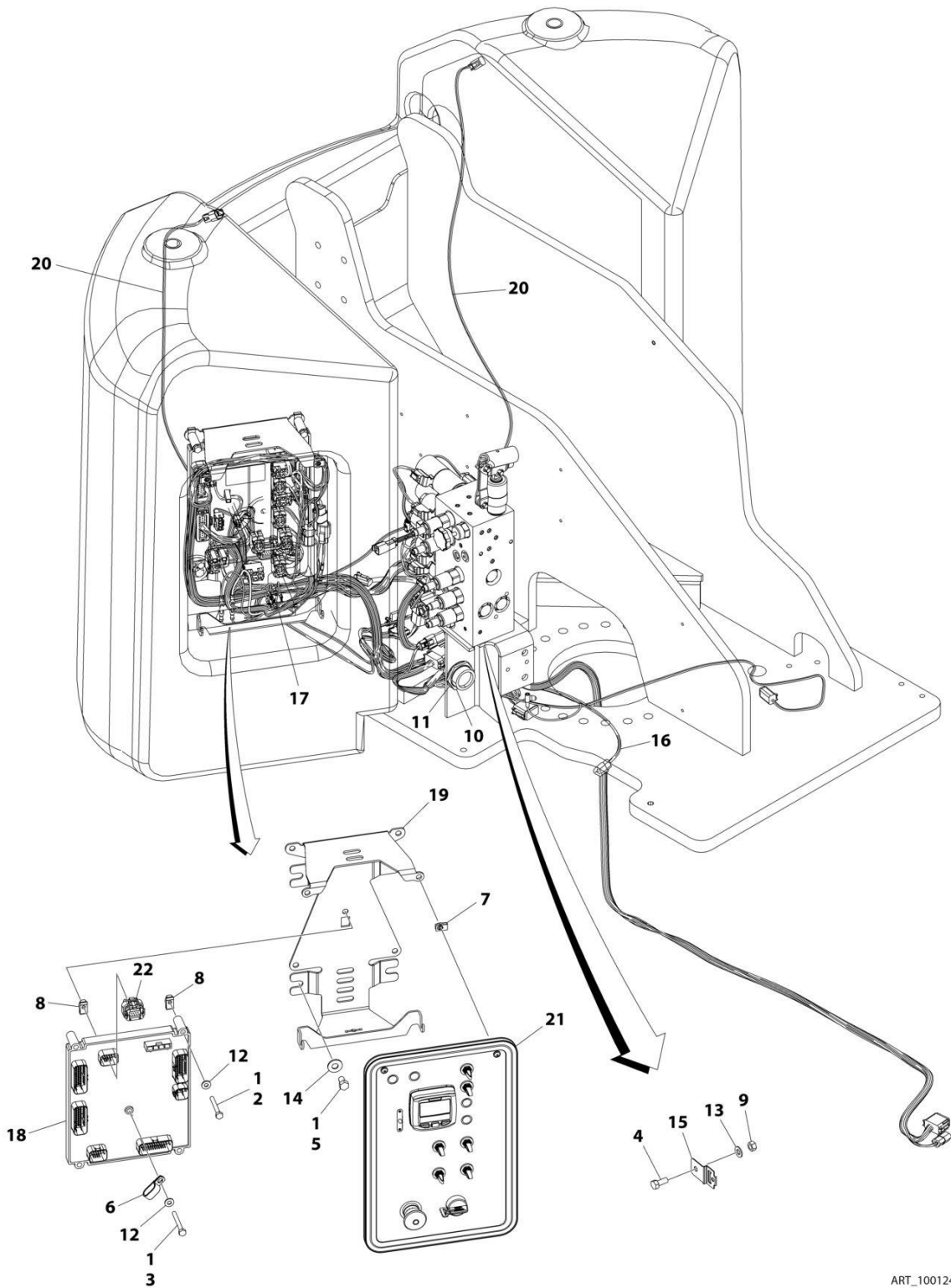
FIGURE 2-12. GROUND CONTROL BOX INSTALLATION - E400ANARROW (ALL SPECS EXCEPT AUSTRALIAN, CE & UK CA SPECS) (Prior to SN 0300298643)
