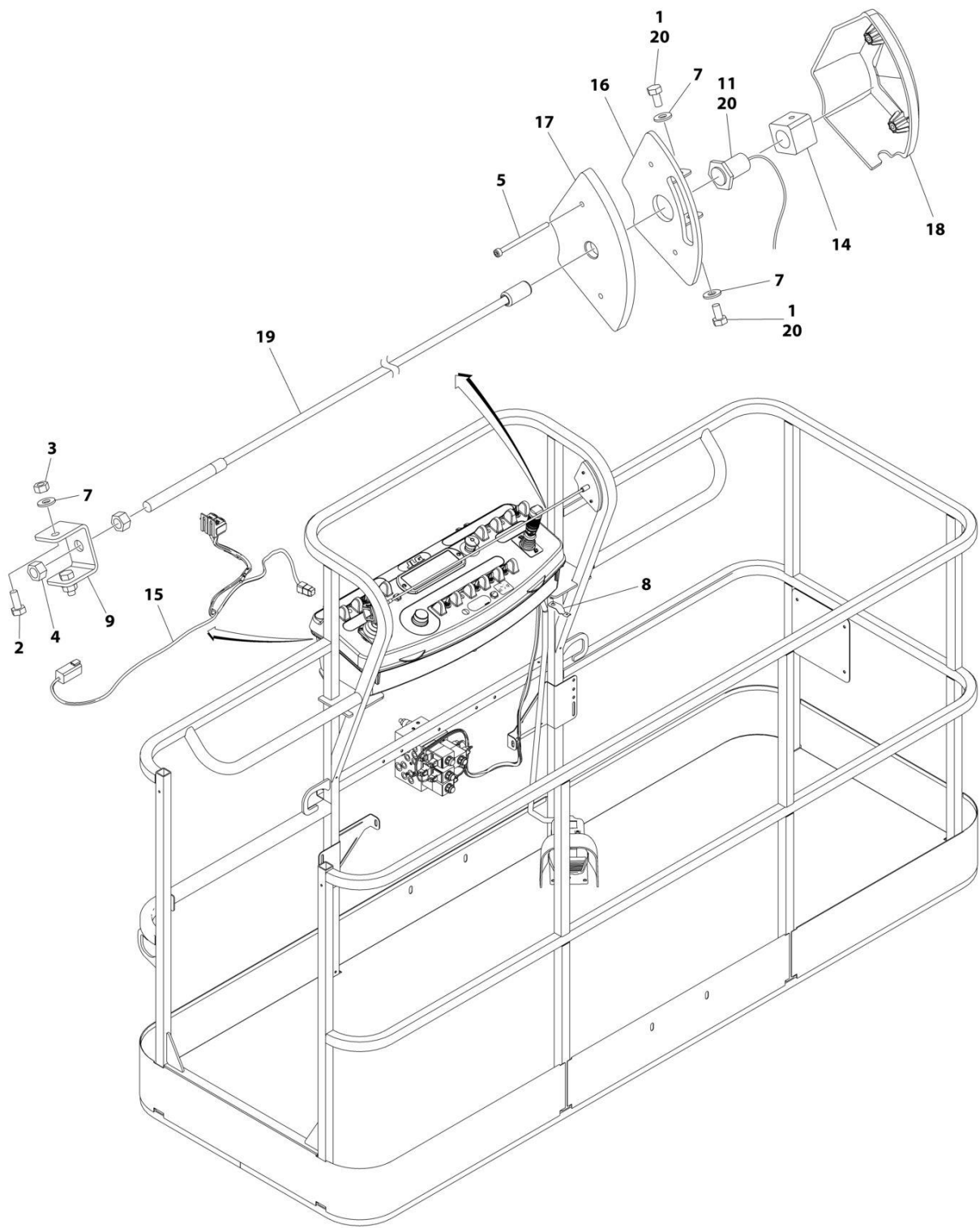
FIGURE 4-22. SKYLINE INSTALLATION
