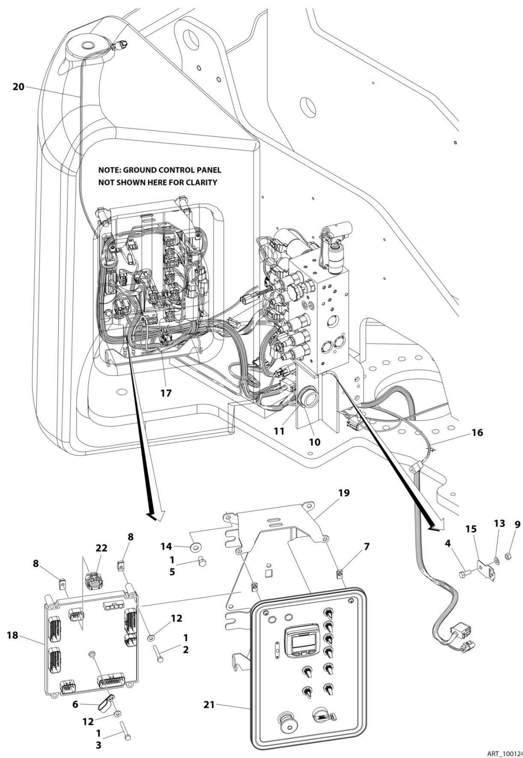
FIGURE 2-16. GROUND CONTROL BOX INSTALLATION - E400AJPNARROW (ALL SPECS EXCEPT CE & UK CA SPEC) (Prior to SN 0300298643)
