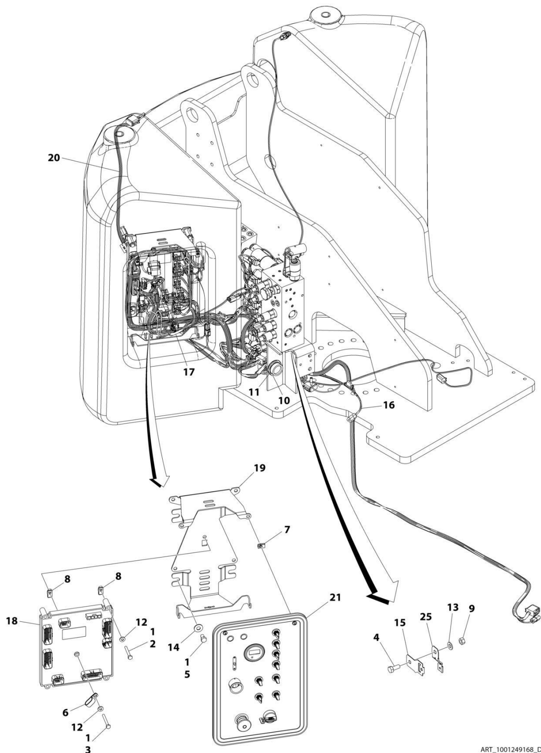
FIGURE 2-19. GROUND CONTROL BOX INSTALLATION - E400AJPNARROW (CE & UK CA SPEC) (SN 0300298643 to Present)
