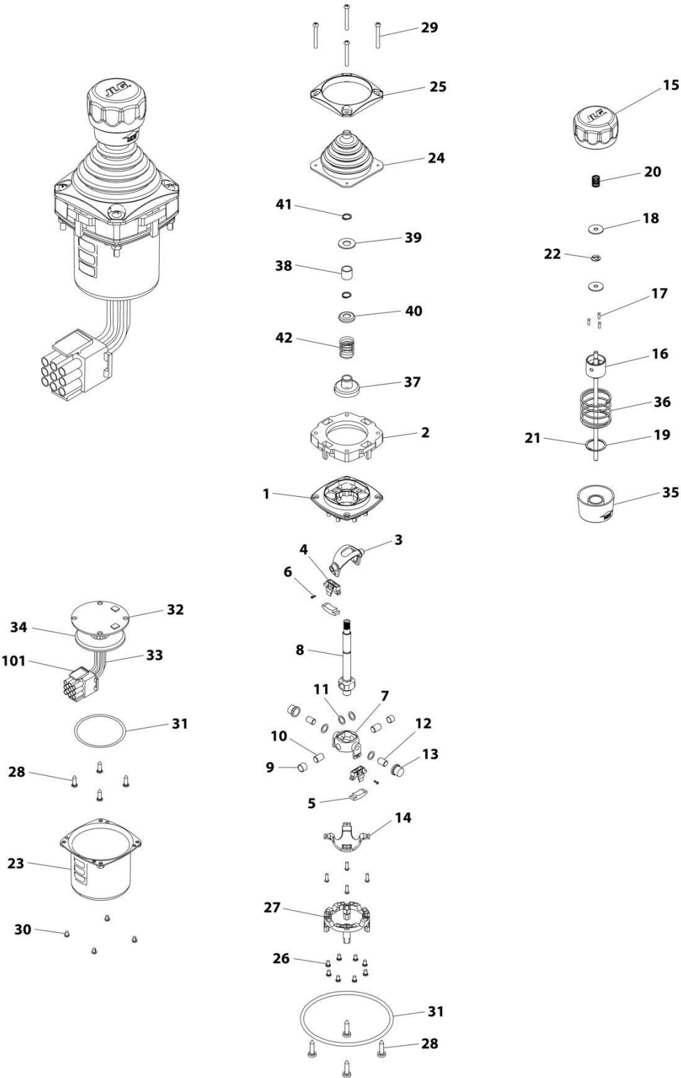
FIGURE 4-17. CONTROLLER ASSEMBLY - LIFT AND SWING
