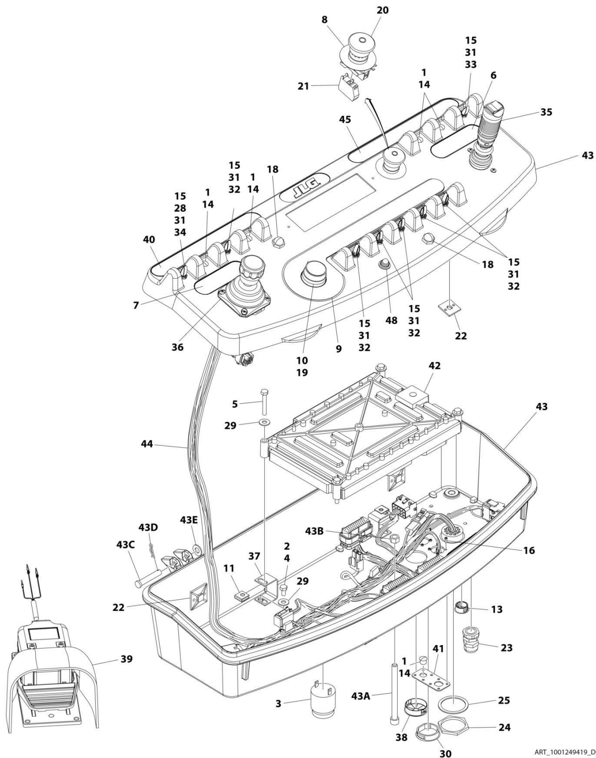
FIGURE 4-13. PLATFORM CONSOLE ASSEMBLY - E400ANARROW/E400AJPNARROW - UL LISTED (ALL SPECS EXCEPTED AUSTRALIAN, CE, JAPANESE & UK CA SPECS)
