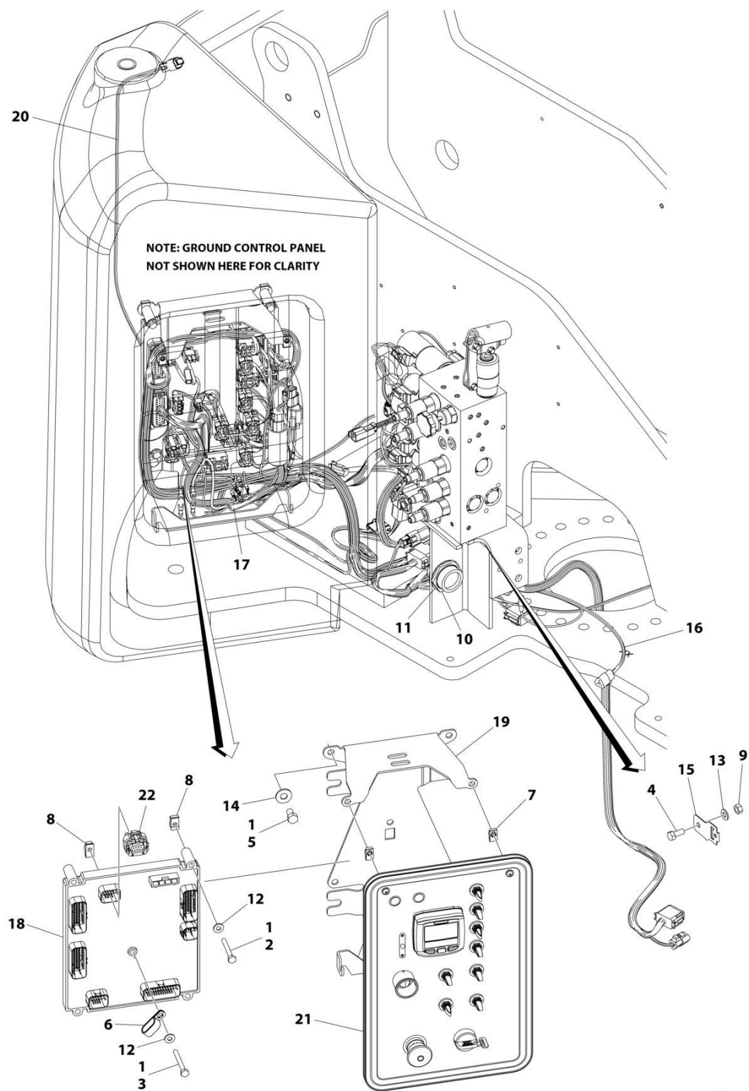
FIGURE 2-18. GROUND CONTROL BOX INSTALLATION - E400AJPNARROW (CE & UK CA SPEC) (Prior to SN 0300298643)
