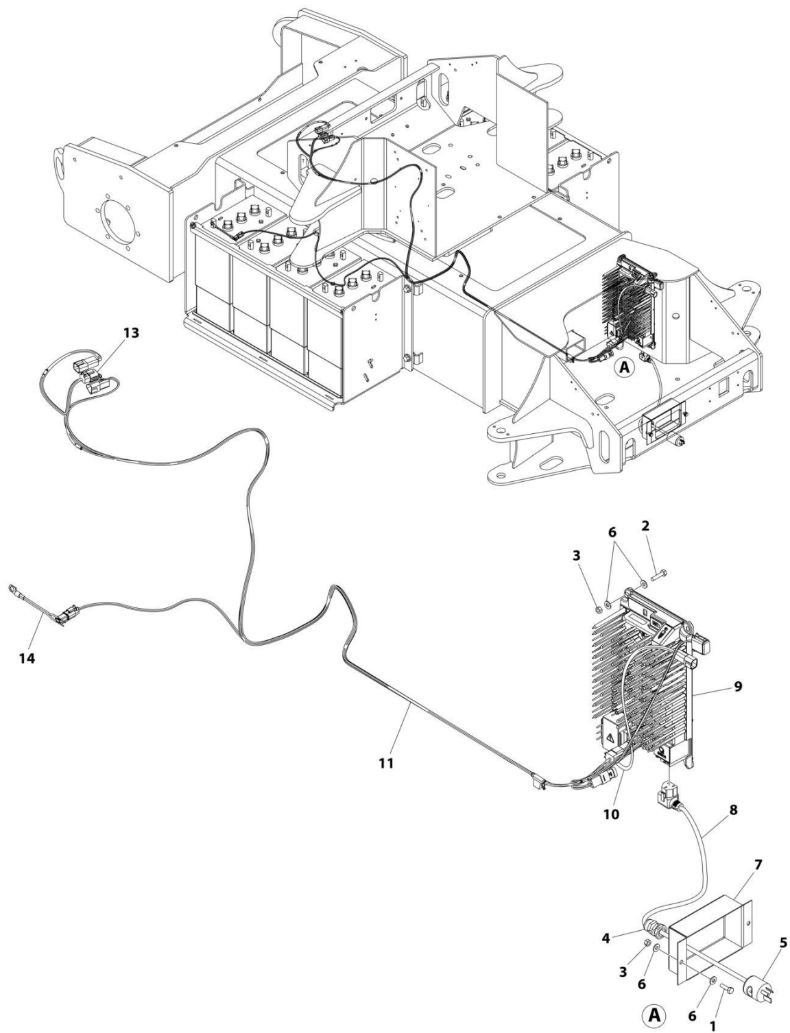
FIGURE 1-25. BATTERY CHARGER INSTALLATION (ANSI EXPORT, CE, CHINA & UK CA SPECS) (SN 0300298643 to Present)
