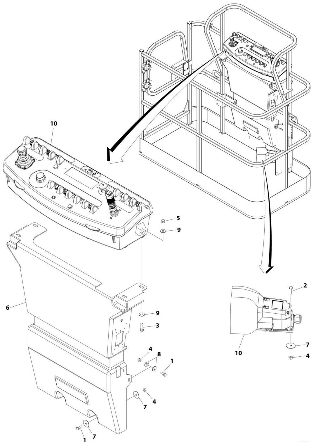
FIGURE 4-9. PLATFORM CONSOLE AND FOOTSWITCH INSTALLATION - E400AJPNARROW - NON-UL LISTED (ALL SPECS EXCEPT UL SPECS)
