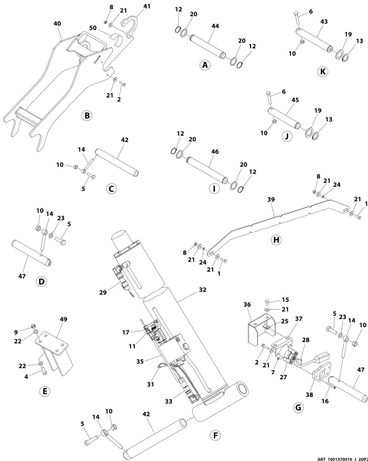
FIGURE 3-2. SCISSORS ARMS INSTALLATION (KOREAN, CHINESE, AUSTRALIAN, CE & UK CA SPECS) (Prior to SN B200081951, Prior to SN M200071248)
