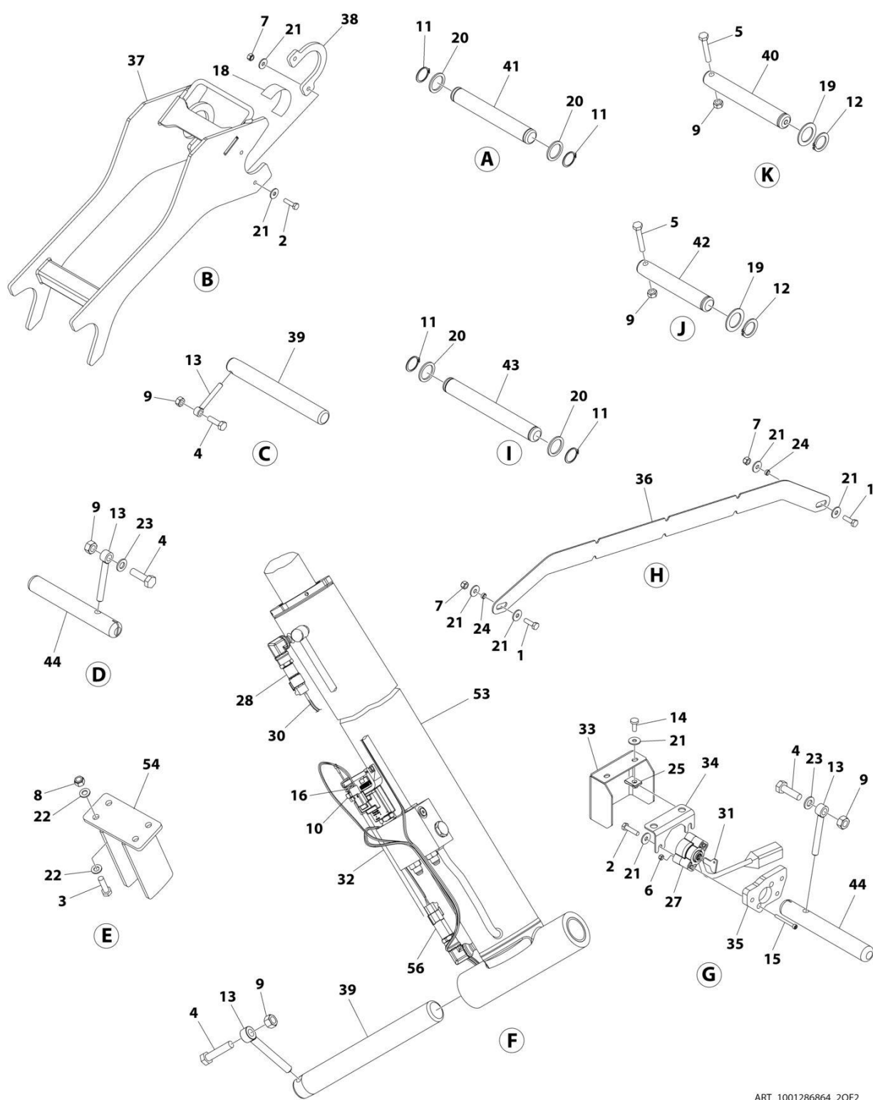
FIGURE 3-4. SCISSORS ARMS INSTALLATION (ANSI, ANSI EXPORT, CSA & JAPANESE SPECS) (Prior to SN B200081951, Prior to SN M200071248)
