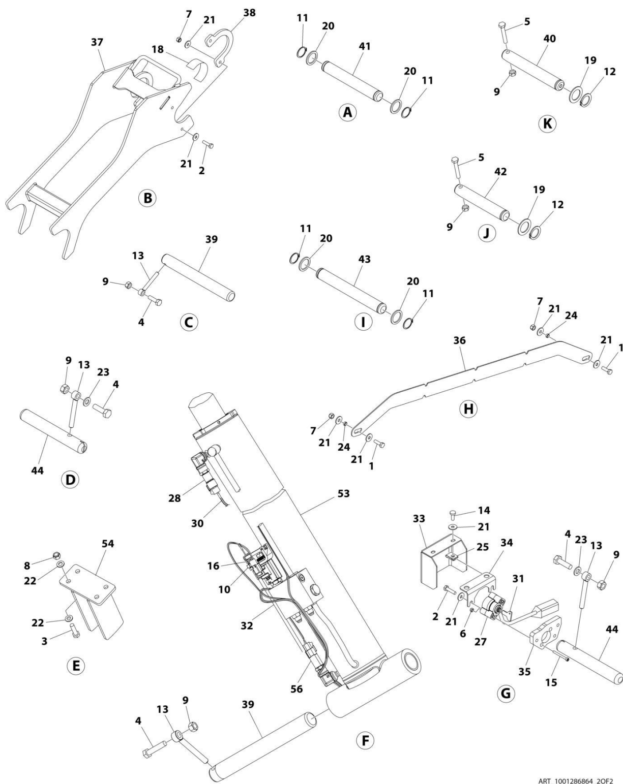
FIGURE 3-6. SCISSORS ARMS INSTALLATION (ALL SPECS)
