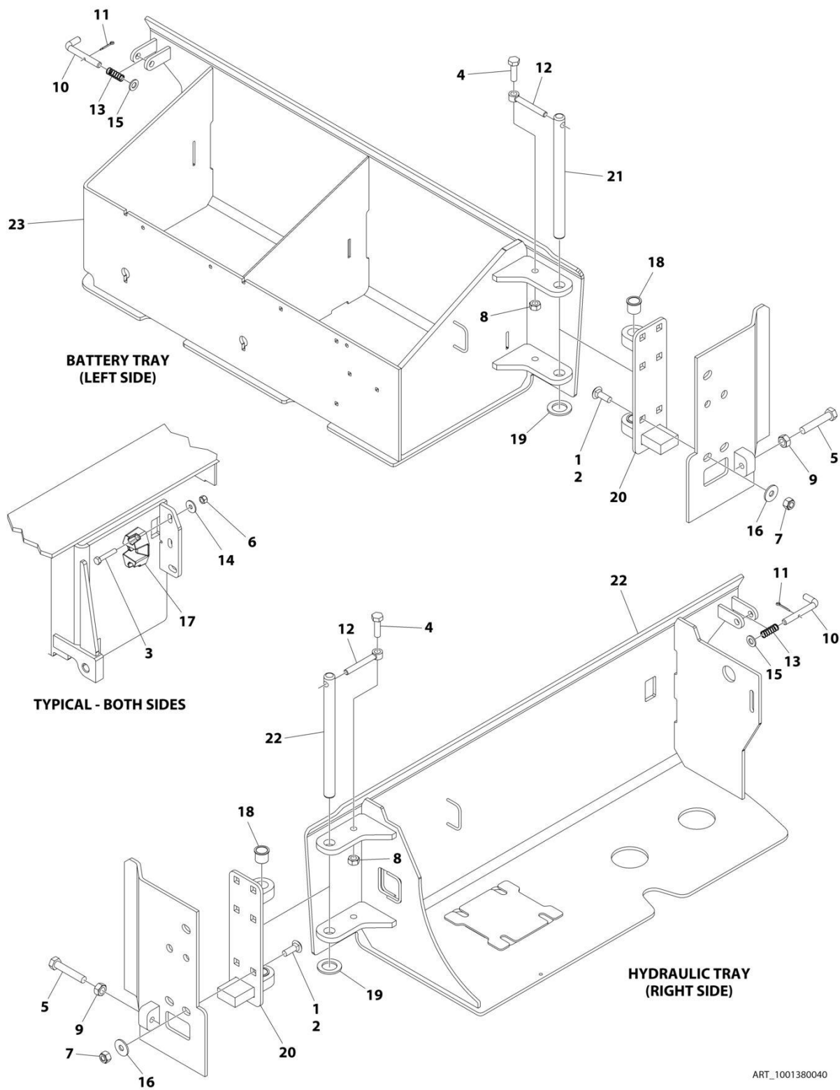
FIGURE 2-15. DOORS INSTALLATION
