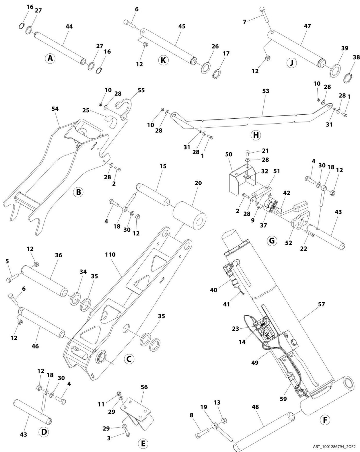
FIGURE 3-6. SCISSORS ARMS INSTALLATION (MACHINES WITH SN STARTING WITH B2) (ALL SPECS EXCEPT CHINA SPECS) (SN B200081909 to Present)
