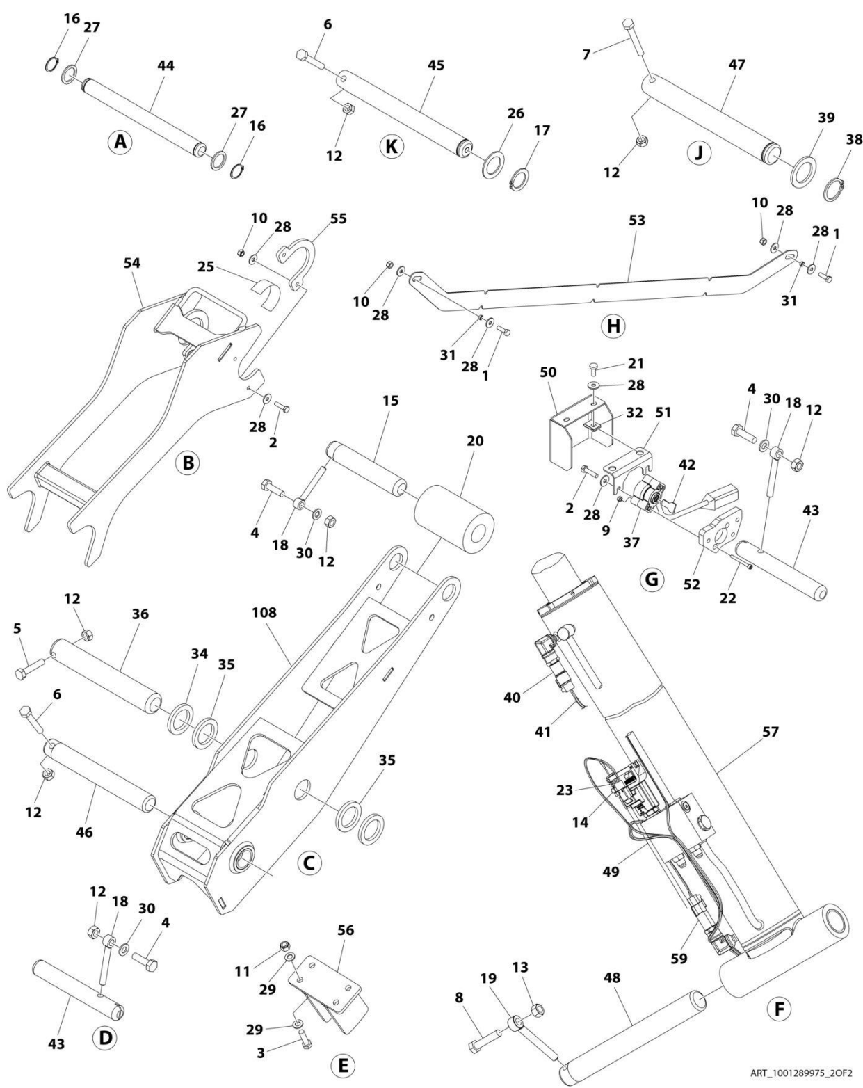
FIGURE 3-8. SCISSORS ARMS INSTALLATION (MACHINES WITH SN STARTING WITH M2)
