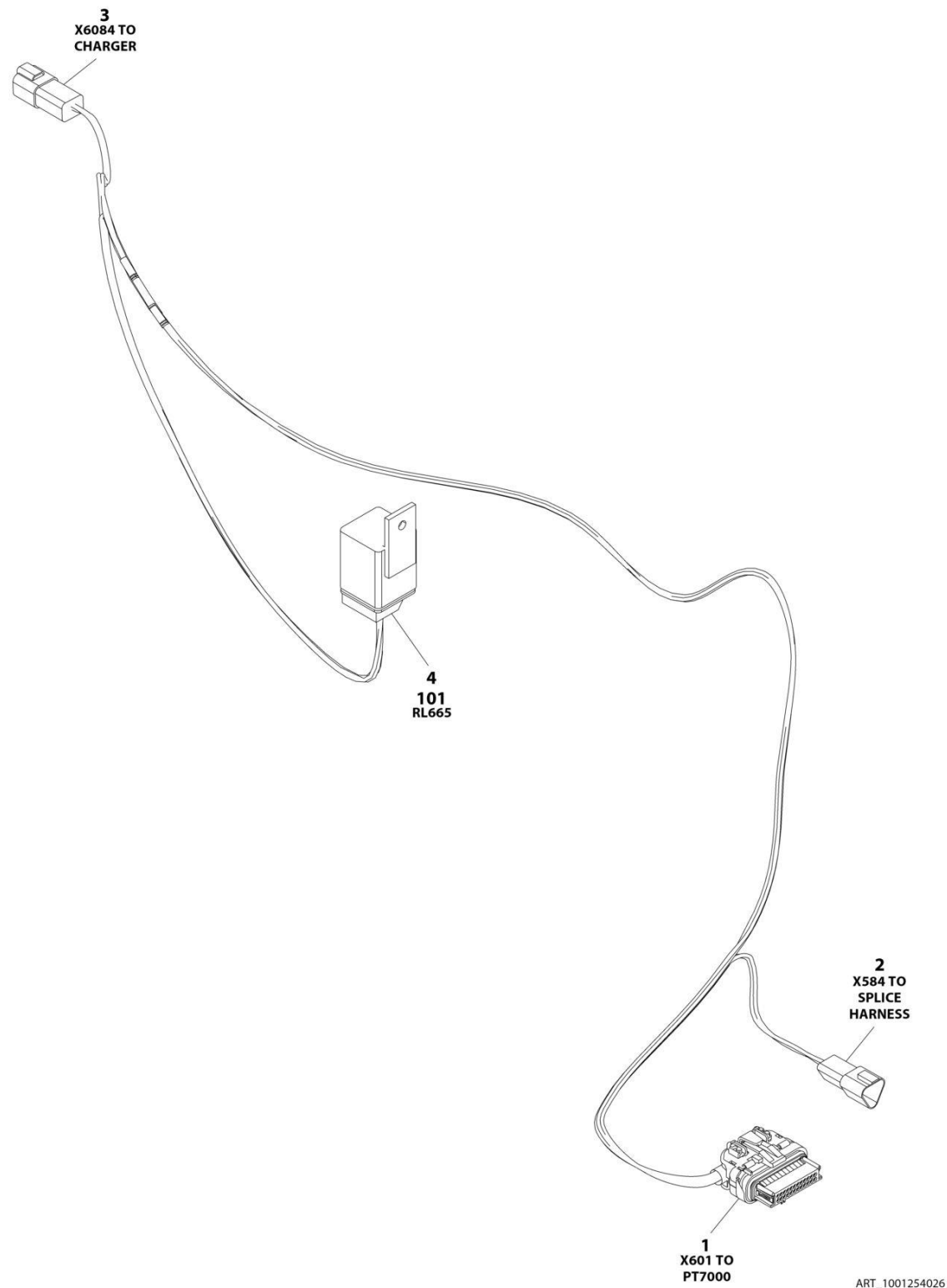
FIGURE 6-30. CLEARSKY HARNESS - 3G & 4G (ALL SPECS EXCEPT CHINA SPECS)
