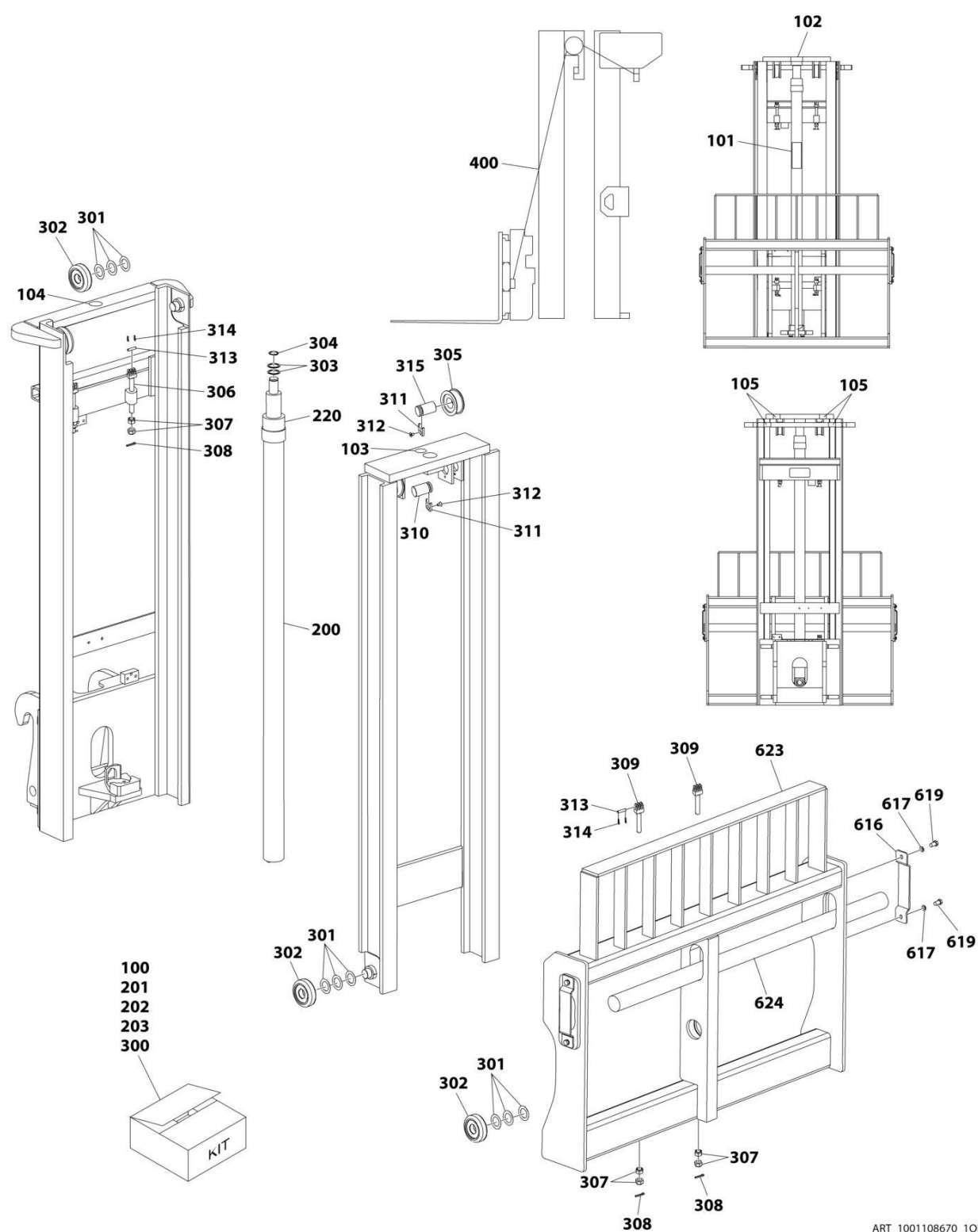
FIGURE 3-25. MAST ASSEMBLY - 8FT (4500LBS) (WITH SIDE TILT) (SN 0160037900 to Present, Including 0160037855)
