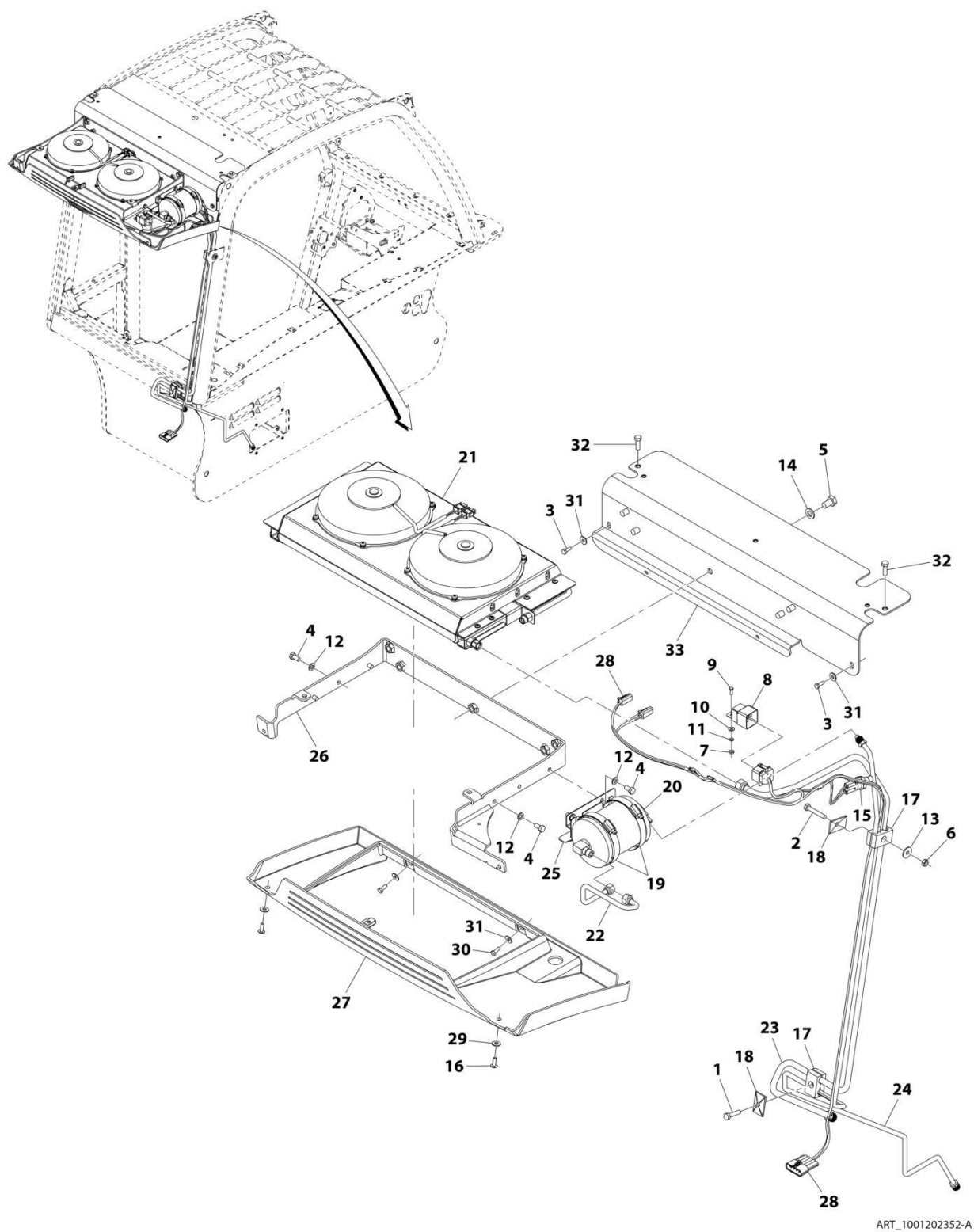
FIGURE 6-40. A/C CONDENSER INSTALLATION
