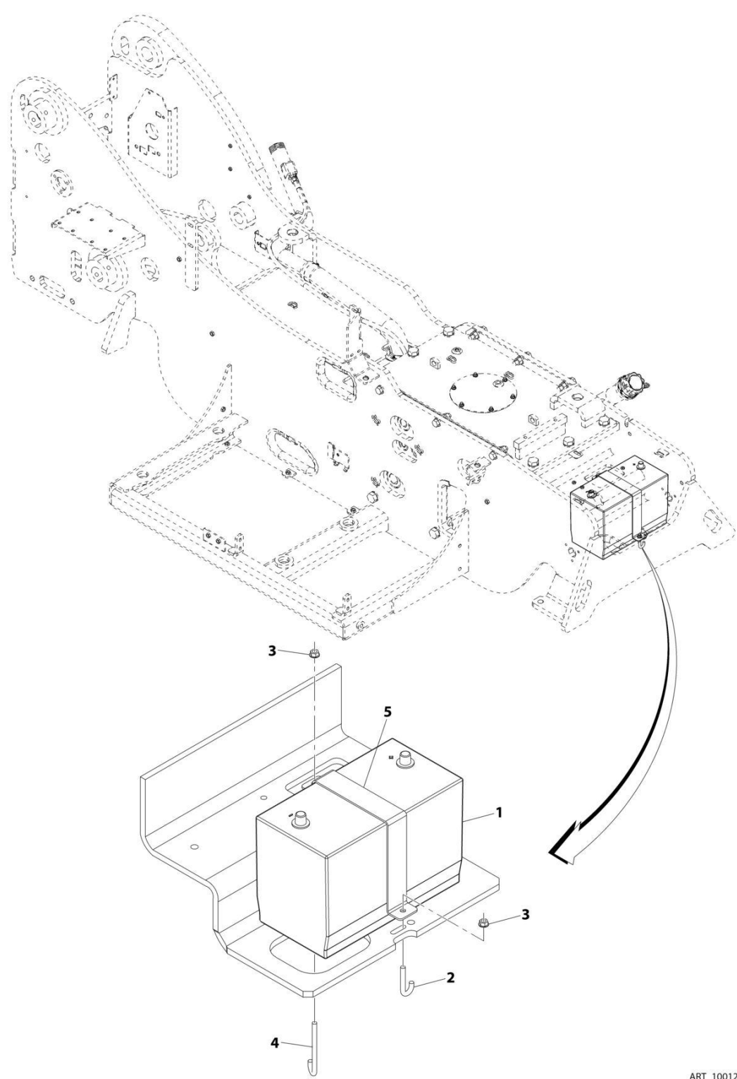
FIGURE 10-5. BATTERY INSTALLATION
