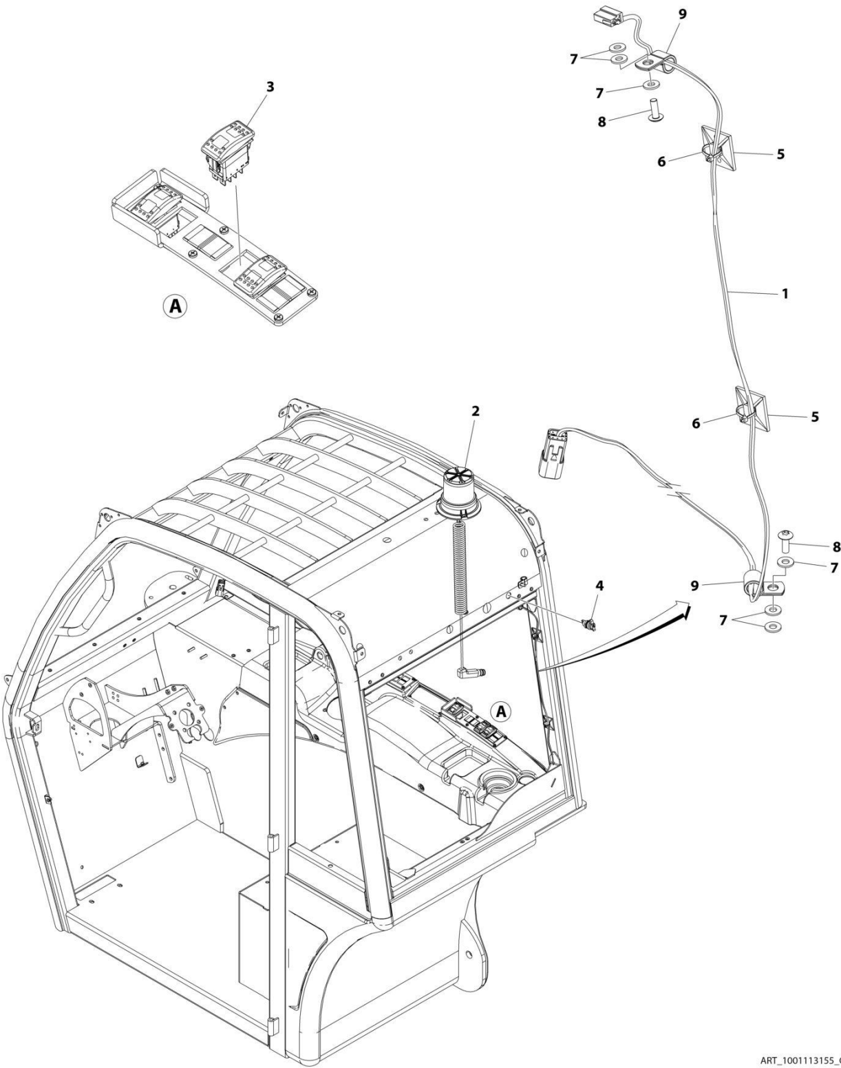
FIGURE 10-35. LIGHTS - BEACON LIGHT INSTALLATION (OPEN CAB)
