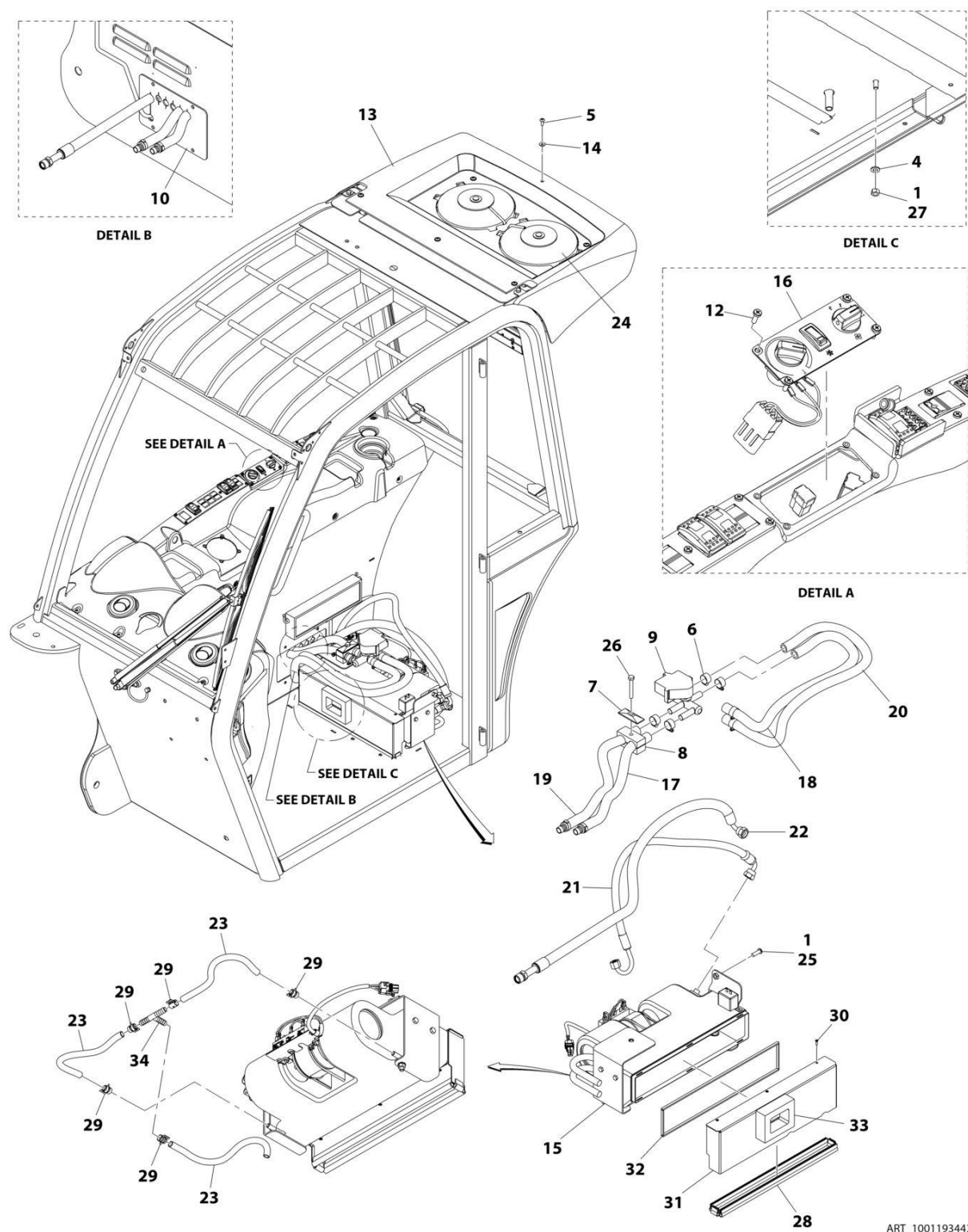
FIGURE 6-34. HEATER AND A/C INSTALLATION (CAB PARTS)
