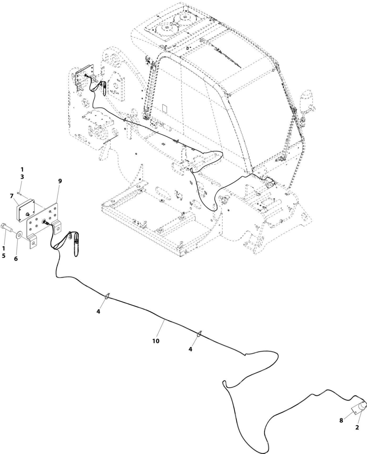
FIGURE 10-55. REVERSE SENSING SYSTEM INSTALLATION
