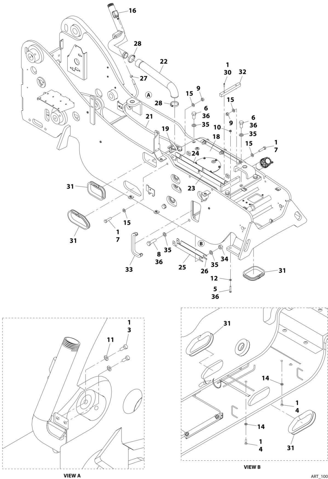
FIGURE 1-4. TANK INSTALLATION
