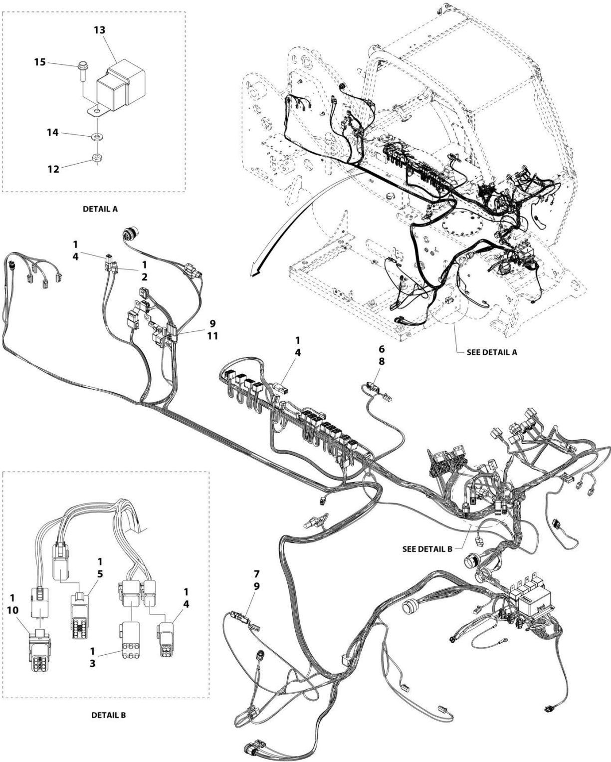
FIGURE 10-20. ELECTRICAL HARNESS CAPS INSTALLATION
