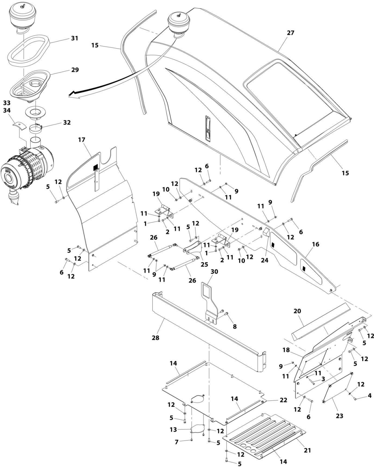
FIGURE 1-1. HOODS INSTALLATION
