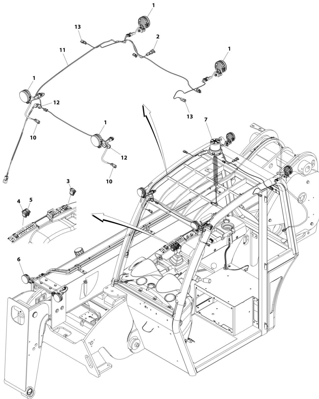
FIGURE 10-45. LIGHTS - WORKLIGHTS INSTALLATION (CAB, BOOM AND BEACON) (CLOSED CAB)
