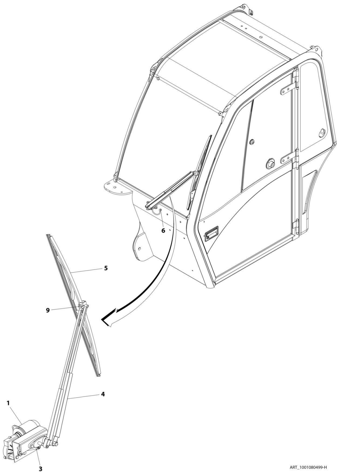
FIGURE 6-24. FRONT WIPER ASSEMBLY
