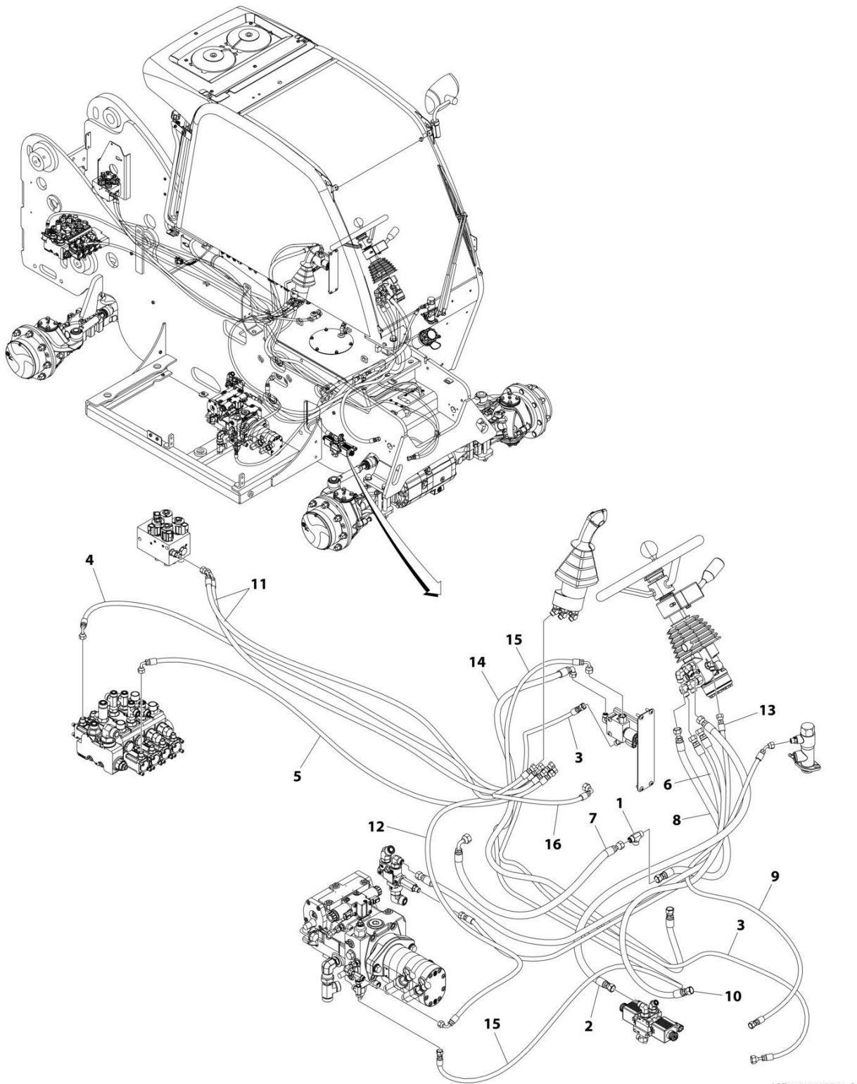
FIGURE 8-6. HOSE INSTALLATION - CAB (ANSI)
