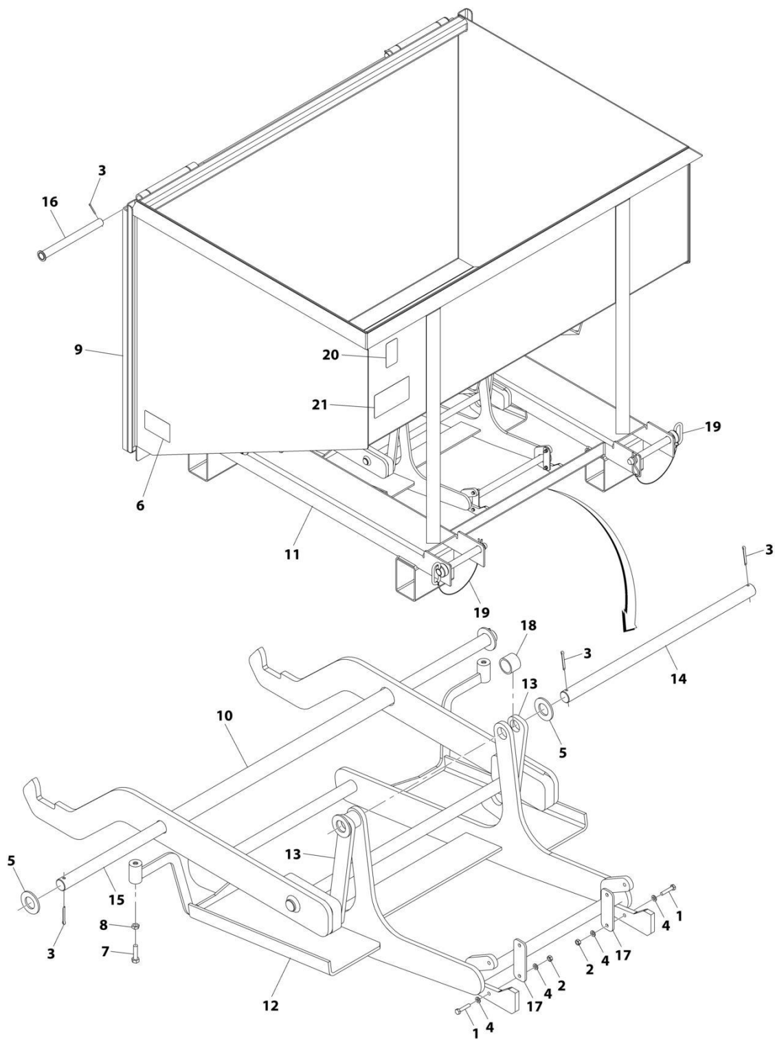
FIGURE 3-56. HOPPER - TRASH
