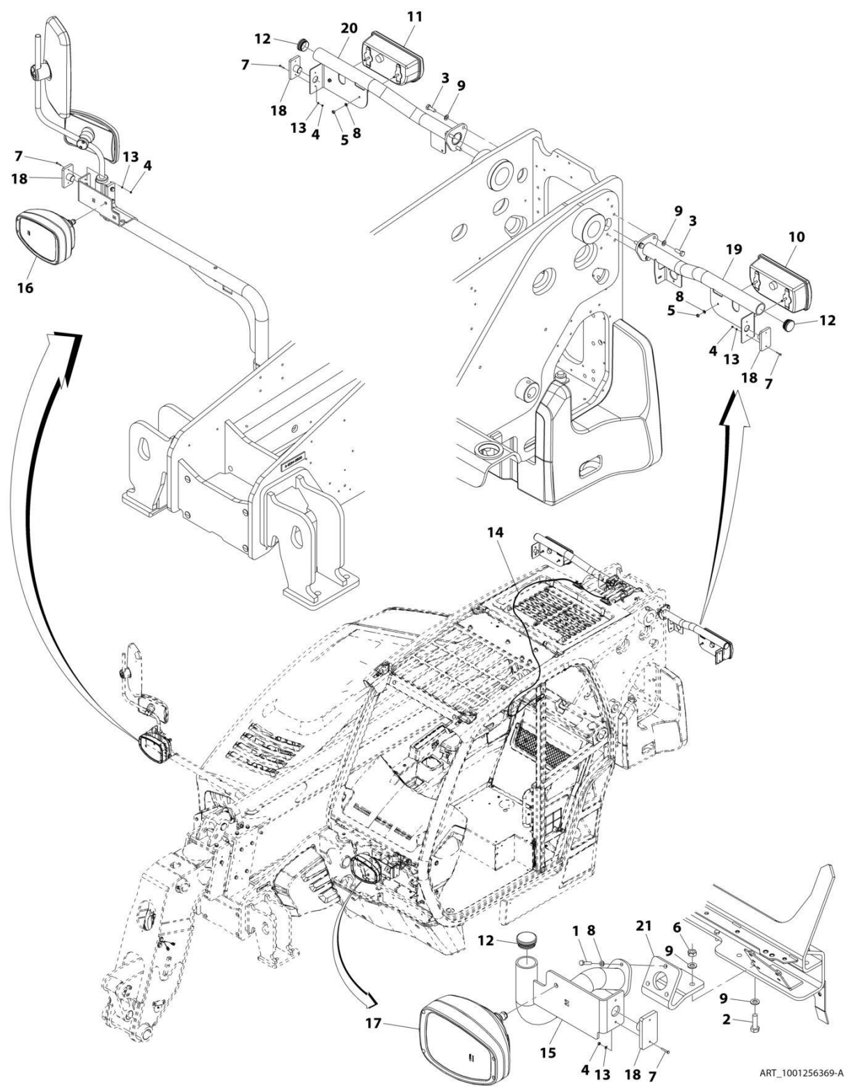
FIGURE 10-41. LIGHTS - DIP LIGHTS INSTALLATION (RH)
