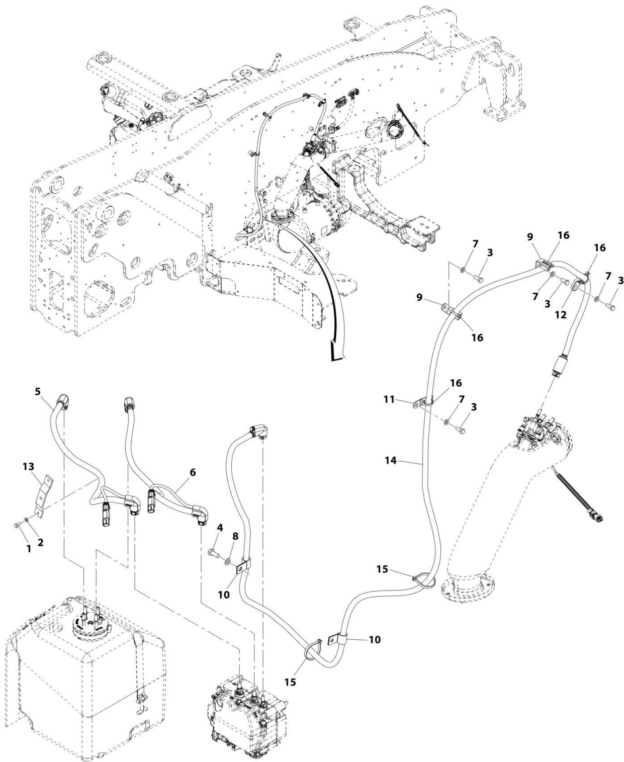
FIGURE 4-10. DEF LINES INSTALLATION (ULS)
