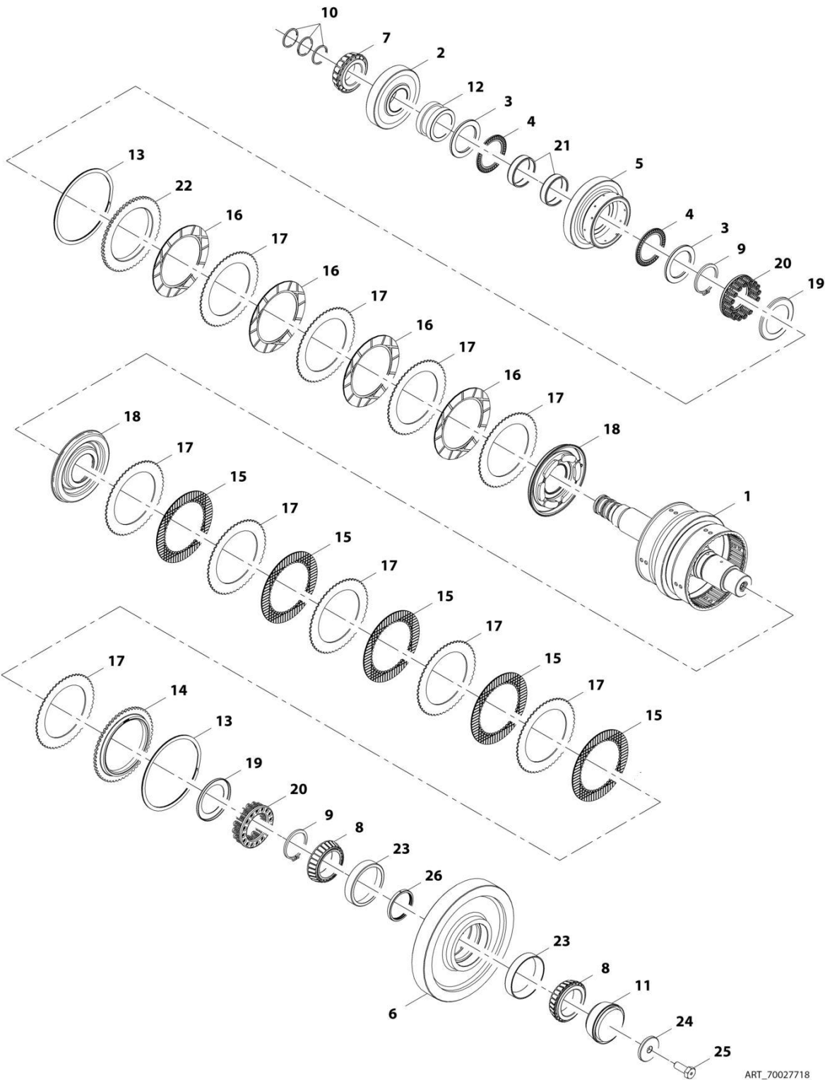
FIGURE 5-11. TRANSMISSION CLUTCH GROUP
