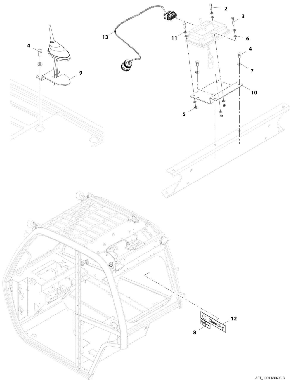
FIGURE 10-26. CLEARSKY INSTALLATION (NO A/C - SHORT ROOF CAP)
