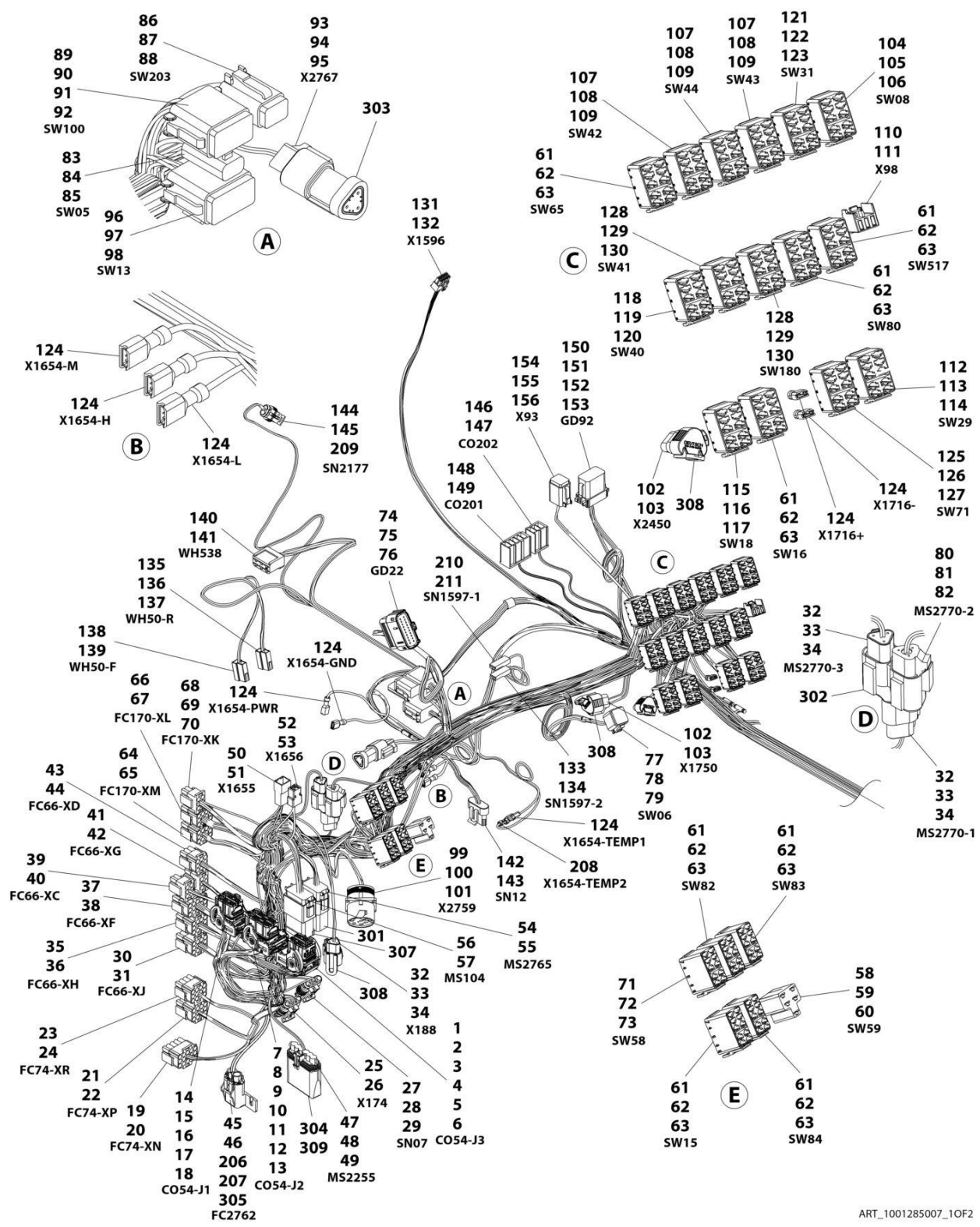
FIGURE 10-12. CAB HARNESS
