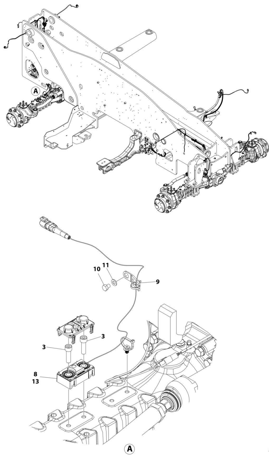
FIGURE 10-54. LSI SENSOR INSTALLATION
