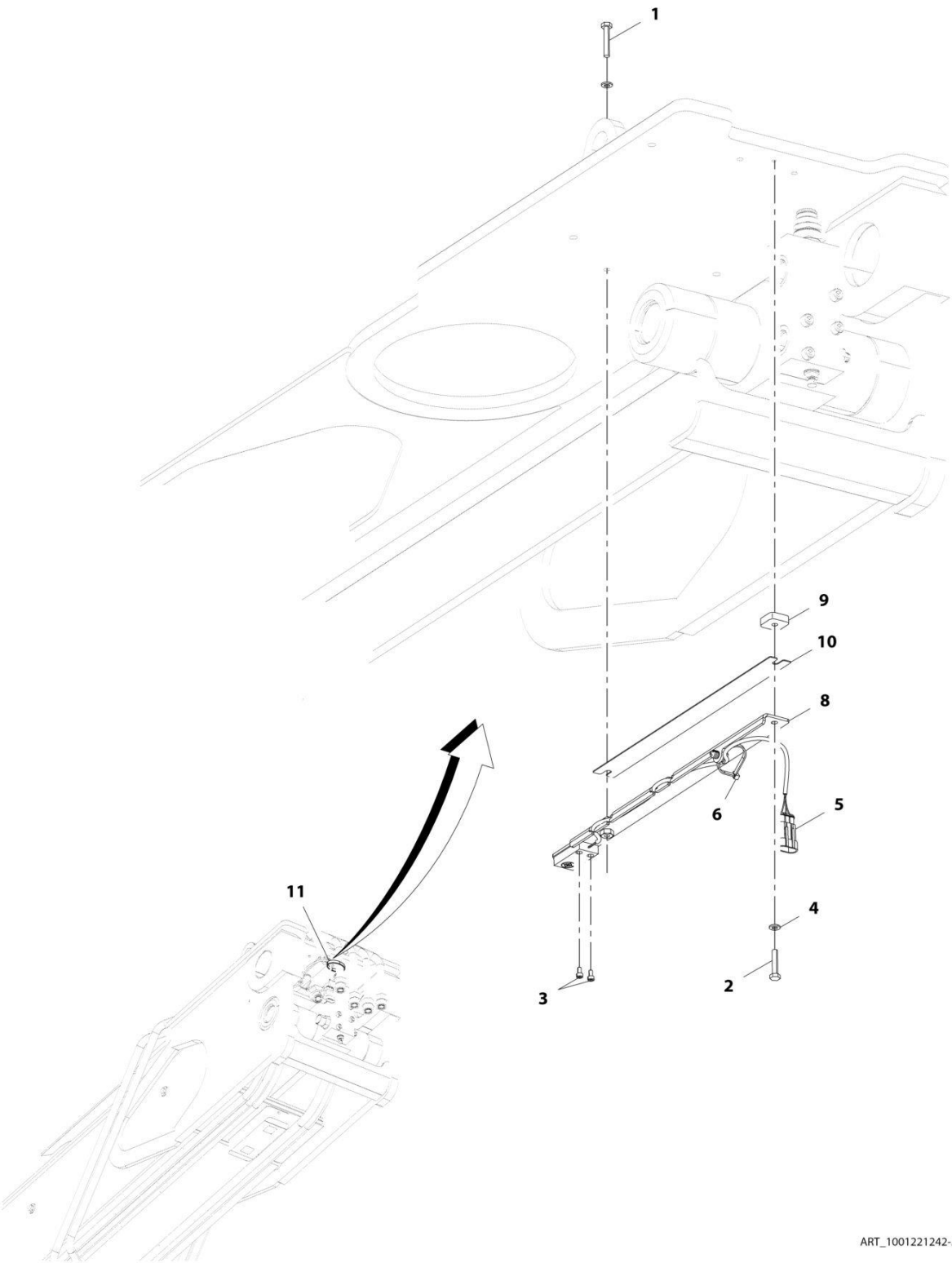
FIGURE 10-8. BOOM RETRACT SENSOR INSTALLATION
