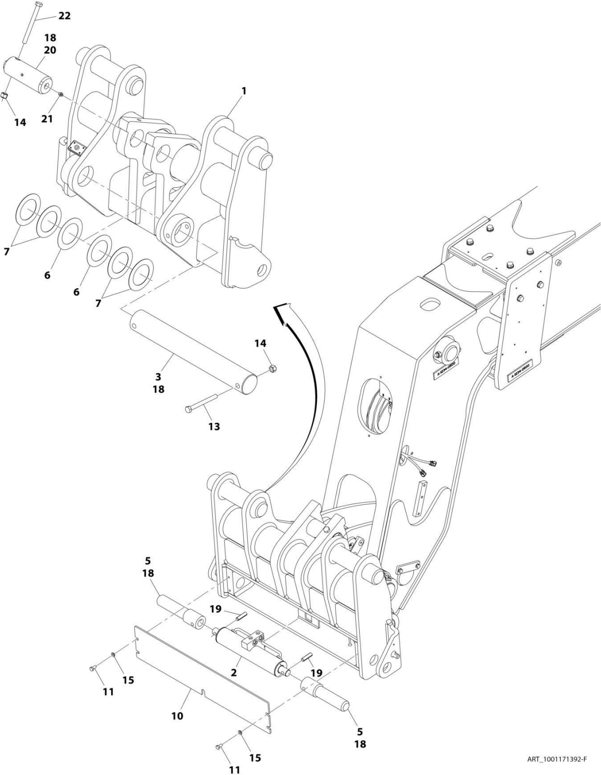
FIGURE 2-10. HYDRAULIC QUICK COUPLER INSTALLATION
