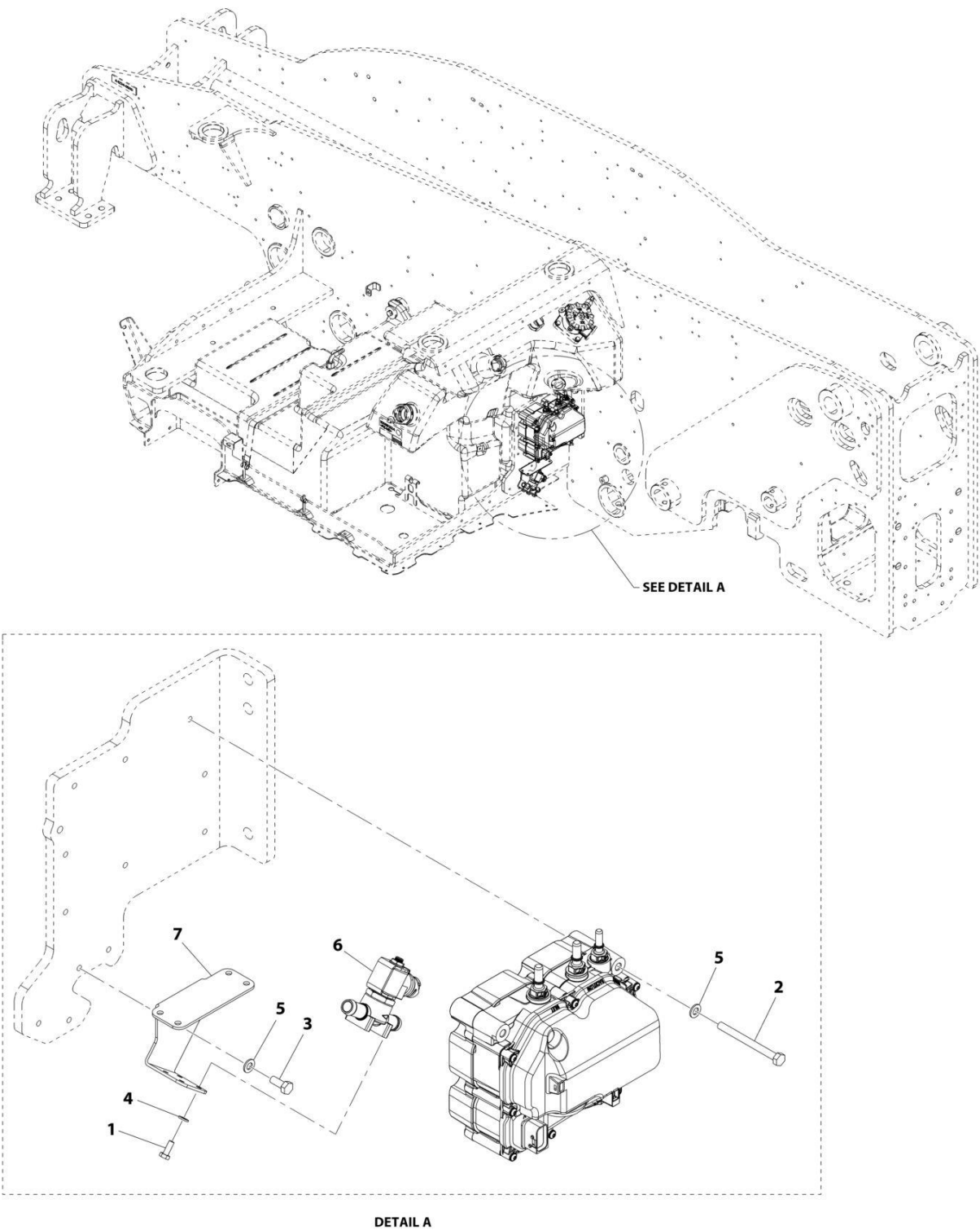
FIGURE 4-11. DEF CONTROL MODULE INSTALLATION (ULS)
