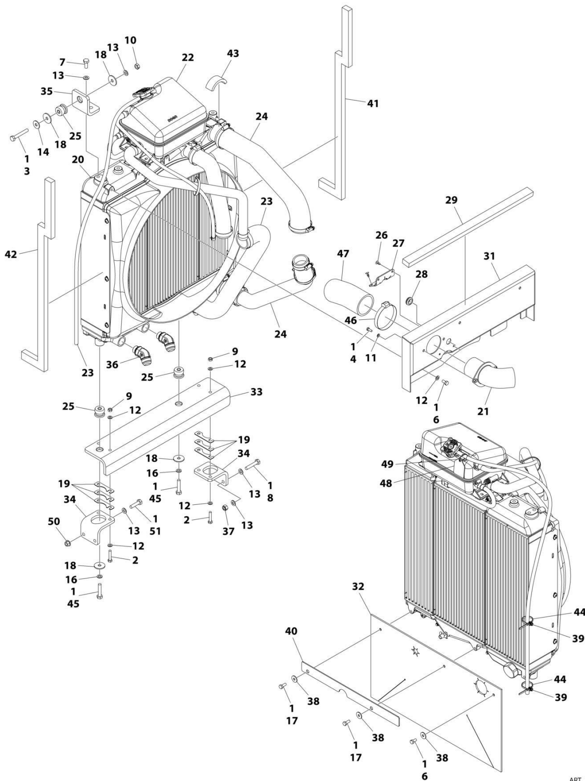
FIGURE 4-16. ENGINE COOLING SYSTEM INSTALLATION (PVC 2305)
