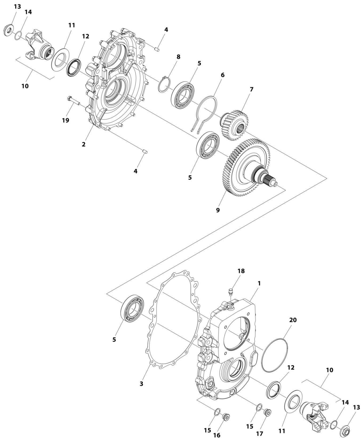
FIGURE 5-37. GEARBOX ASSEMBLY (PVC 2311)
