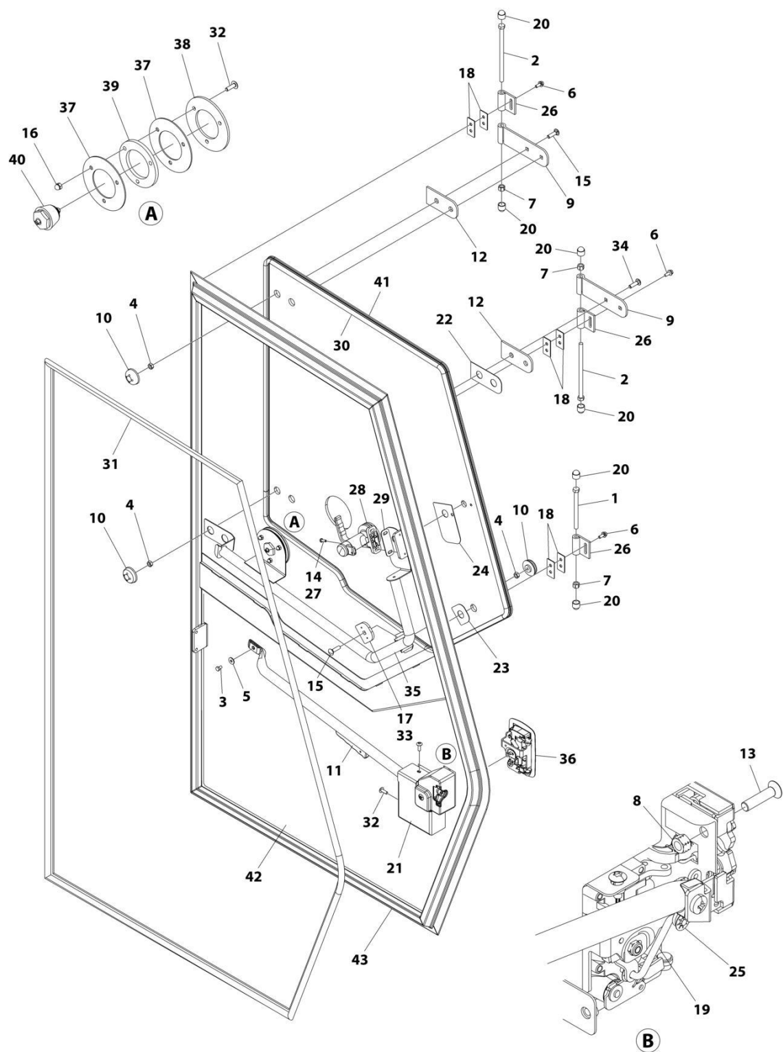
FIGURE 6-15. DOOR ASSEMBLY (SN 0160126061 to Present)
