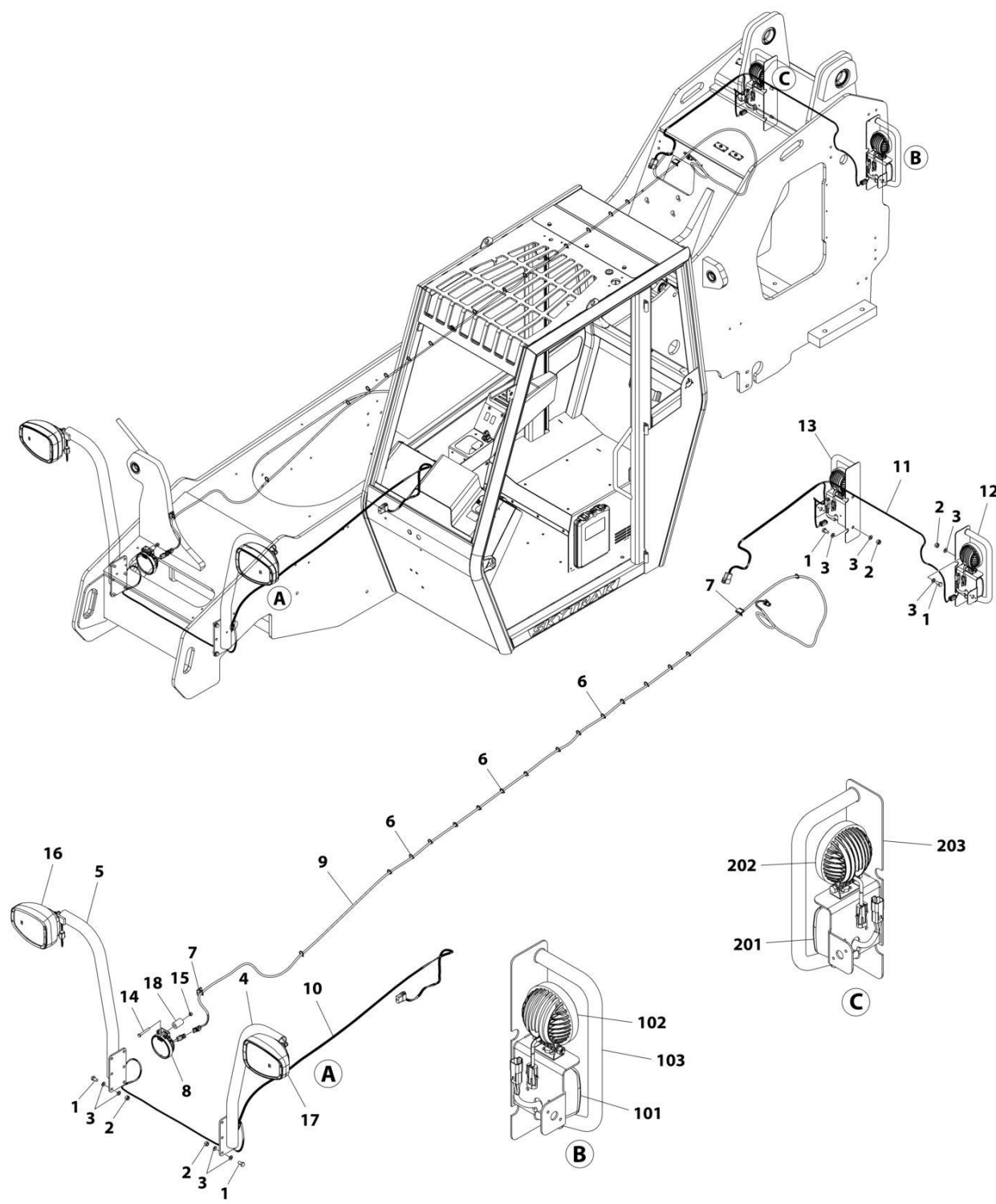
FIGURE 10-39. LIGHTS - ROADLIGHTS INSTALLATION (Prior to SN 0160129391)
