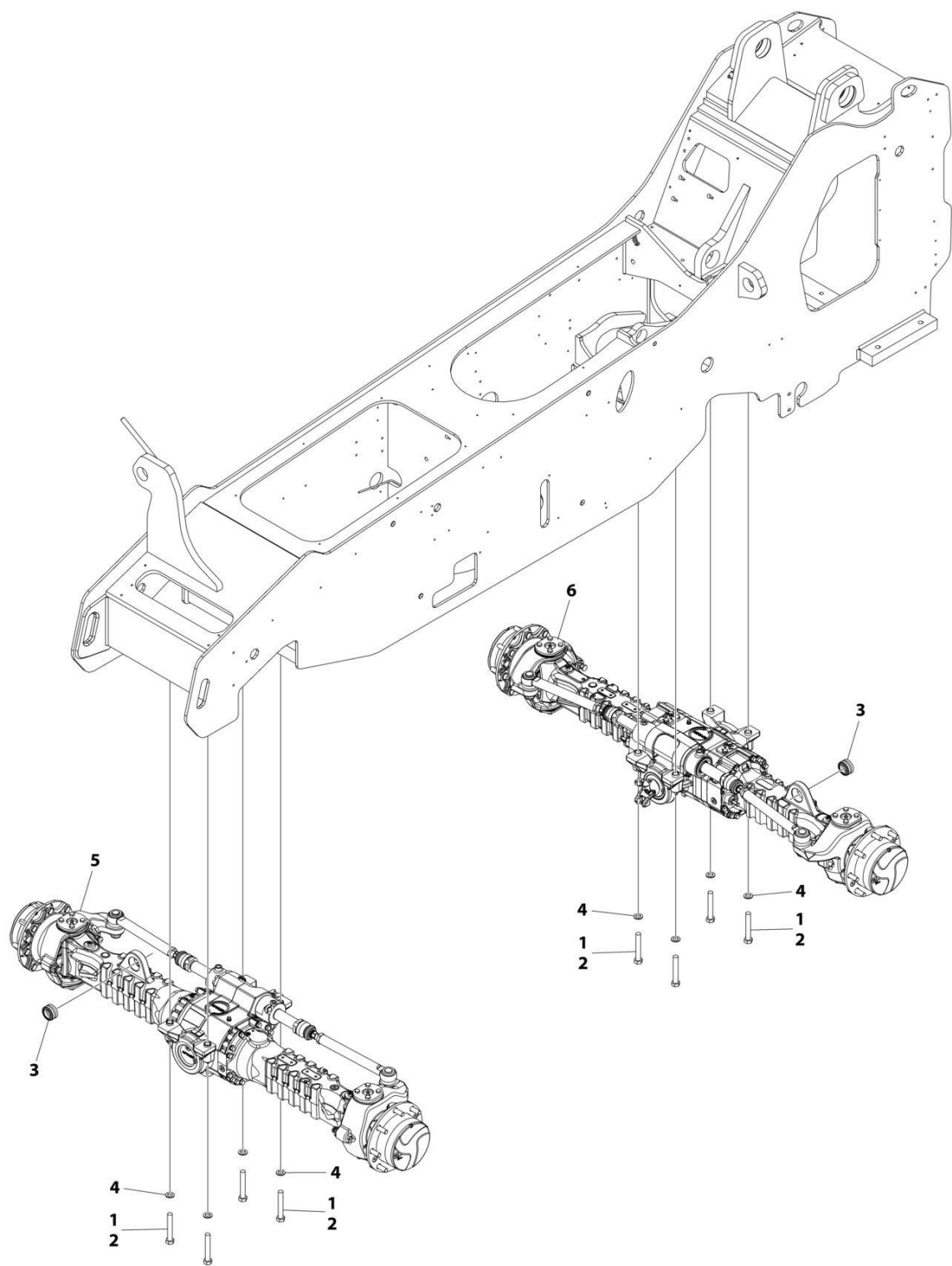
FIGURE 5-2. AXLES INSTALLATION (PVC 2311)
