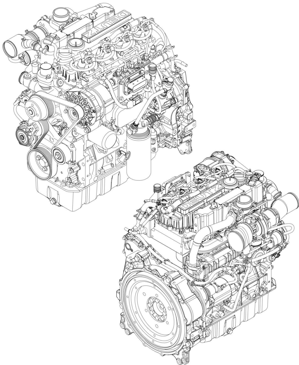
FIGURE 4-5. ENGINE ASSEMBLY - HRC (PVC 2305)
