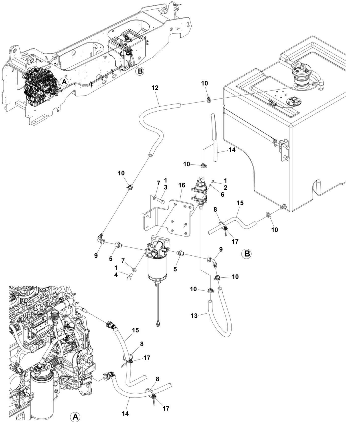
FIGURE 4-14. ENGINE FUEL SYSTEM INSTALLATION (LRC ENGINES)
