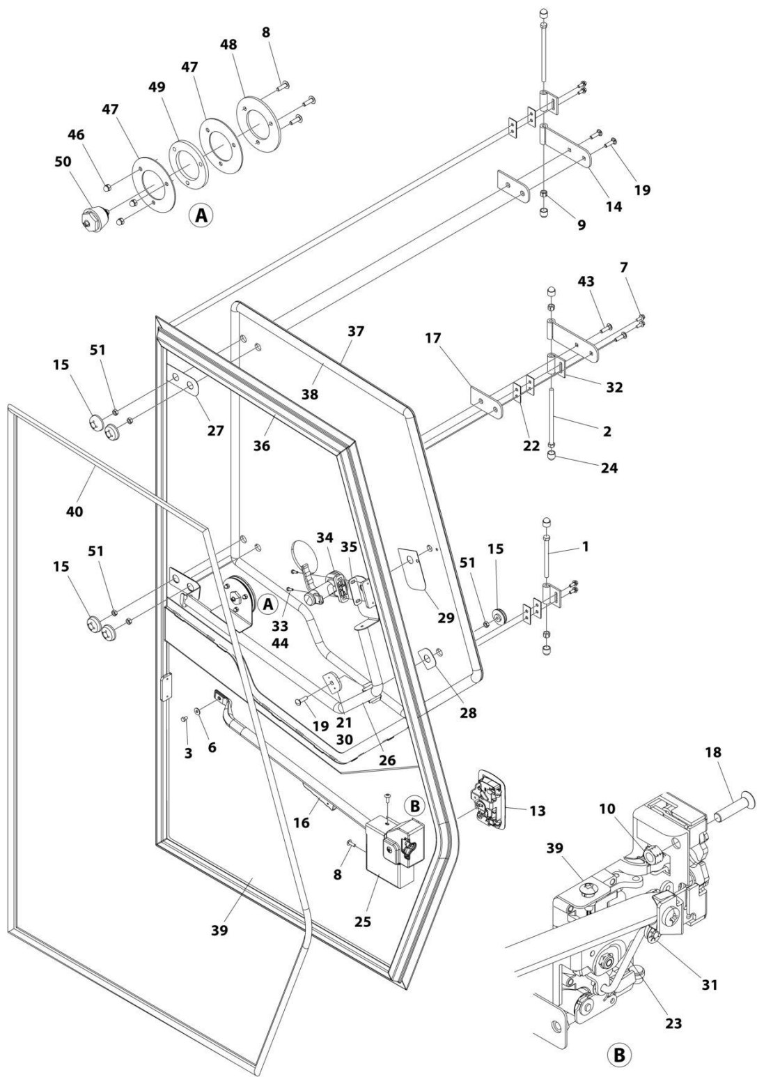
FIGURE 6-14. DOOR ASSEMBLY (Prior to SN 0160126061)
