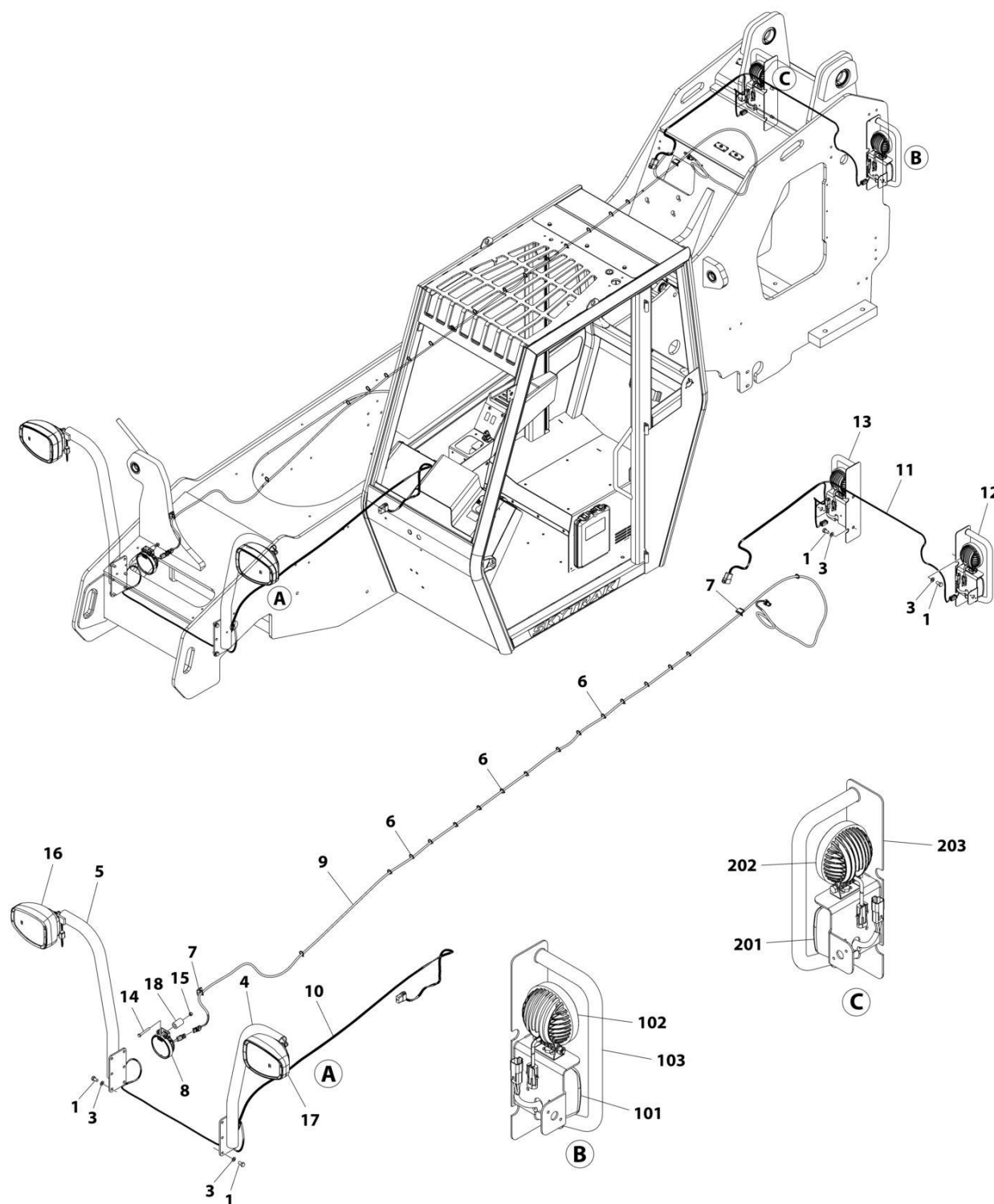
FIGURE 10-40. LIGHTS - ROADLIGHTS INSTALLATION (SN 0160129762 to Present)
