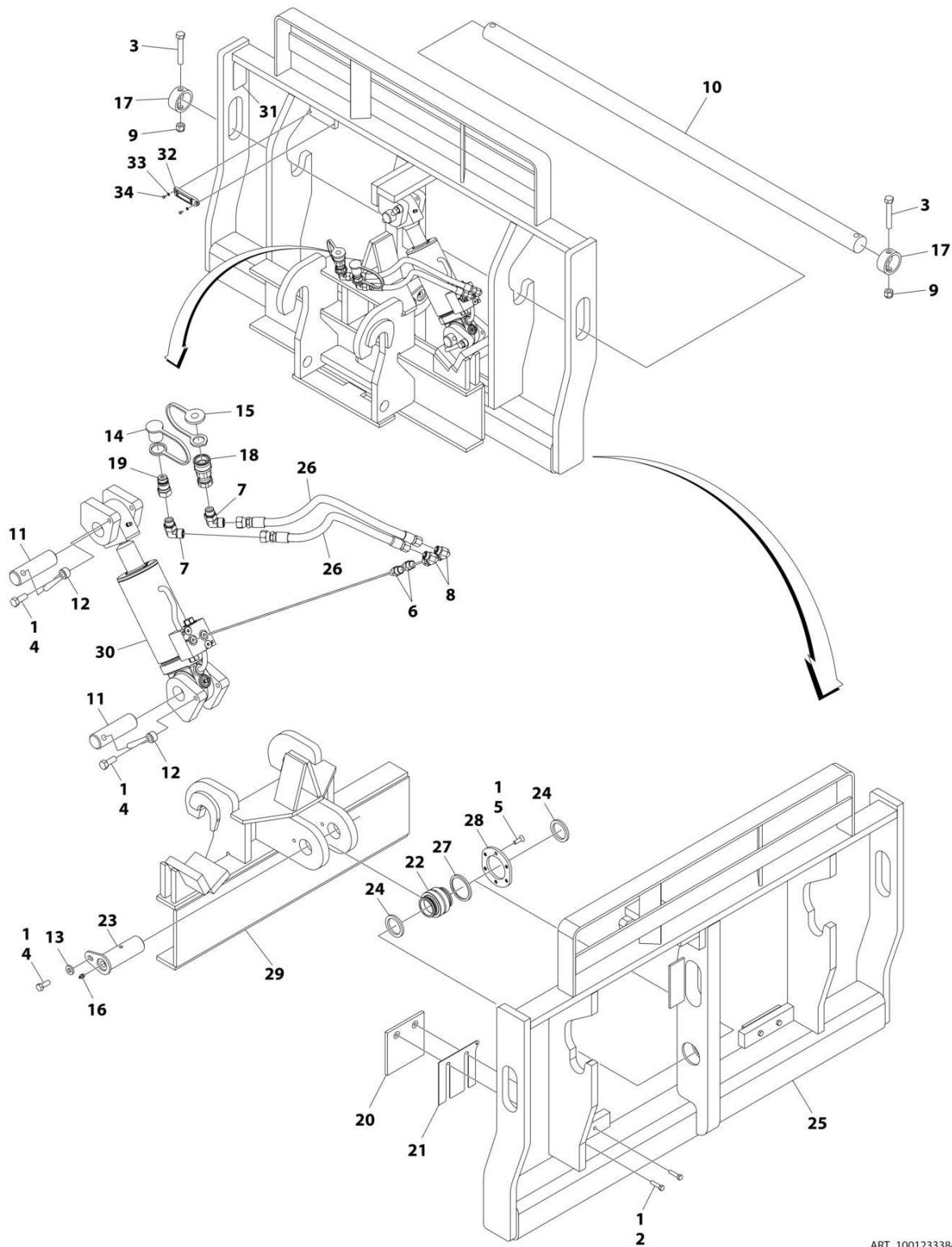
FIGURE 3-21. CARRIAGE ASSEMBLY - 60IN/12000# CAPACITY SIDE TILT (Prior to SN 0160124220, Prior to SN 0160124220)
