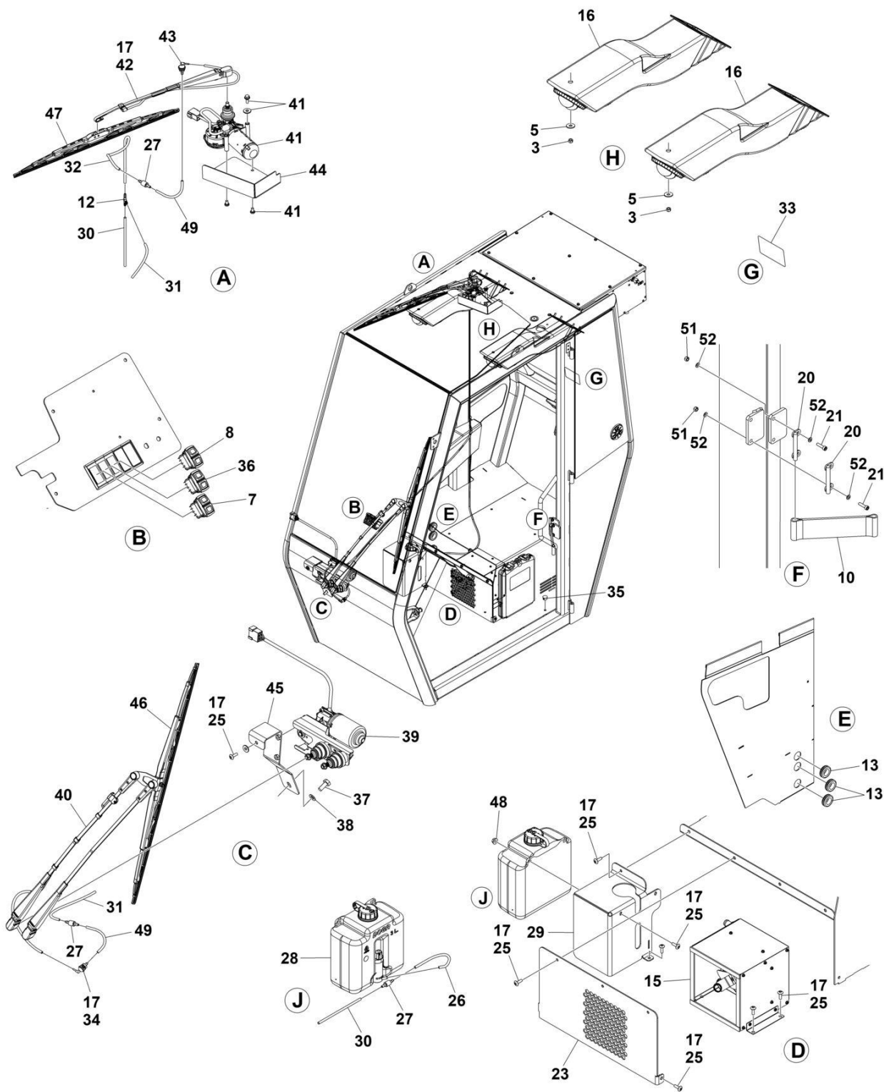
FIGURE 6-21. CAB HEATER INSTALLATION (SN 0160129762 to Present)
