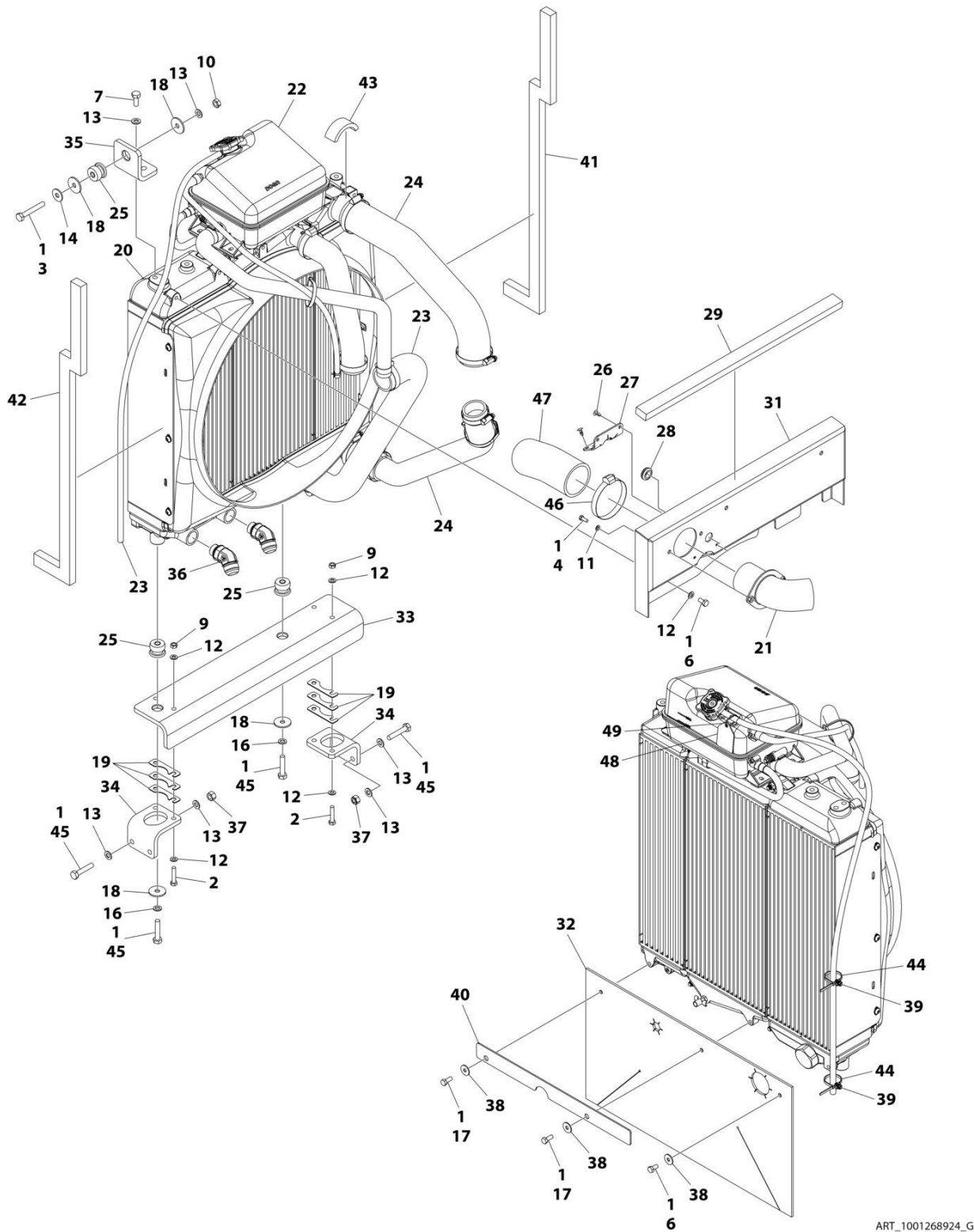
FIGURE 4-17. ENGINE COOLING SYSTEM INSTALLATION (PVC 2305) (SN 0160125282 to Present, SN 0160125419 to Present)
