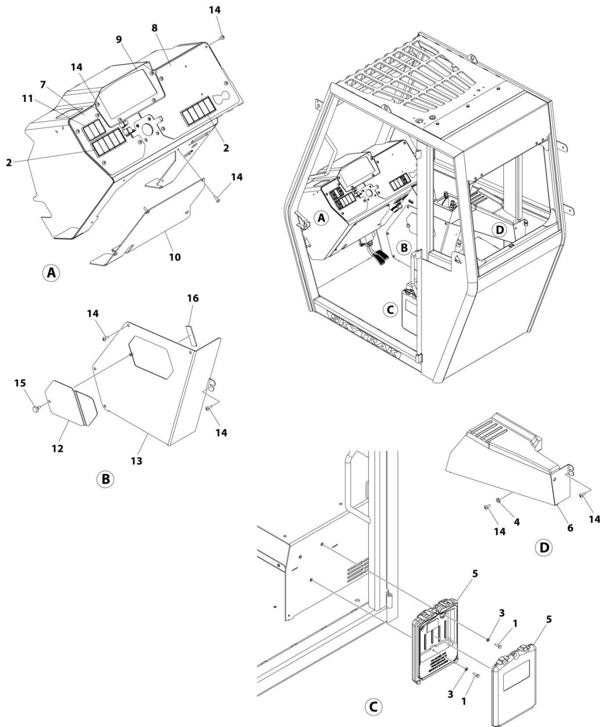
FIGURE 6-6. CAB INTERIOR INSTALLATION (Prior to SN 0160127612)
