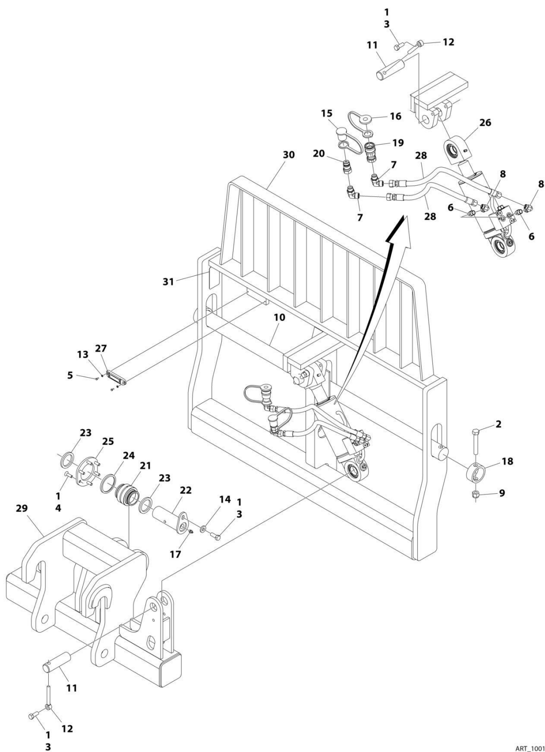
FIGURE 3-19. CARRIAGE ASSEMBLY - 50IN/12000# CAPICITY SIDE TILT (SN 0160124220 to Present, SN 0160124220 to Present)
