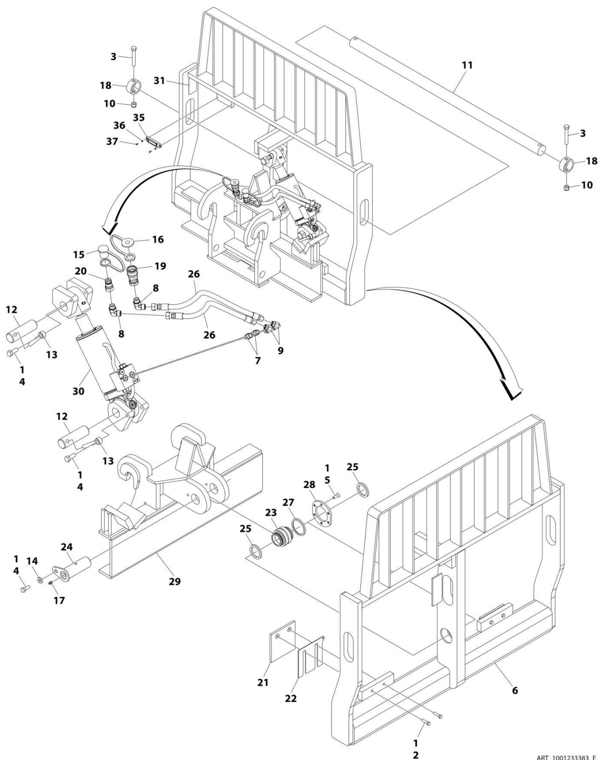
FIGURE 3-18. CARRIAGE ASSEMBLY - 50IN/12000# CAPICITY SIDE TILT (Prior to SN 0160124220, Prior to SN 0160124220)
