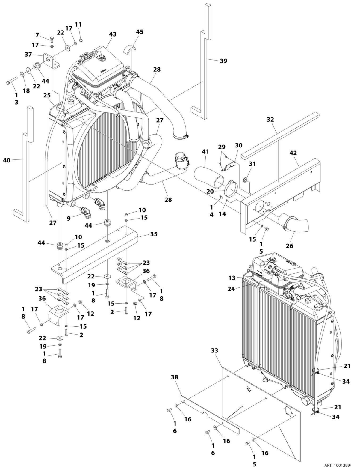
FIGURE 4-18. ENGINE COOLING SYSTEM INSTALLATION (PVC 2311)
