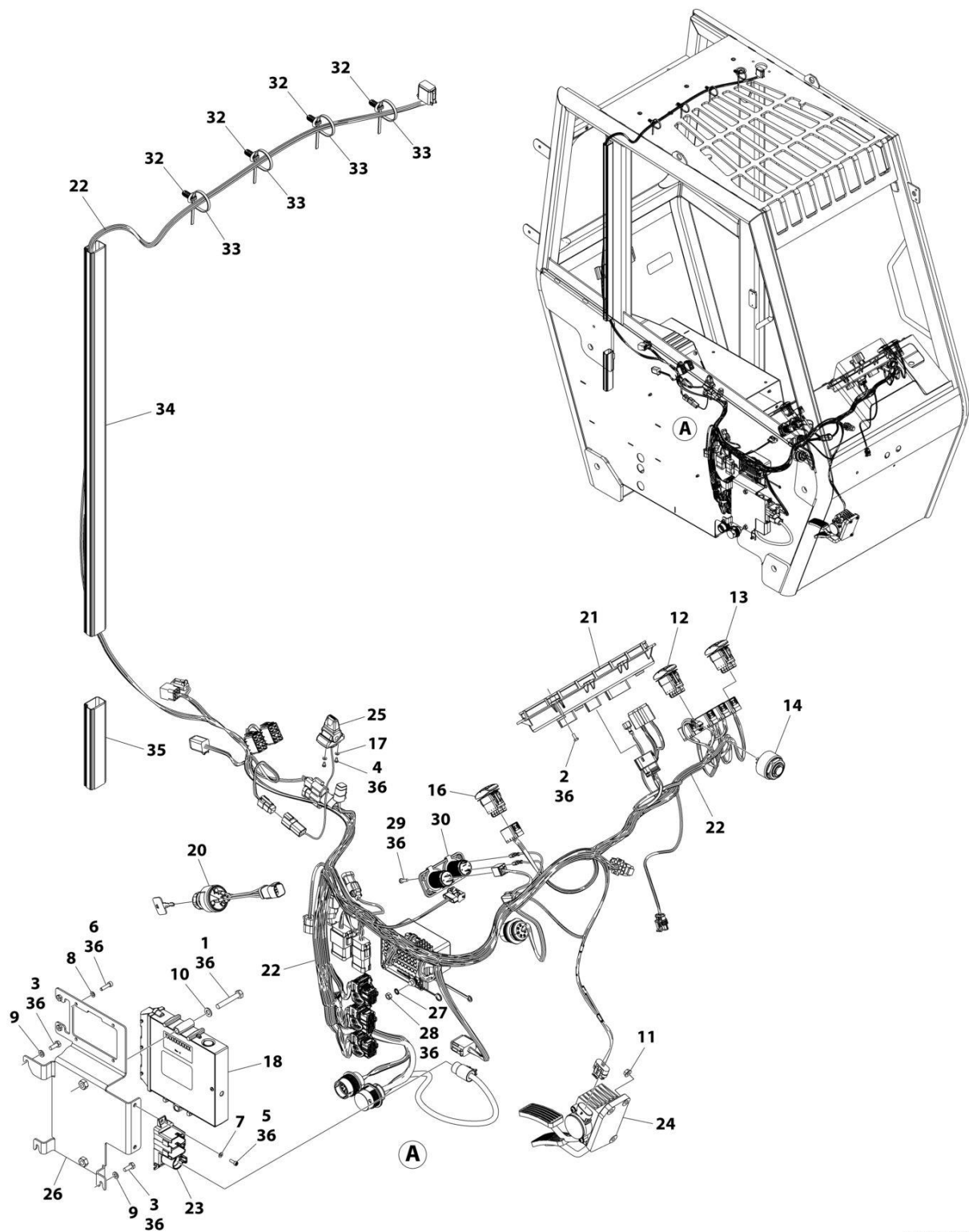
FIGURE 10-13. CAB ELECTRICAL INSTALLATION (Prior to SN 0160127612)
