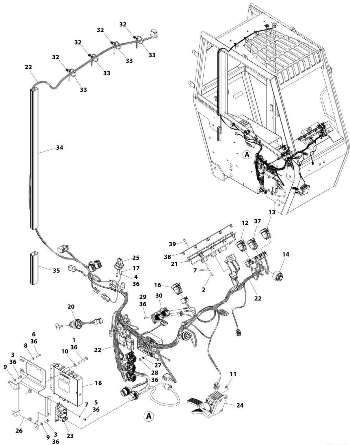
FIGURE 10-14. CAB ELECTRICAL INSTALLATION (SN 0160127872 to Present)
