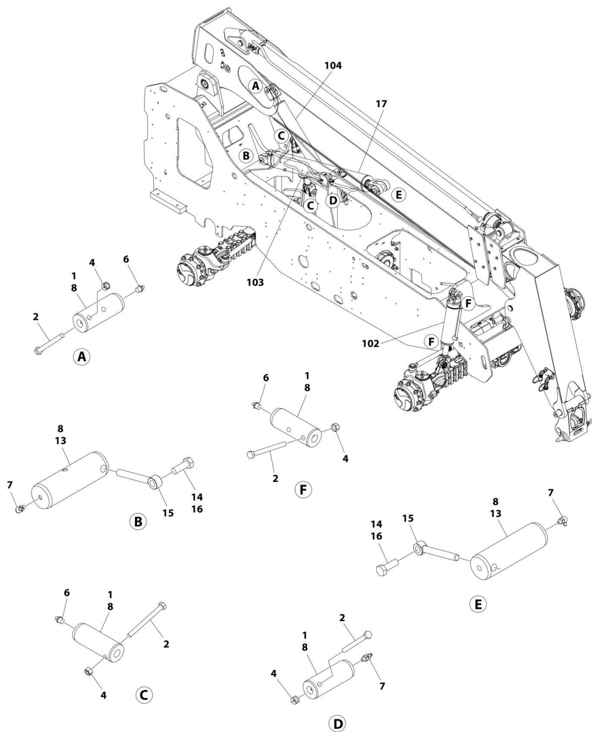
FIGURE 9-9. CYLINDERS INSTALLATION
