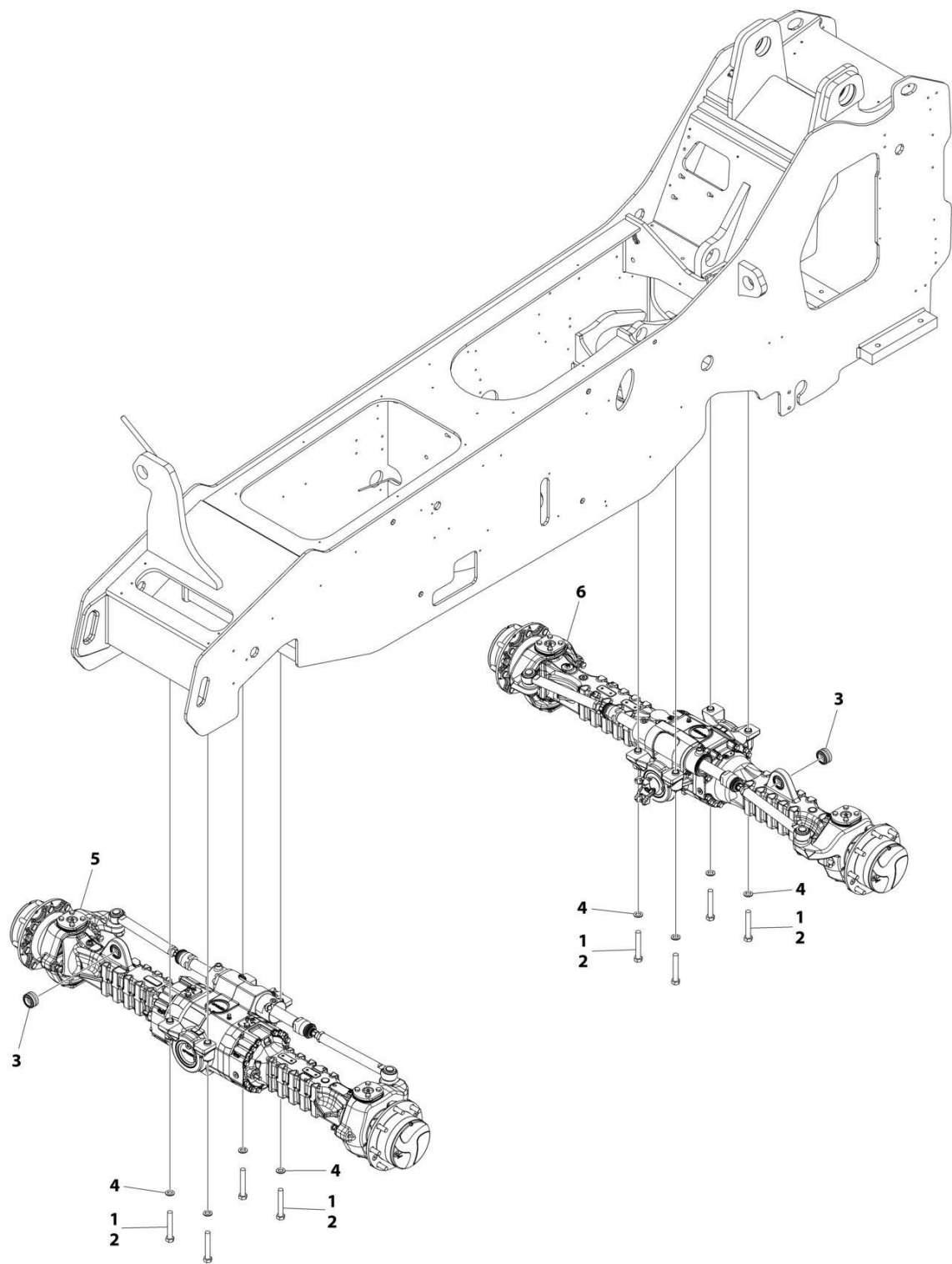
FIGURE 5-1. AXLES INSTALLATION (PVC 2305)
