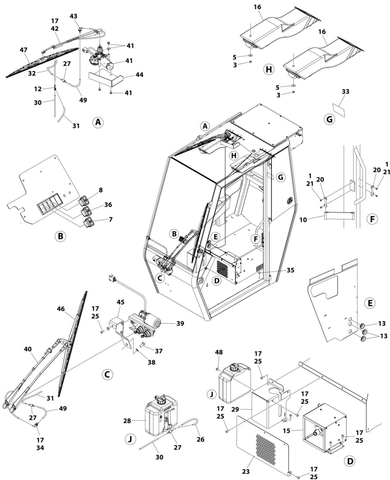
FIGURE 6-20. CAB HEATER INSTALLATION (Prior to SN 0160129391)
