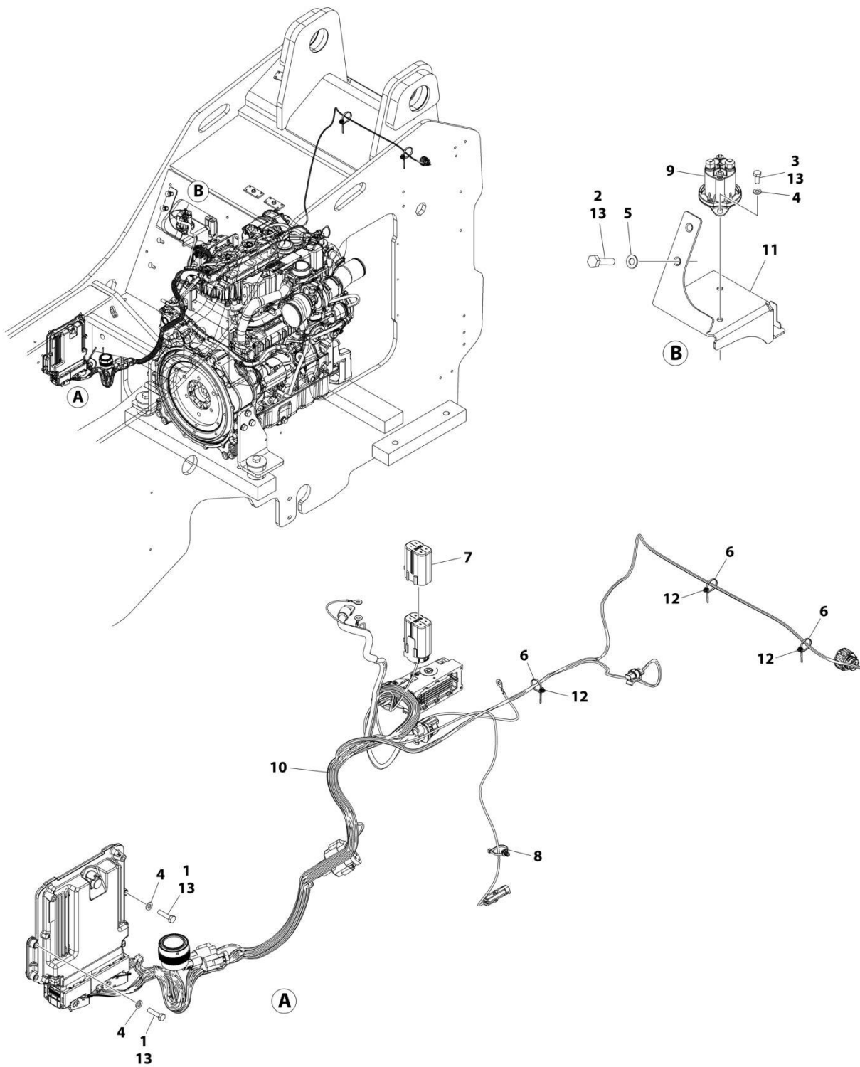
FIGURE 4-10. ENGINE ELECTRICAL INSTALLATION (PVC 2305)
