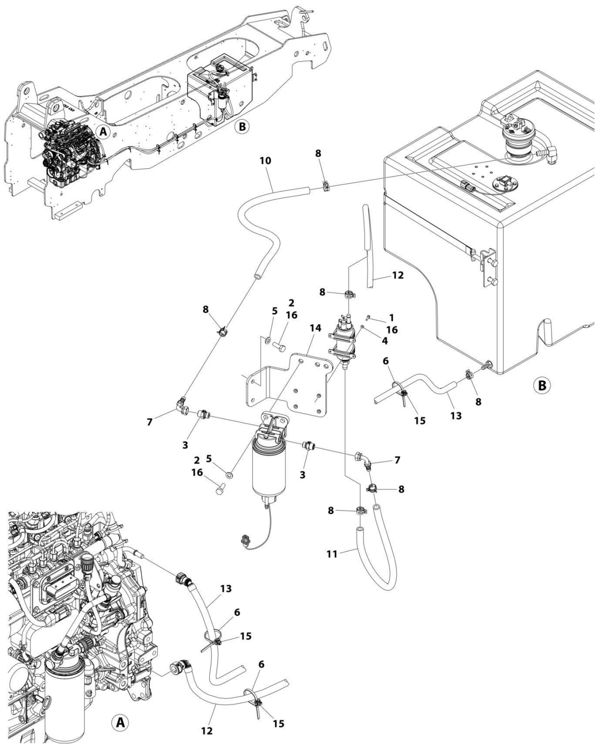
FIGURE 4-13. ENGINE FUEL SYSTEM INSTALLATION (HRC ENGINES)
