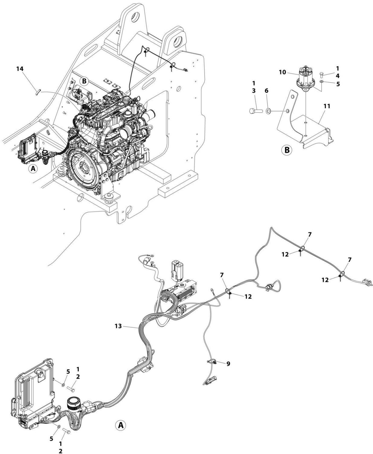
FIGURE 4-11. ENGINE ELECTRICAL INSTALLATION (PVC 2311)
