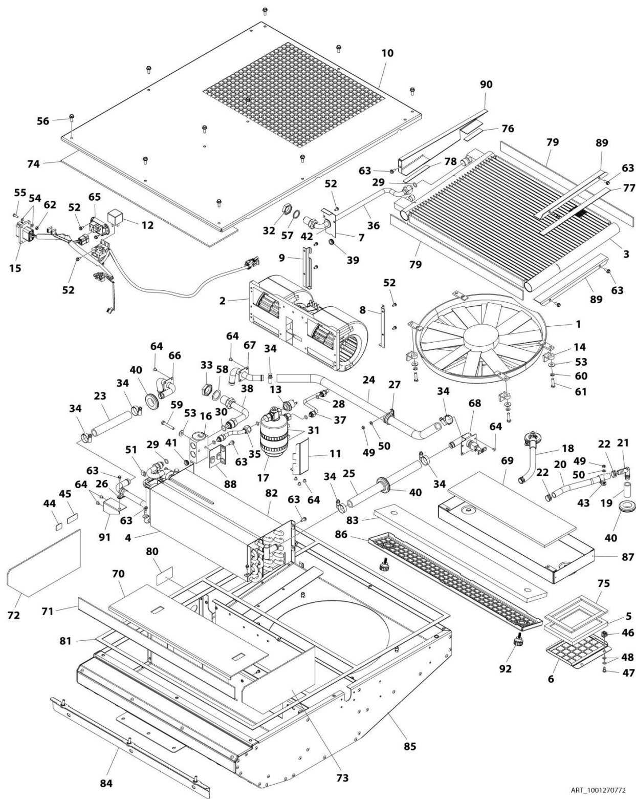
FIGURE 6-18. HVAC ASSEMBLY
