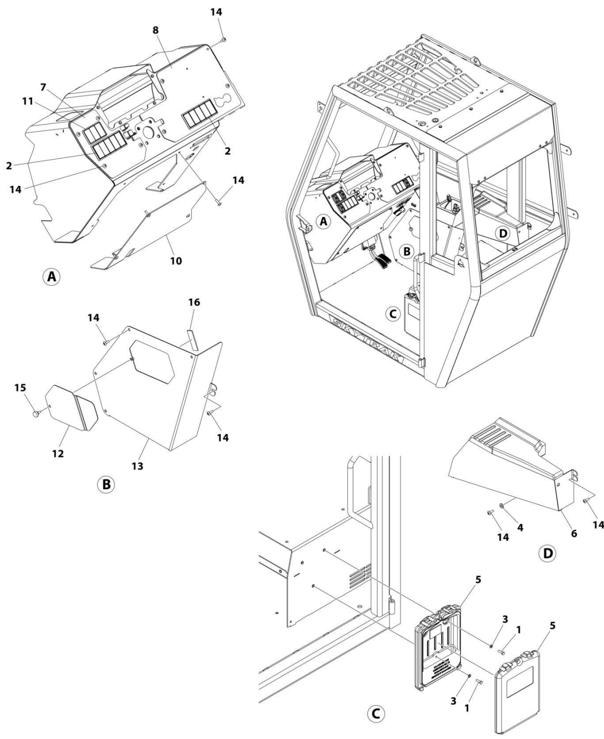
FIGURE 6-7. CAB INTERIOR INSTALLATION (SN 0160127872 to Present)
