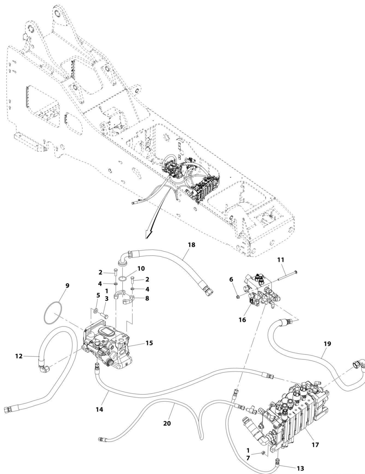
FIGURE 8-20. PUMP HYDRAULICS INSTALLATION
