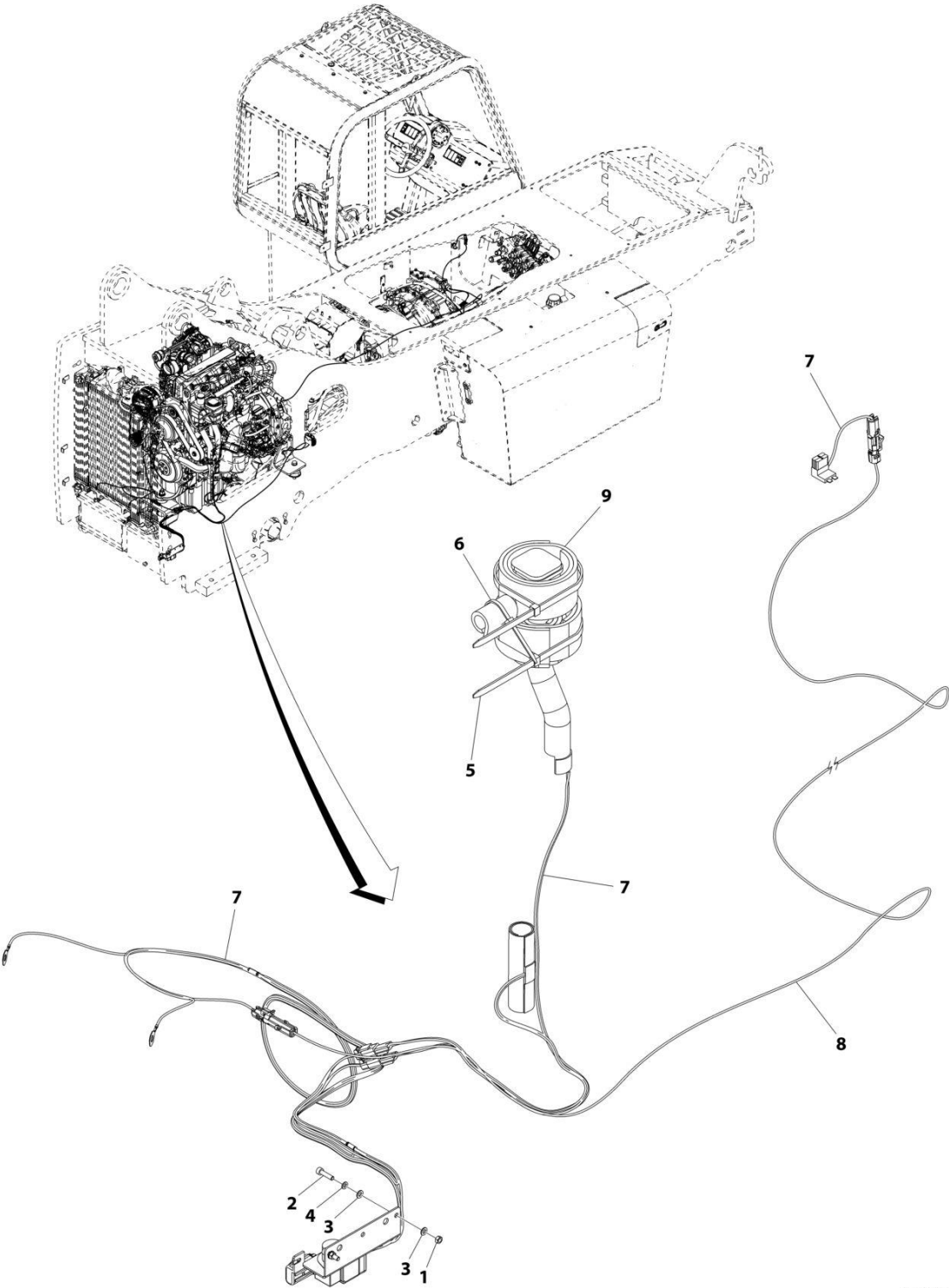
FIGURE 10-15. BREATHER HEATER INSTALLATION
