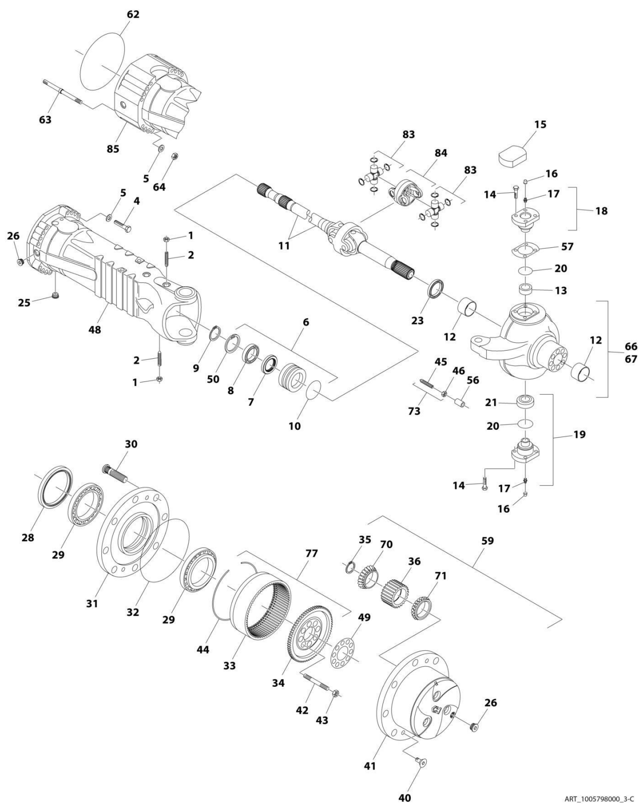
FIGURE 5-26. FRONT AXLE - HUB REDUCTION (74HP)
