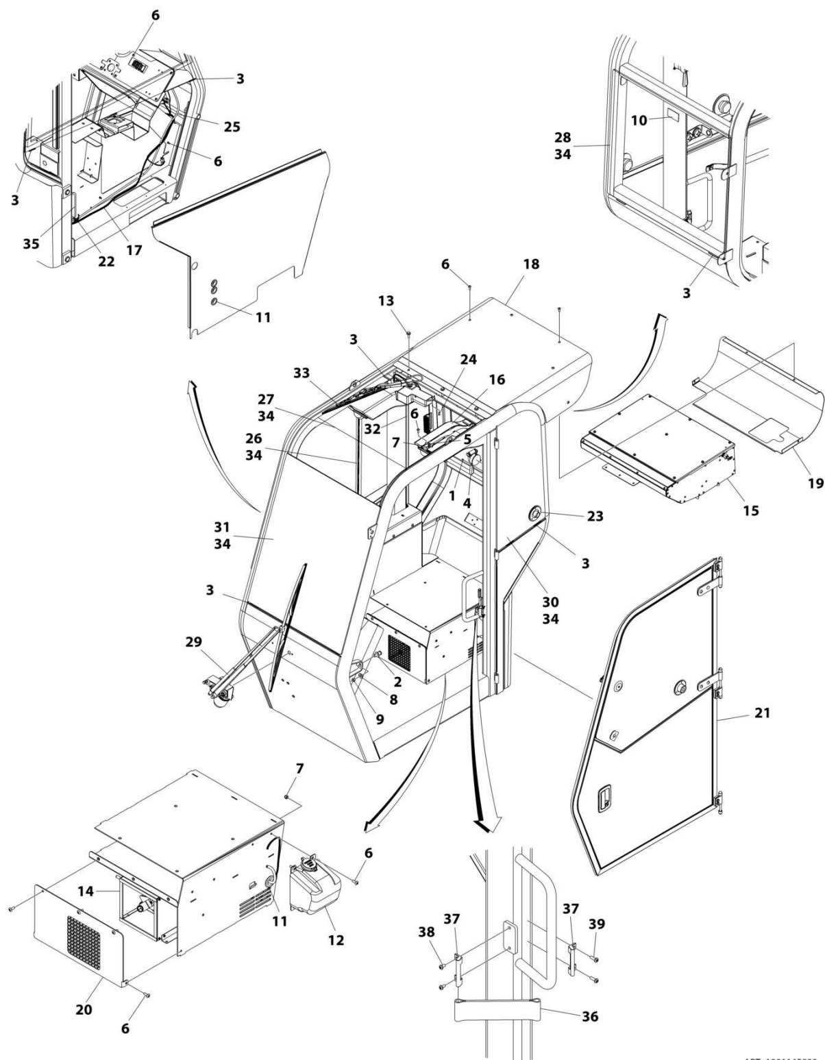
FIGURE 6-11. CAB ENCLOSURE WITH HEATER
