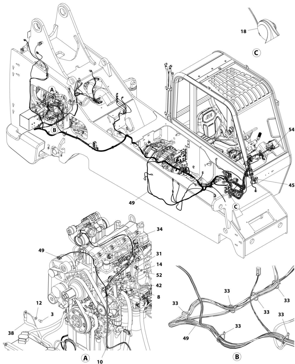
FIGURE 10-2. ELECTRICAL INSTALLATION (74HP) (ULS) (SN 0160125882 to Present)
