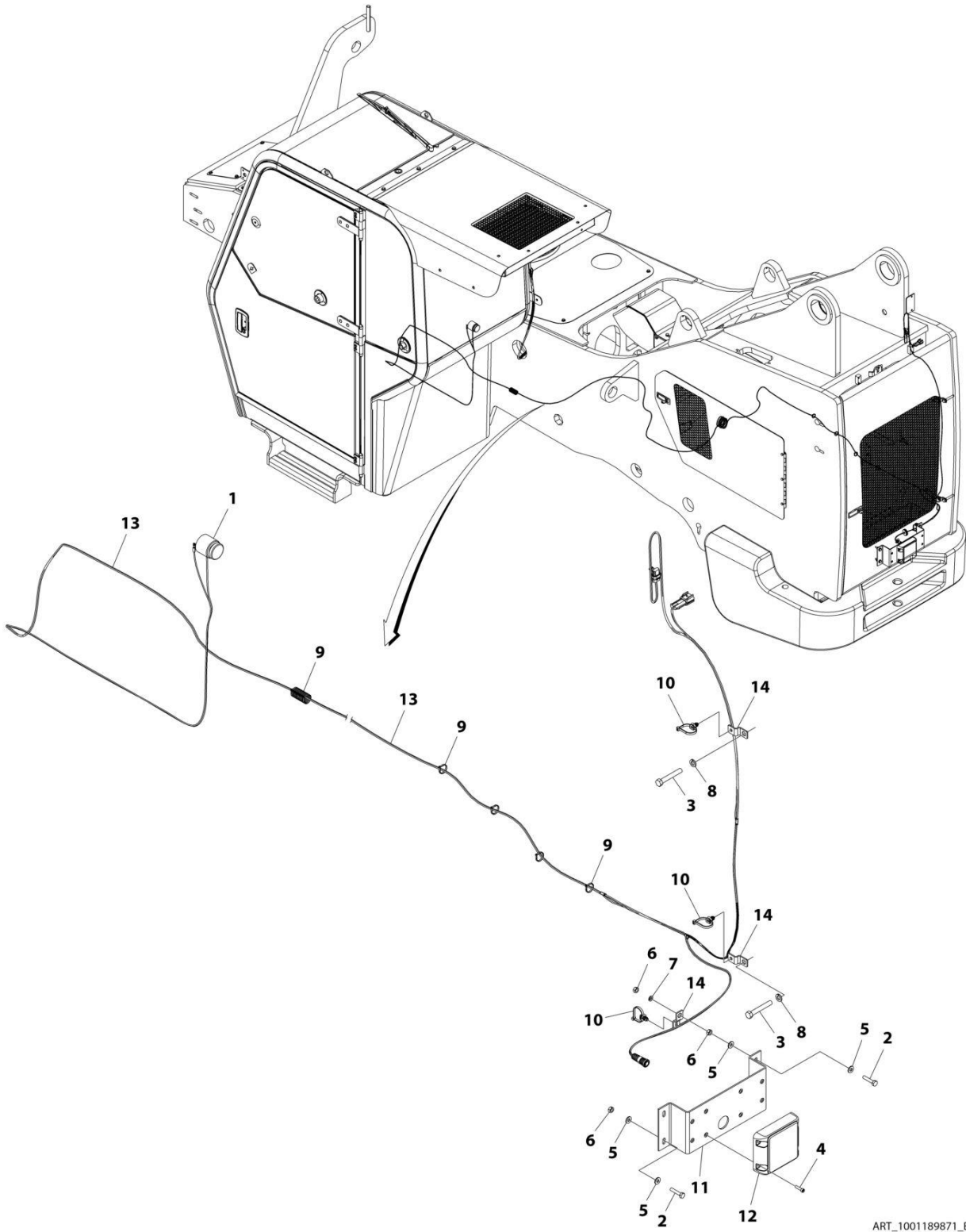
FIGURE 10-54. REVERSE SENSING SYSTEM INSTALLATION
