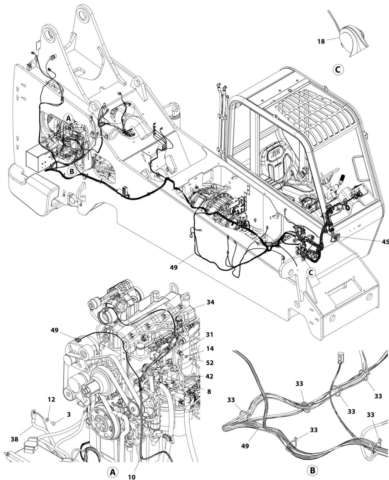
FIGURE 10-1. ELECTRICAL INSTALLATION (74HP) (ULS)
