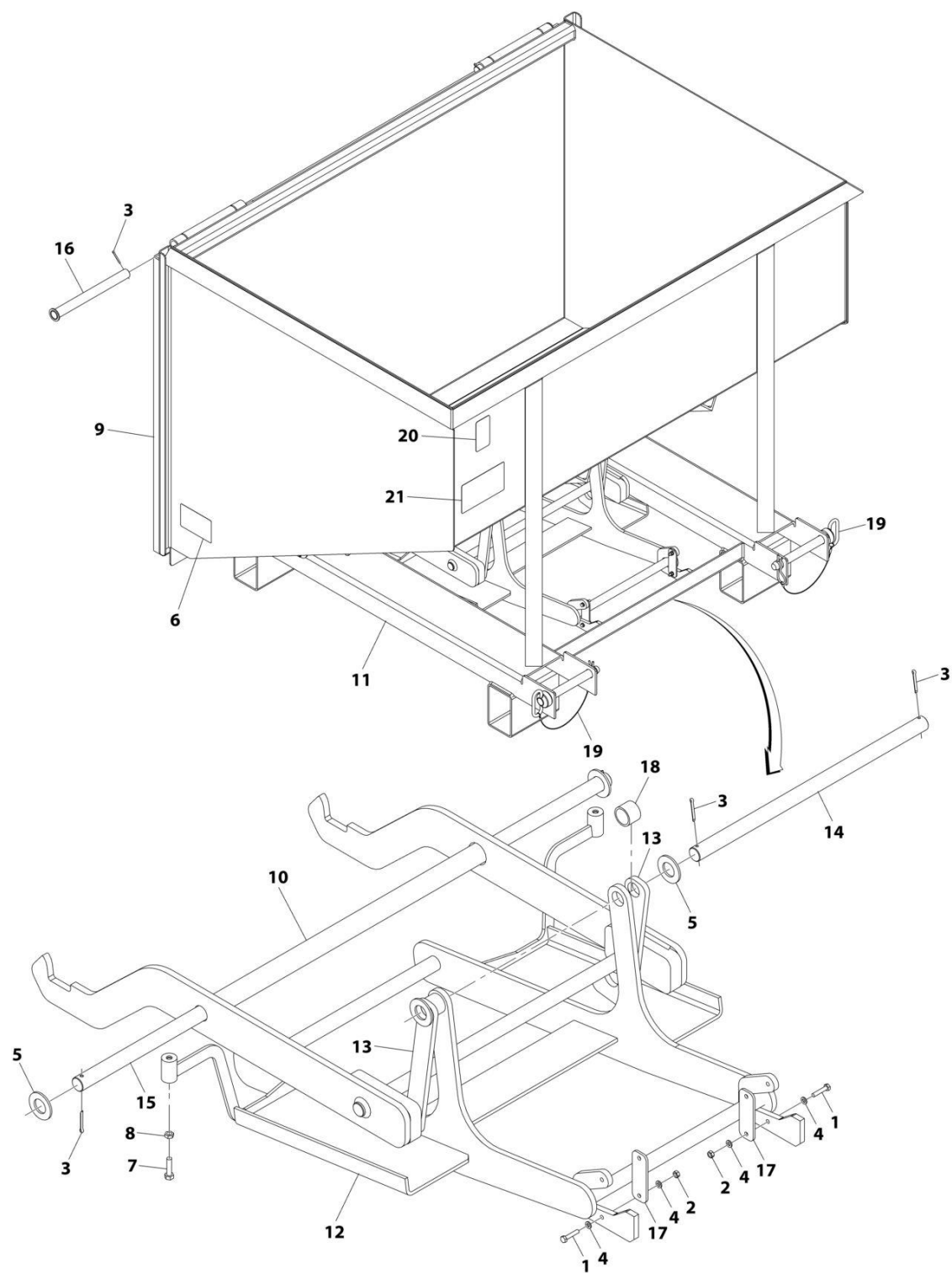
FIGURE 3-50. TRASHER HOPPER
