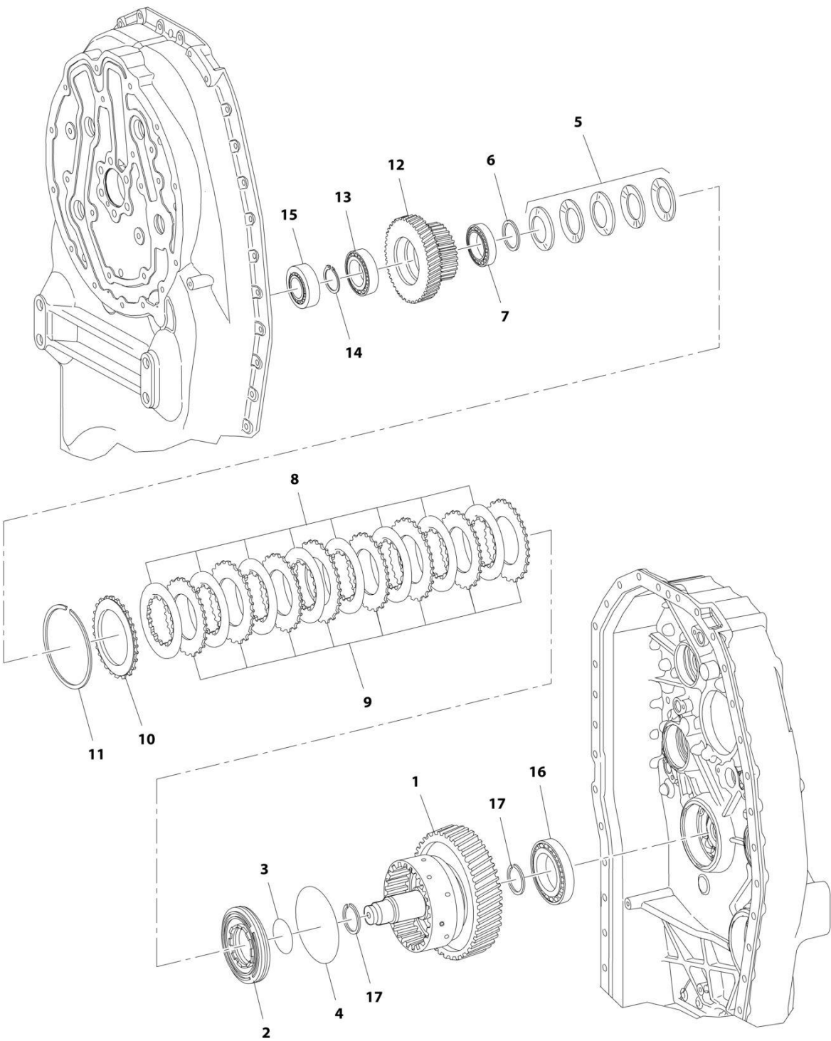
FIGURE 5-6. TRANSMISSION, COUPLING GROUP 3
