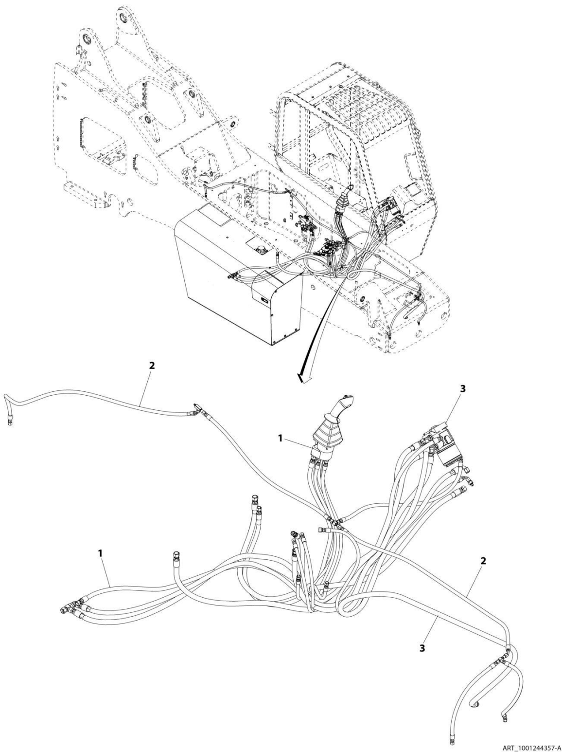
FIGURE 8-7. CAB HYDRAULICS INSTALLATION
