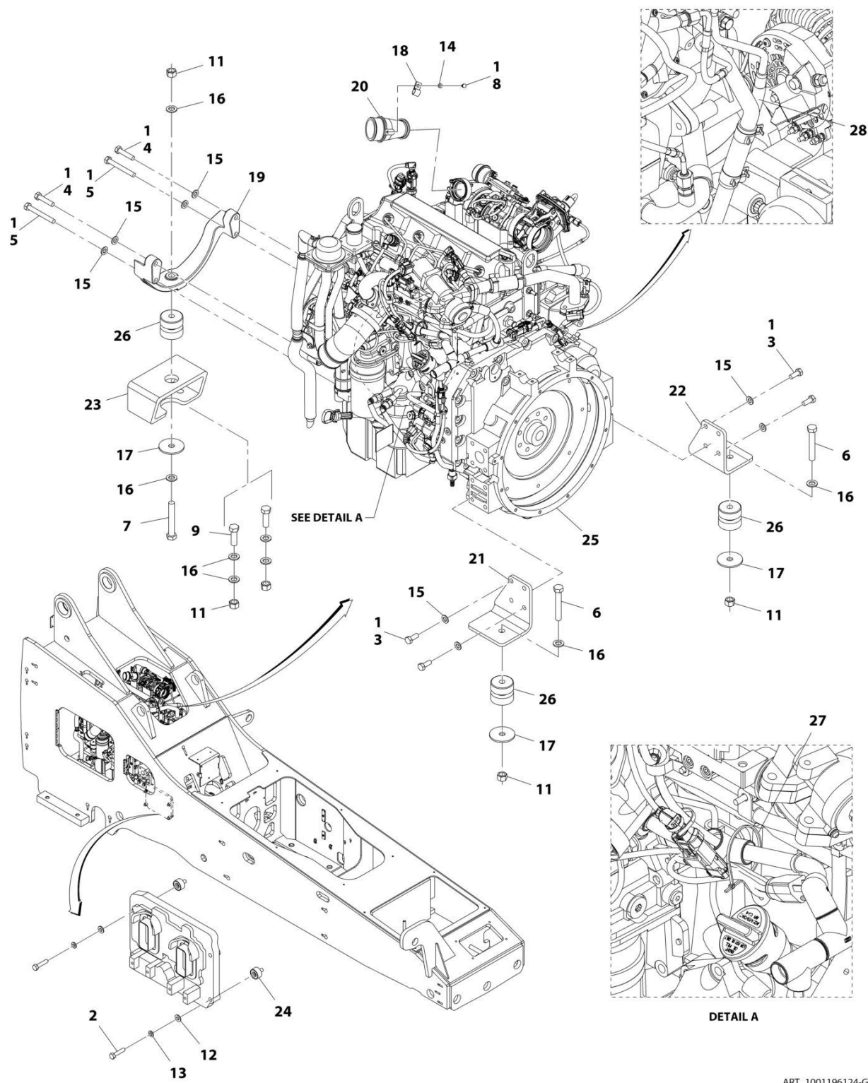
FIGURE 4-1. ENGINE INSTALLATION - 74HP (ULS)
