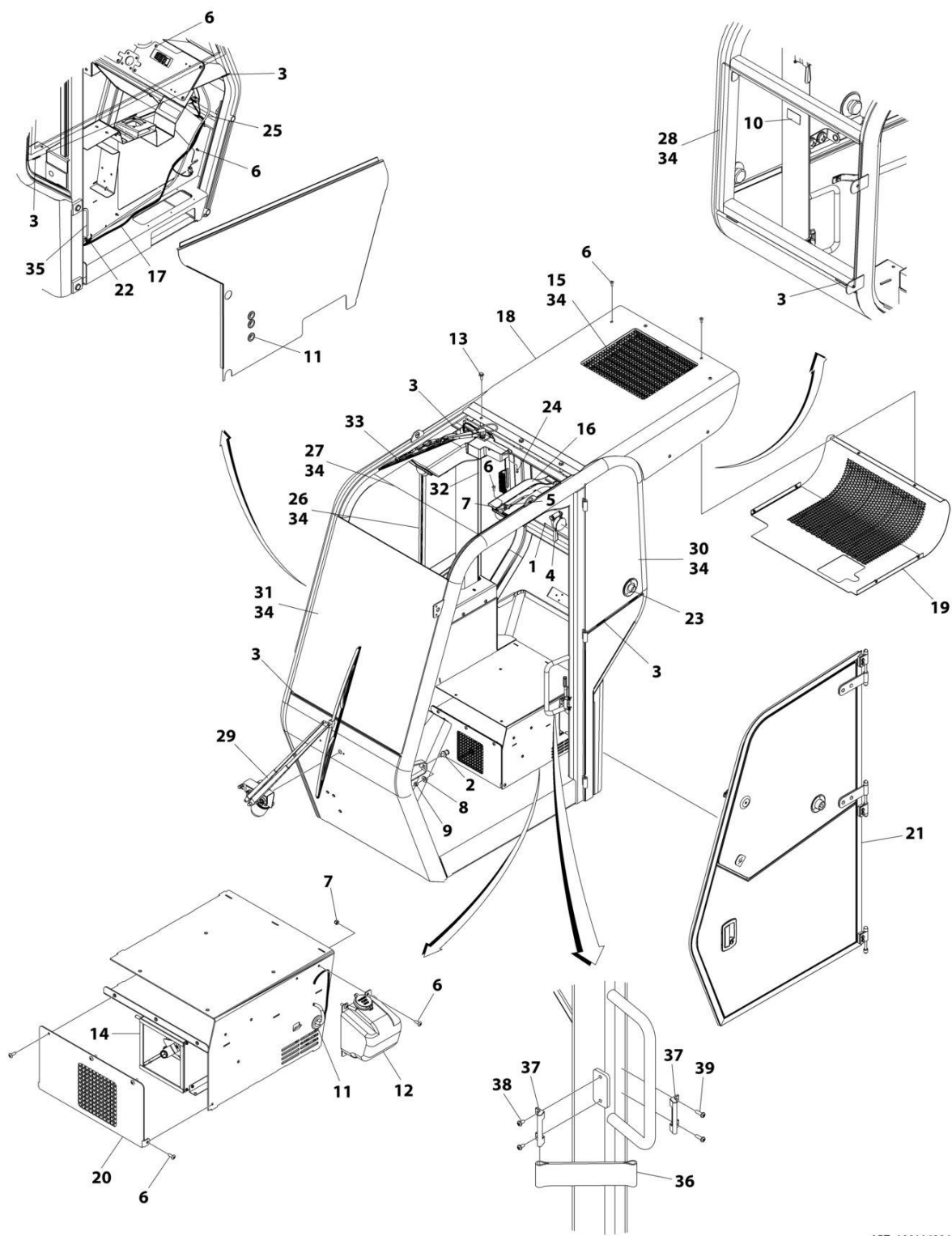
FIGURE 6-17. CAB ENCLOSURE WITH HEATER & AC
