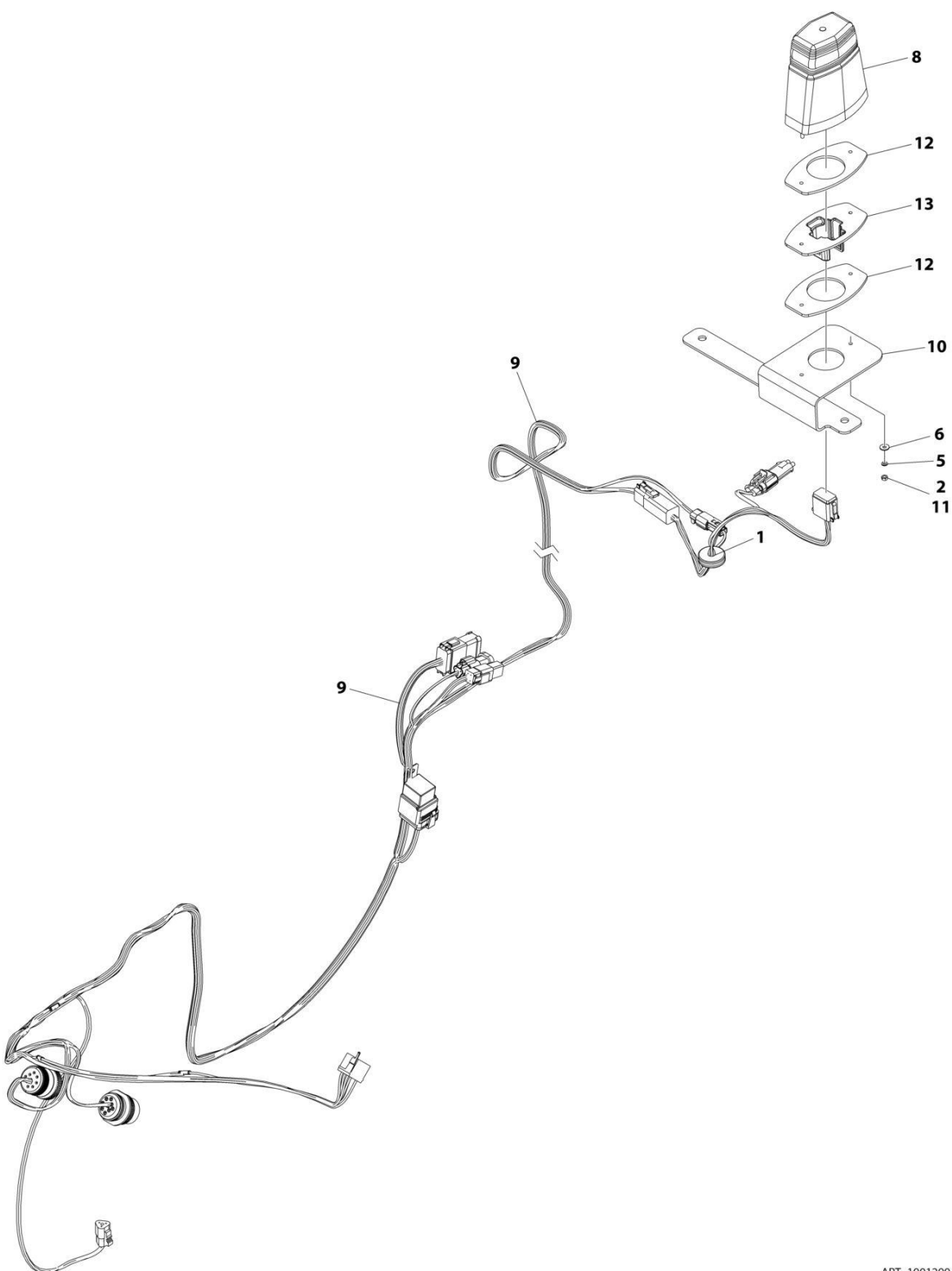
FIGURE 10-28. CLEARSKY INSTALLATION - SMART FLEET (OPEN CAB) (SN 0160126735 to Present)
