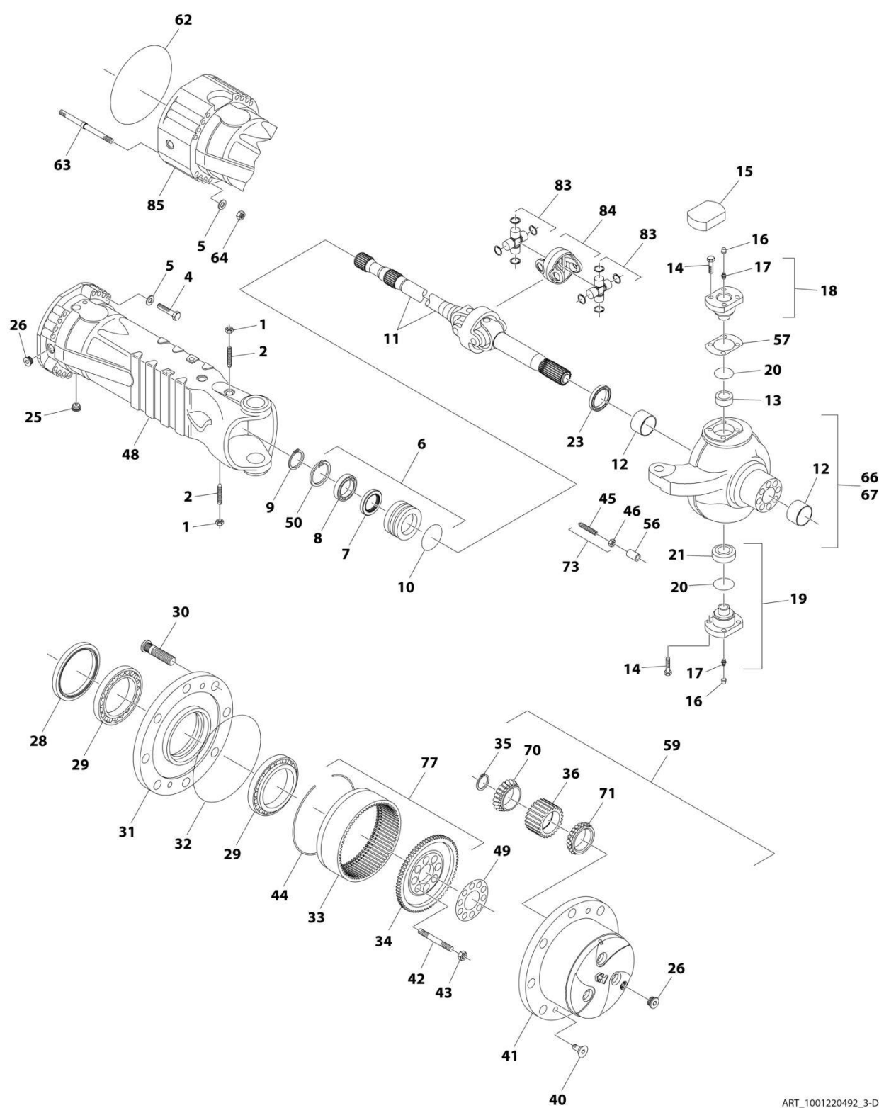
FIGURE 5-39. FRONT AXLE - HUB REDUCTION (110HP)
