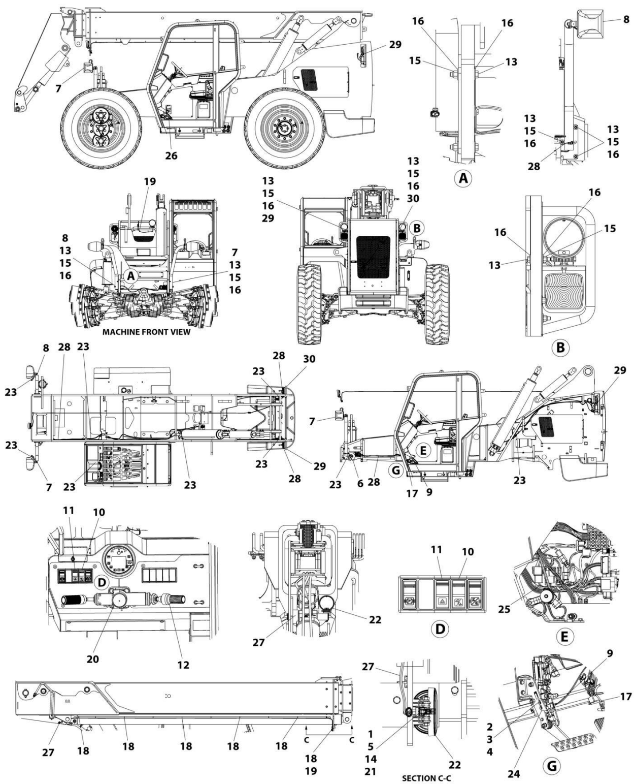
FIGURE 10-40. LED ROAD LIGHT INSTALLATION
