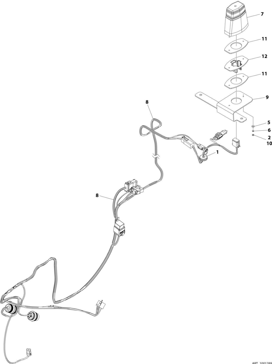
FIGURE 10-26. CLEARSKY INSTALLATION - SMART FLEET (CLOSED CAB) (SN 0160126735 to Present)
