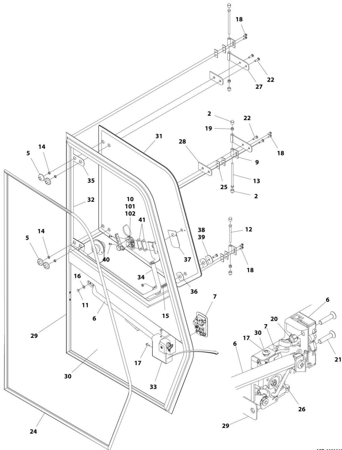
FIGURE 6-18. CAB DOOR ASSEMBLY
