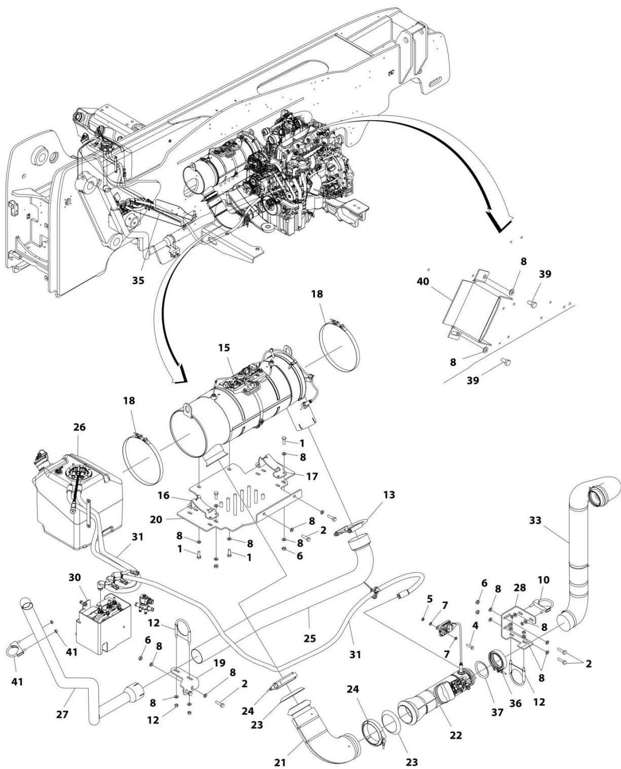
FIGURE 4-32. EXHAUST INSTALLATION, 110HP (ULS)
