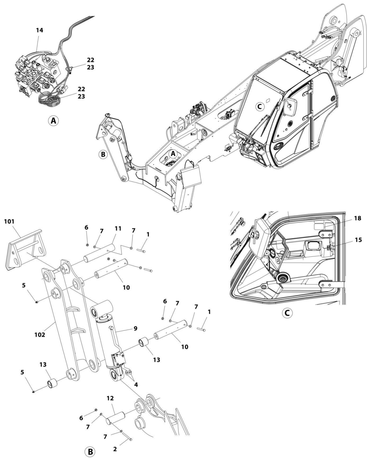
FIGURE 1-10. OUTRIGGERS INSTALLATION
