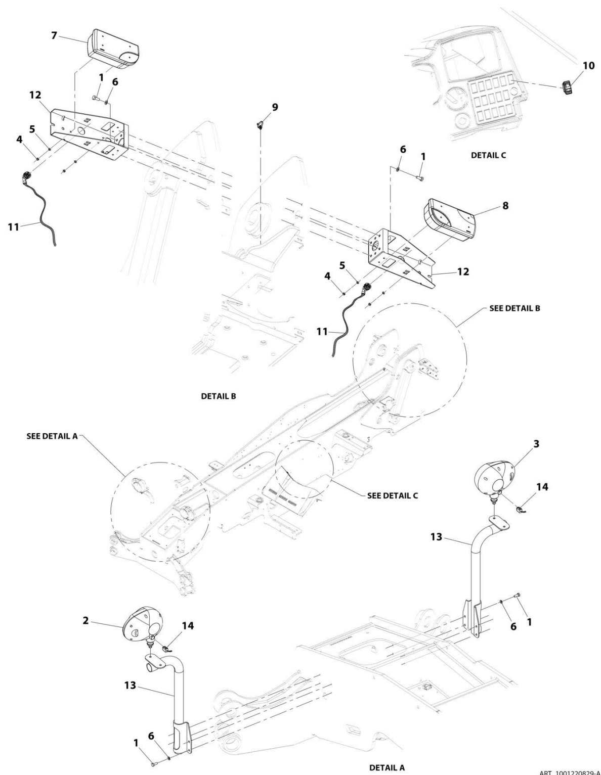
FIGURE 10-68. LIGHTS - ROADLIGHTS INSTALLATION
