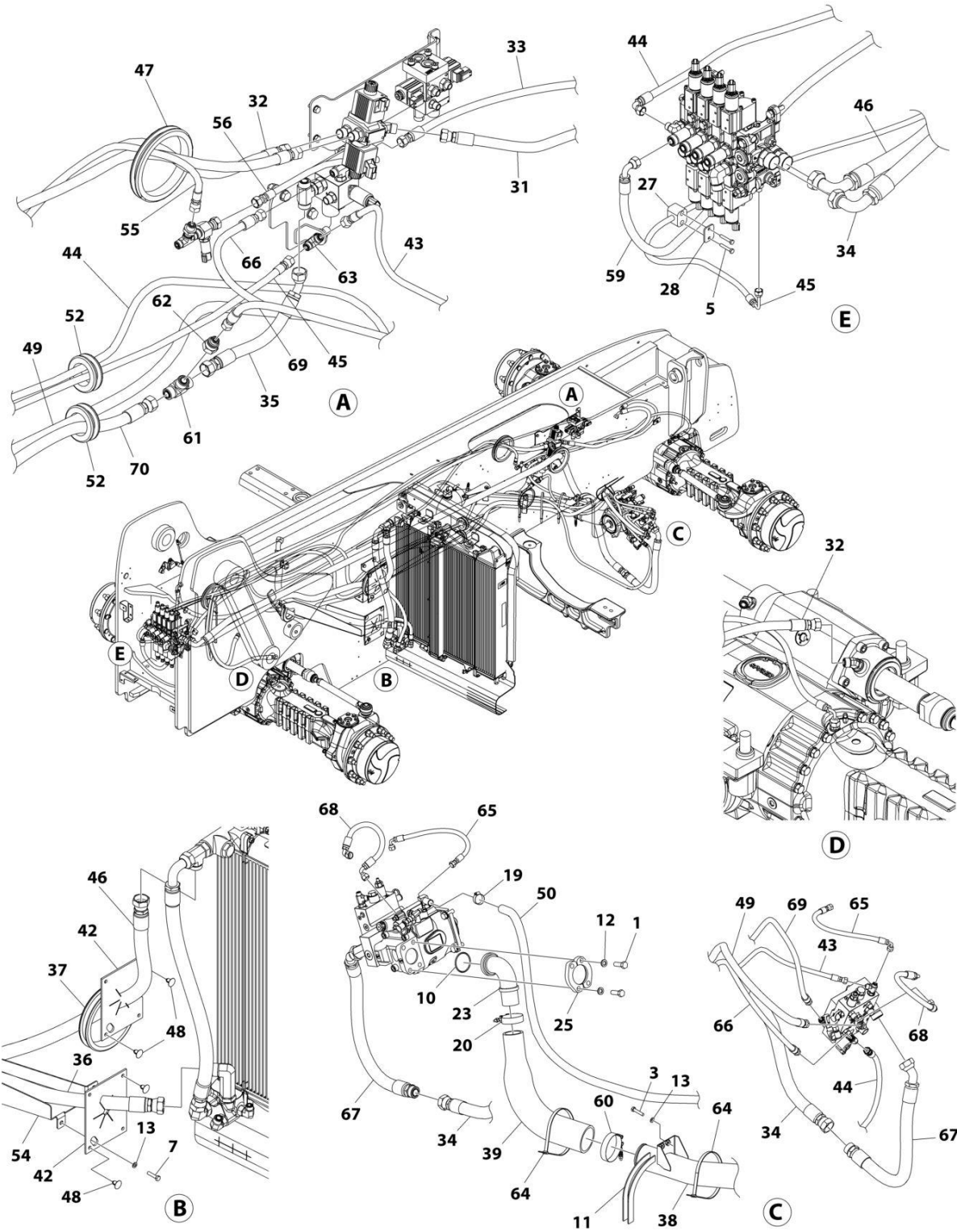
FIGURE 8-14. FRAME HYDRAULICS INSTALLATION
