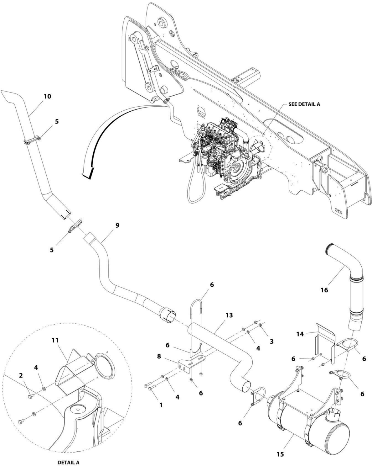
FIGURE 4-29. EXHAUST INSTALLATION, 110HP (LS)
