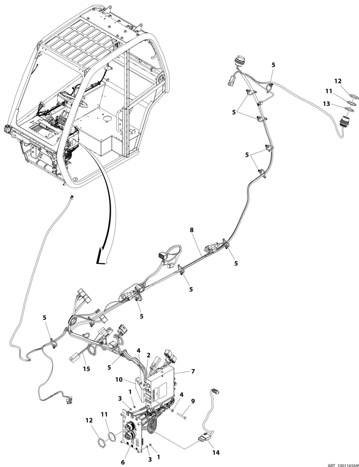
FIGURE 10-21. CAB ELECTRICAL INSTALLATION
