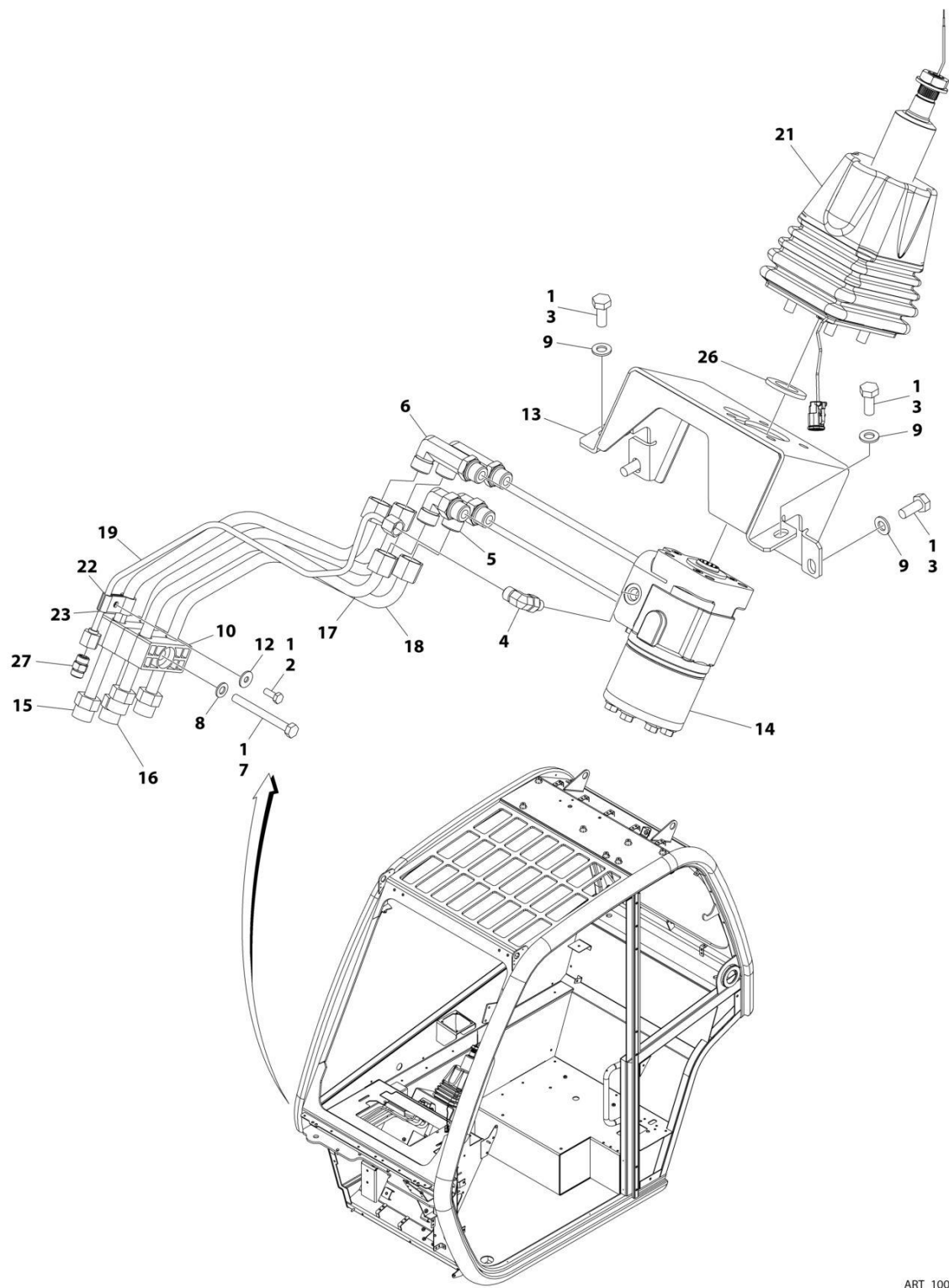
FIGURE 7-14. STEERING COLUMN INSTALLATION
