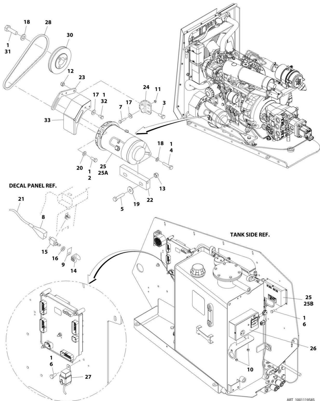
FIGURE 3-21. 2800W GENERATOR INSTALLATION - KUBOTA ENGINE MACHINES 220V/50HZ GENERATOR (ANSI EXPORT, AUSTRALIAN, CHINA, CE & UK CA SPECS)
