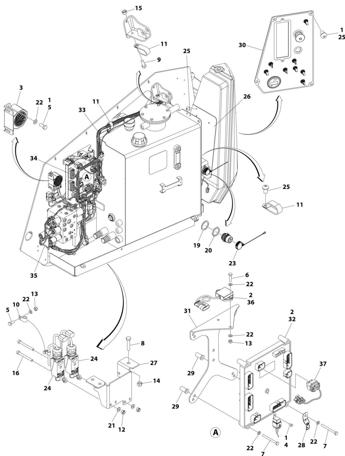
FIGURE 2-11. ELECTRICAL COMPONENTS INSTALLATION (ALL SPECS EXCEPT CE & UK CA)
