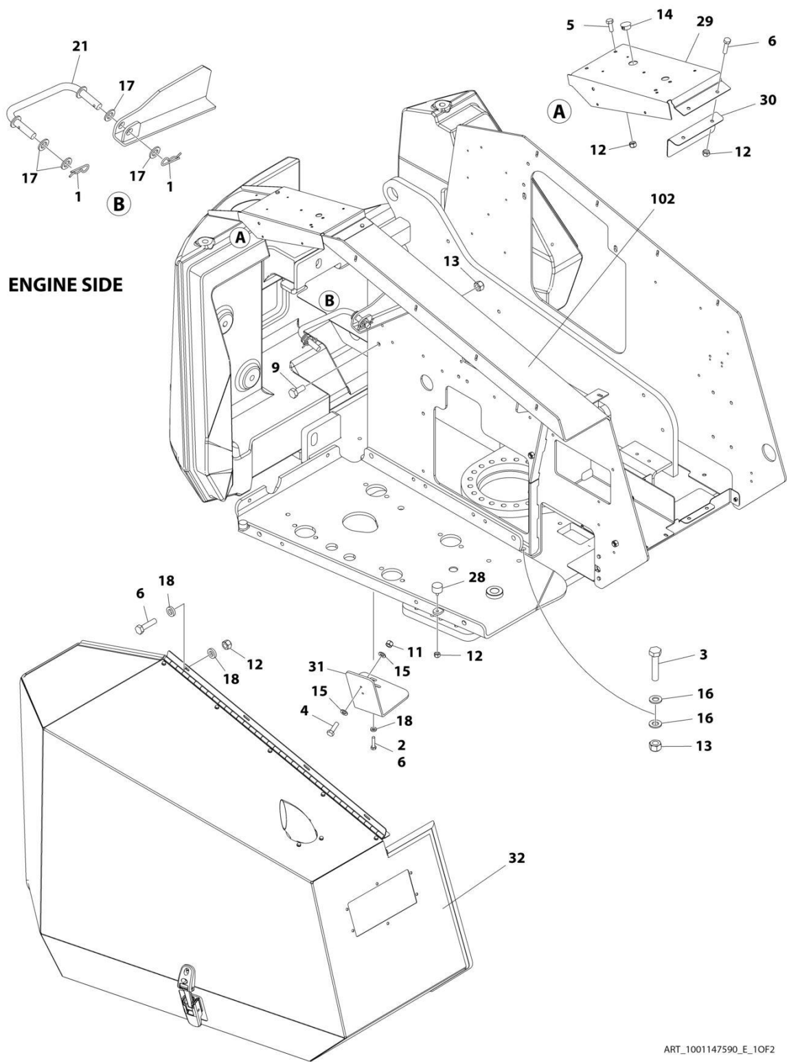
FIGURE 2-30. HOODS INSTALLATION (SN 0300297926 to Present)
