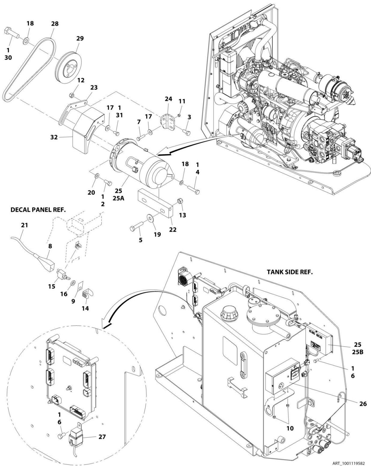
FIGURE 3-24. 3500W GENERATOR INSTALLATION - KUBOTA ENGINE MACHINES 120V/60HZ GENERATOR (ANSI, ANSI EXPORT, CHINA, CSA AND JAPANESE SPECS)
