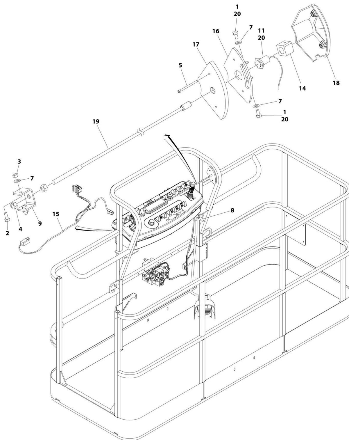
FIGURE 5-16. SKYLINE INSTALLATION
