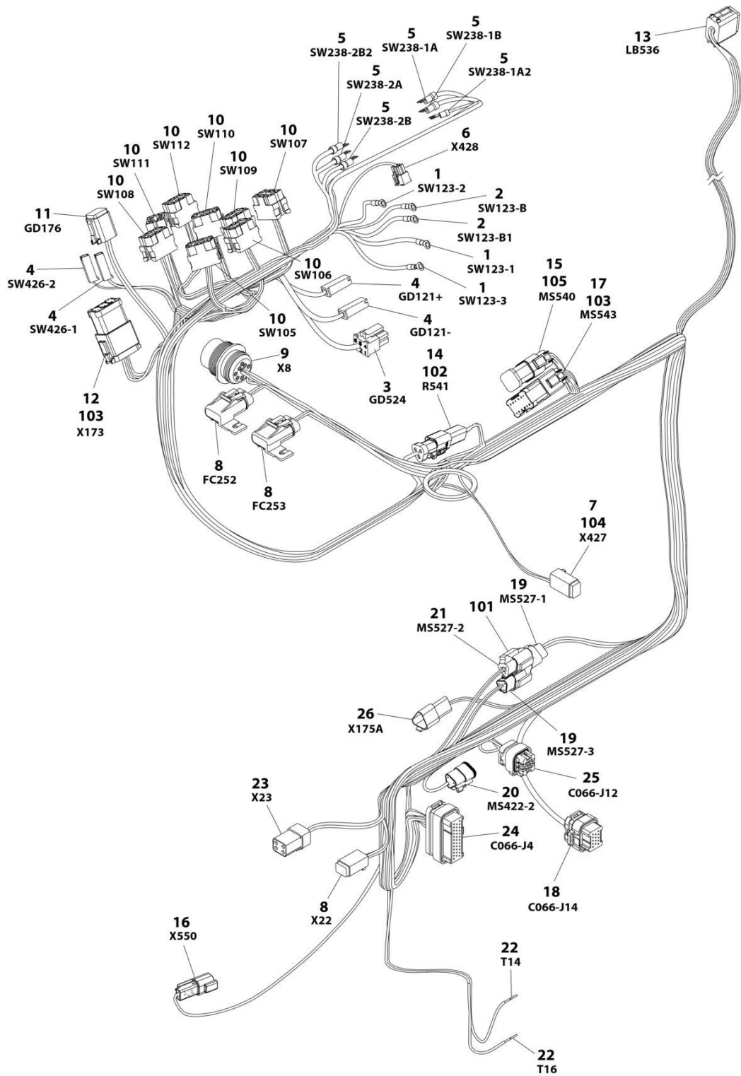
FIGURE 8-51. GROUND CONTROL HARNESS
