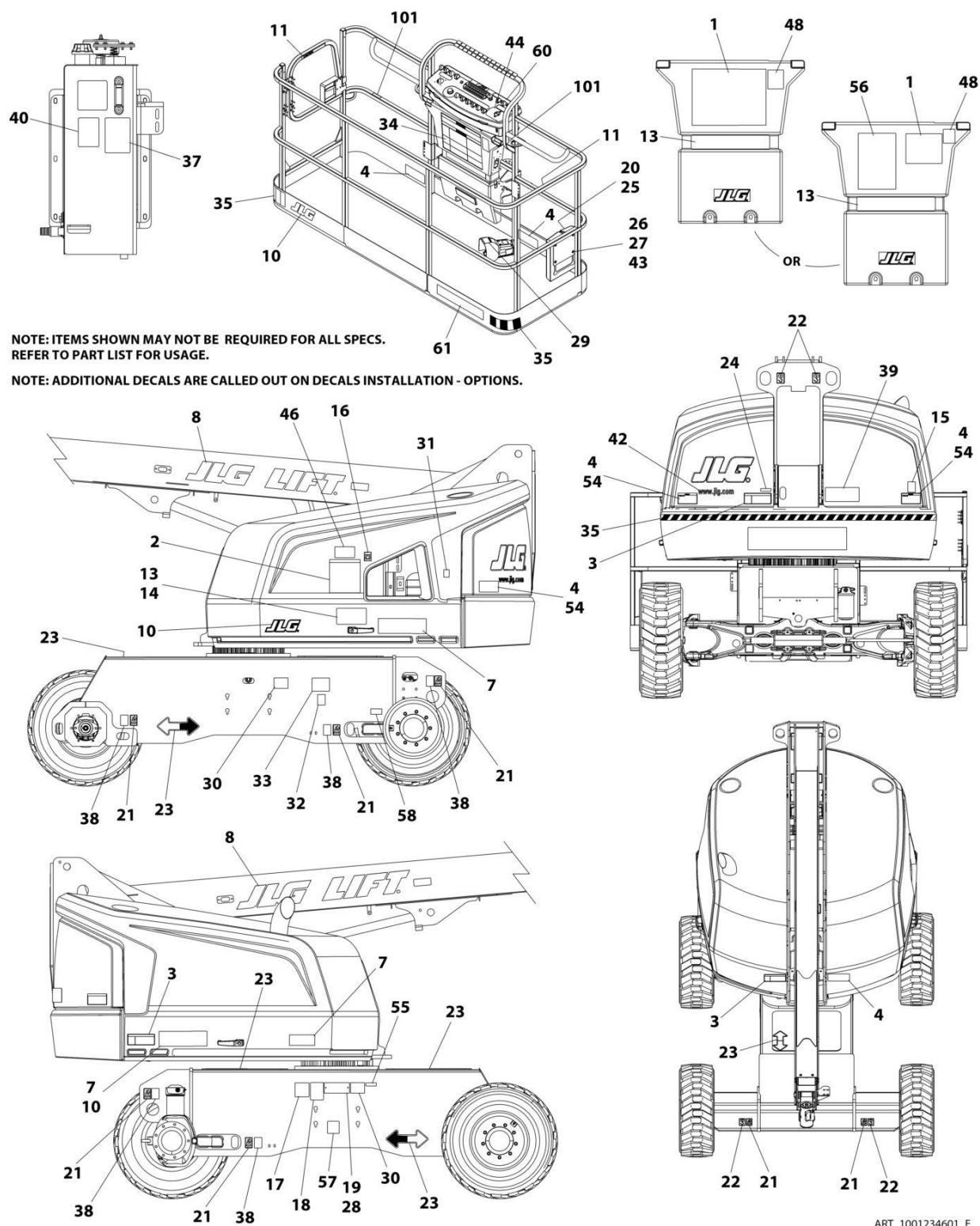
FIGURE 9-9. DECAL INSTALLATION - JAPANESE SPECS
