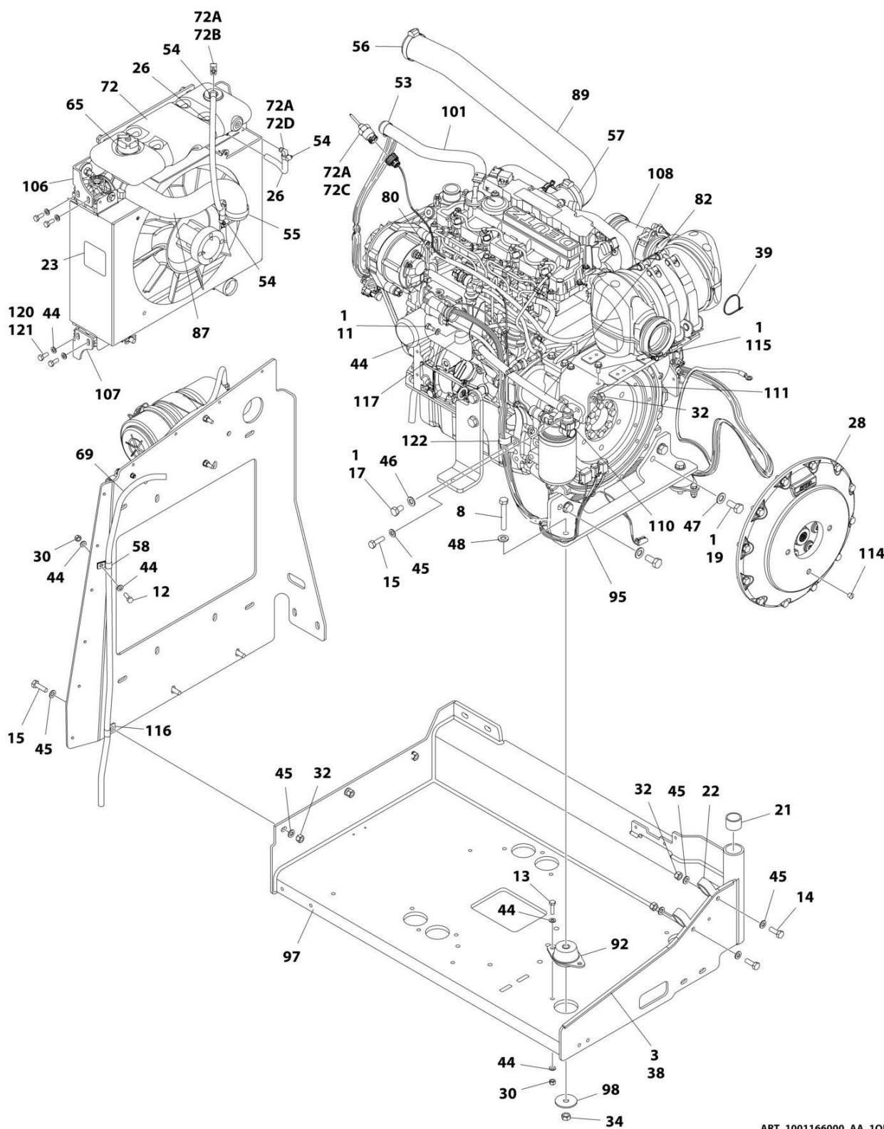
FIGURE 3-11. DEUTZ D2.9L4 ENGINE ASSEMBLY (WITHOUT ARCTIC PACKAGE)
