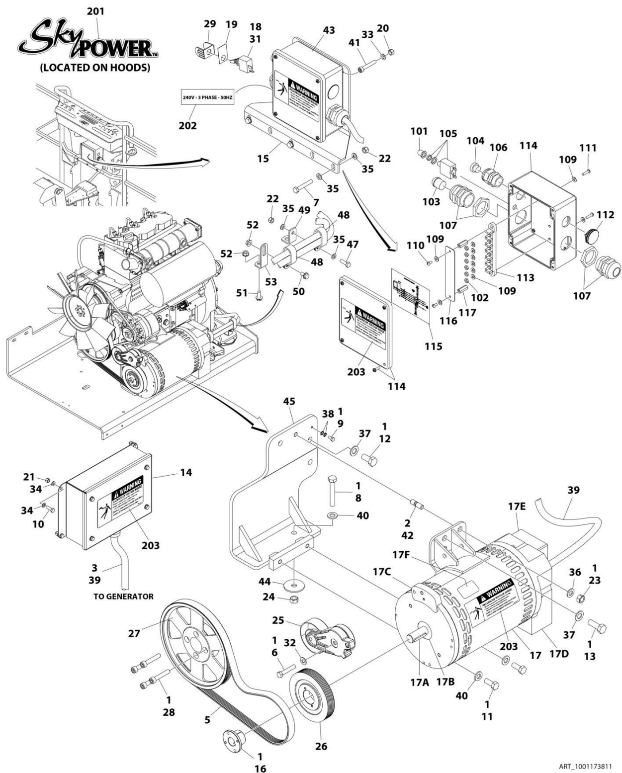
FIGURE 3-49. 7500W/50HZ SKYPOWER GENERATOR INSTALLATION - DEUTZ D2011 ENGINES
