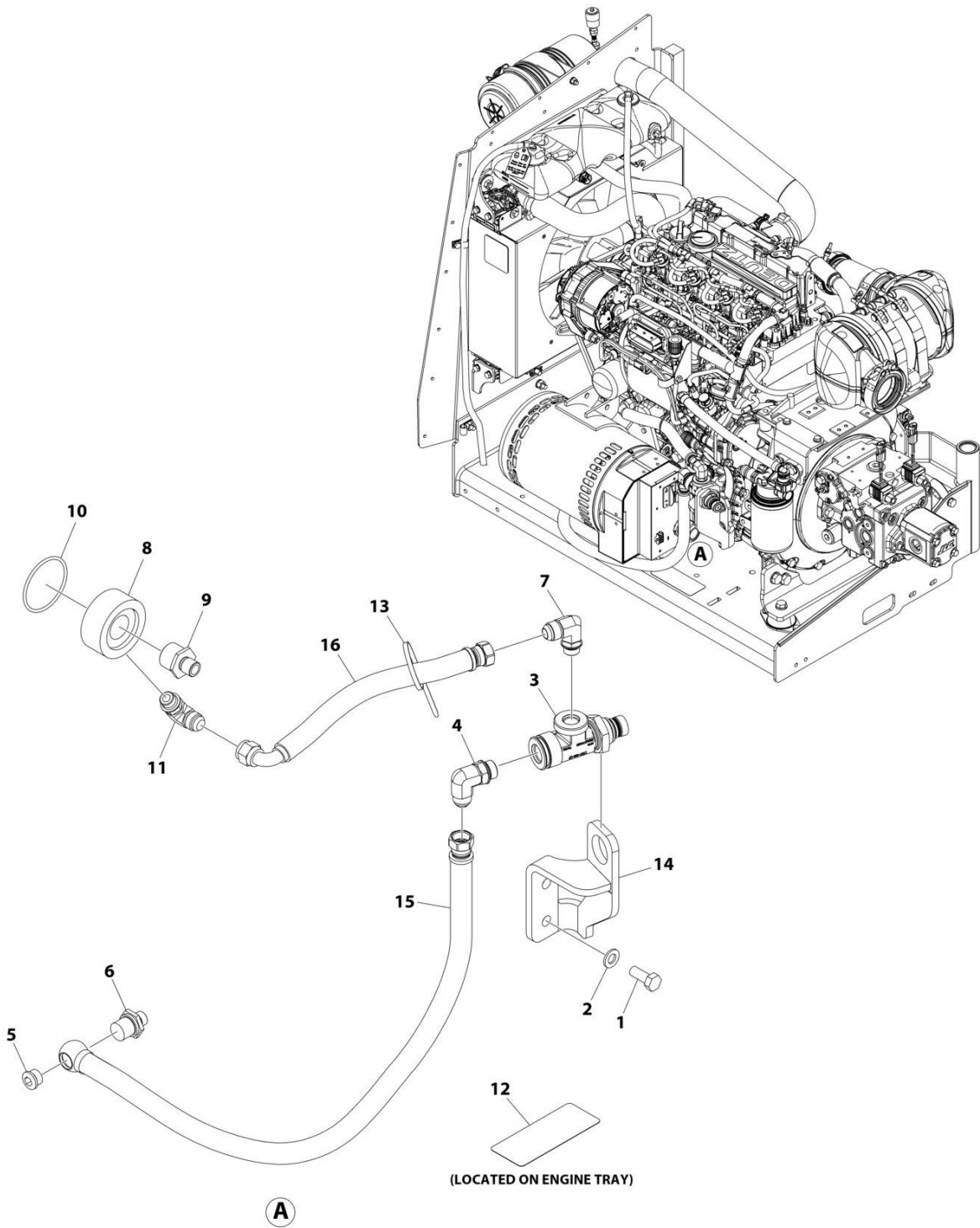
FIGURE 3-23. QUICKFIT OIL DRAIN INSTALLATION (DEUTZ D2.9L4 ENGINES)
