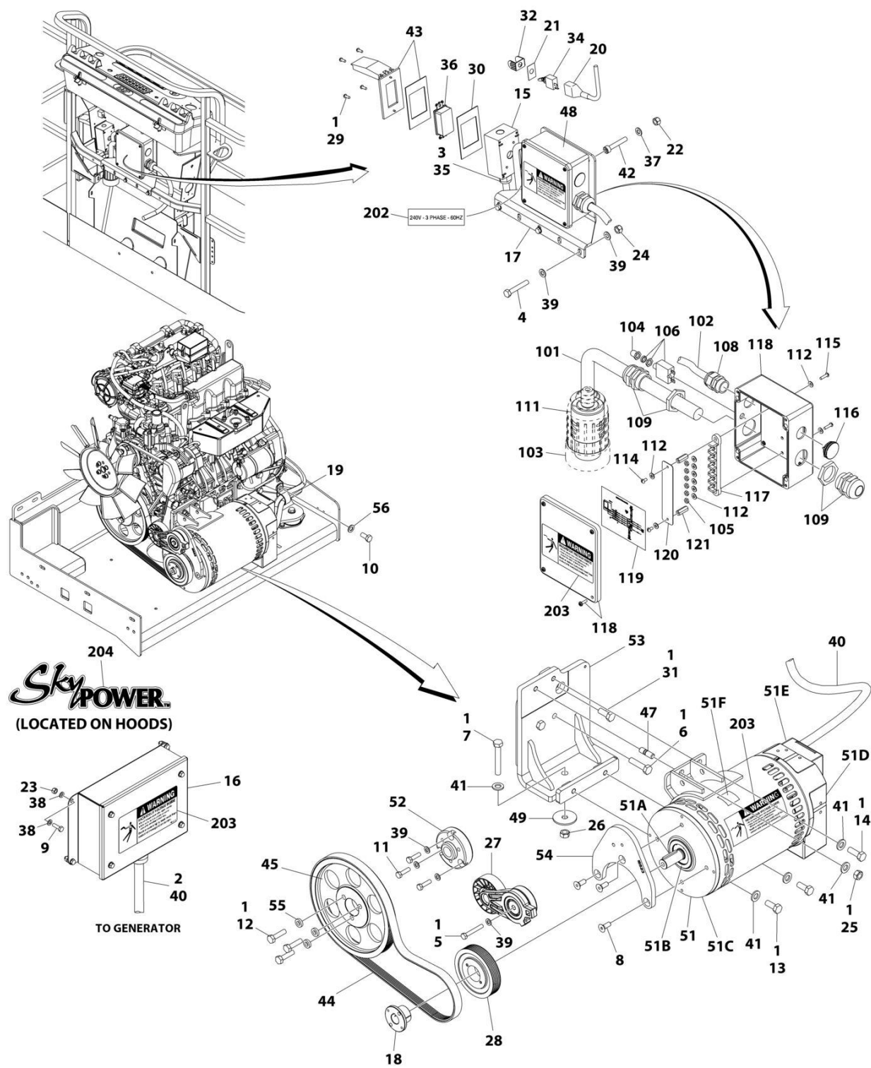
FIGURE 3-52. 7500W/60HZ SKYPOWER GENERATOR INSTALLATION - KUBOTA ENGINES
