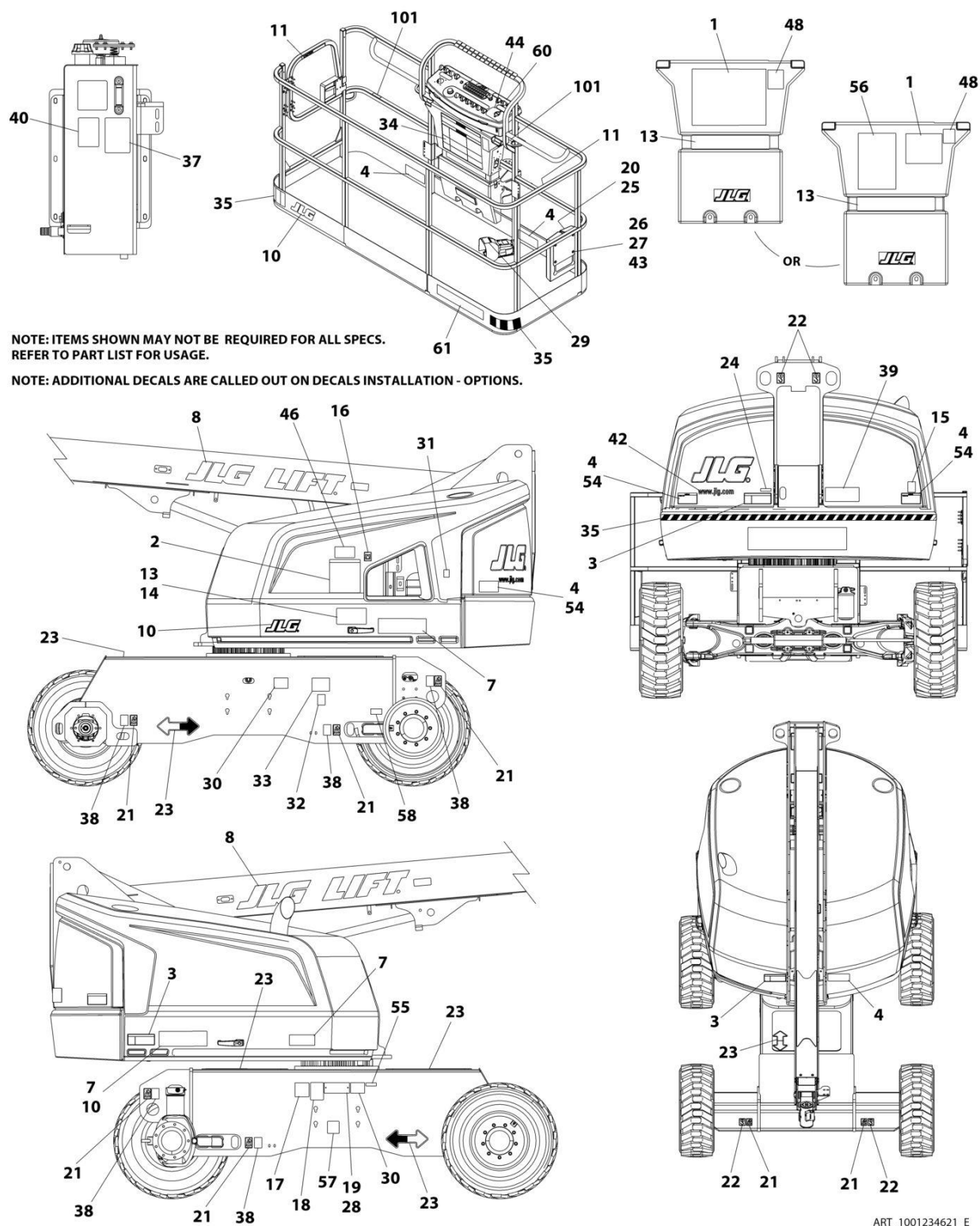
FIGURE 9-8. DECAL INSTALLATION - CSA SPECS (GAS MACHINES)
