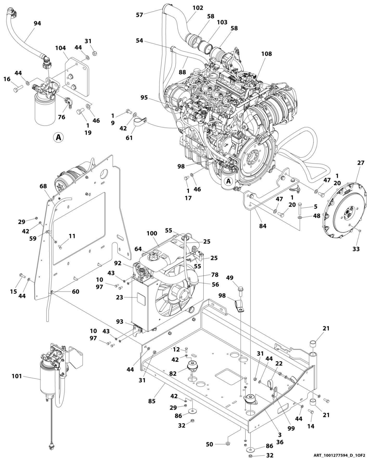
FIGURE 3-18. DEUTZ D2.9L4 (STAGE V) ENGINE ASSEMBLY
