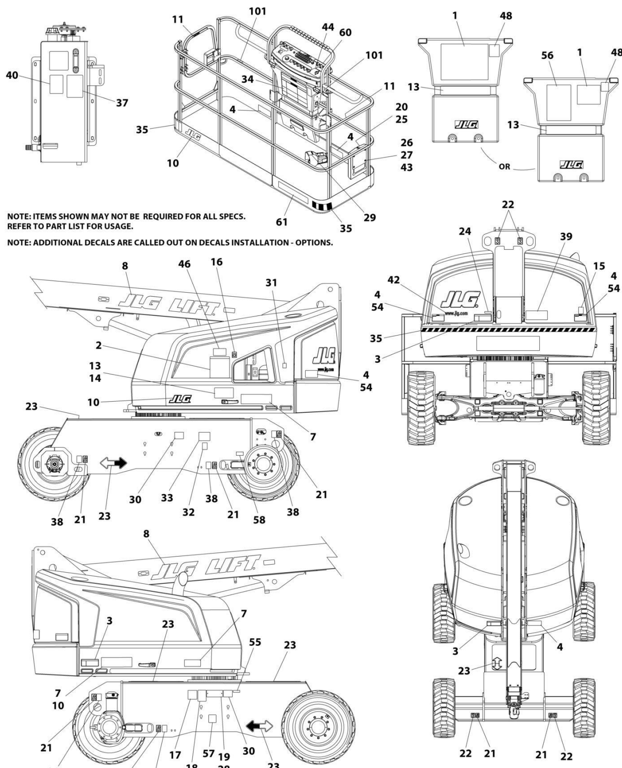
FIGURE 9-4. DECAL INSTALLATION - BRAZIL SPECS
