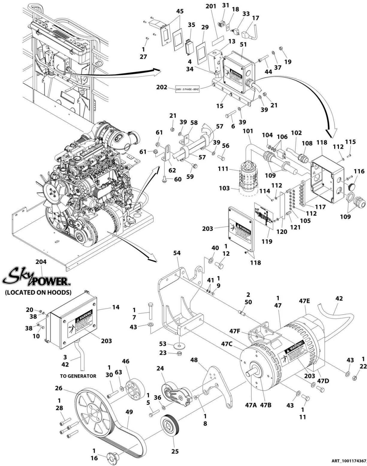
FIGURE 3-51. 7500W/60HZ SKYPOWER GENERATOR INSTALLATION - DEUTZ D2.9L4 ENGINES
