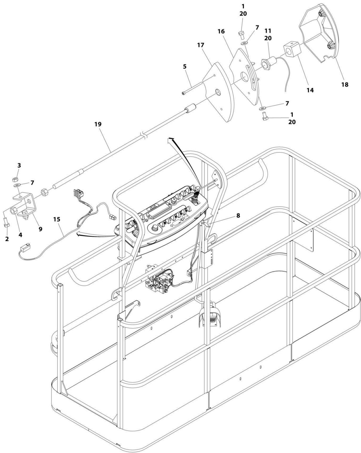
FIGURE 5-18. SKYLINE INSTALLATION
