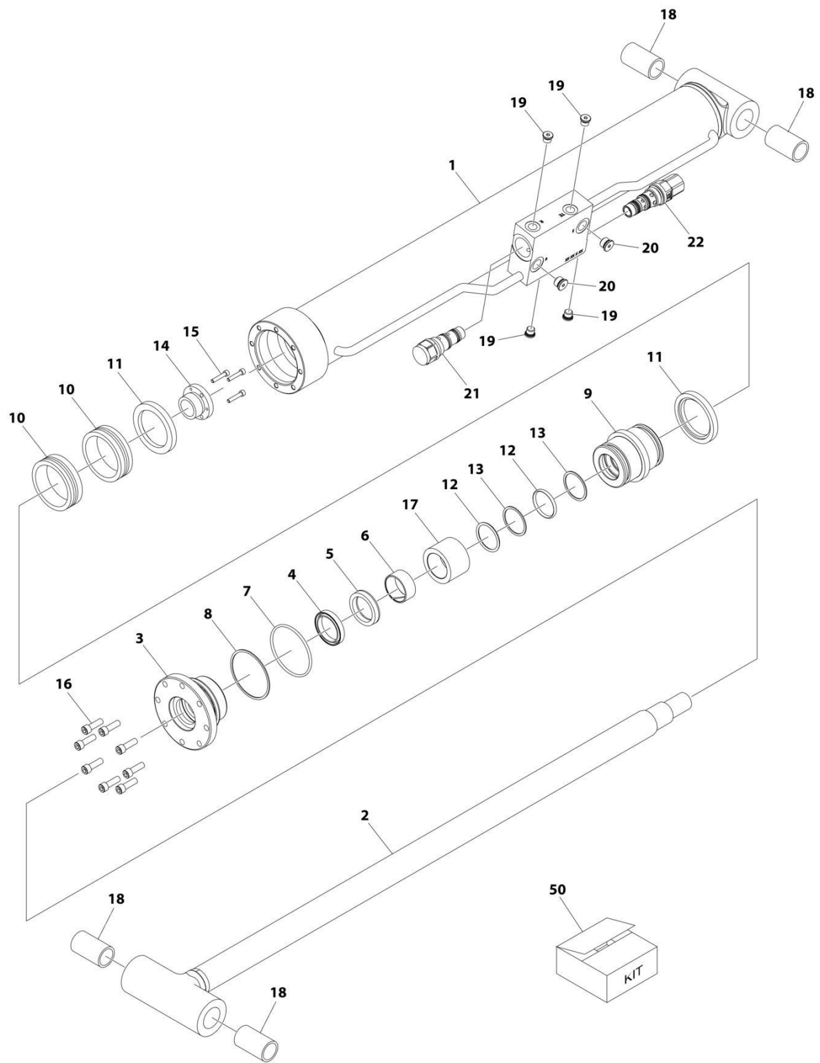
FIGURE 6-4. LIFT CYLINDER ASSEMBLY - JIB (460SJ HC3)
