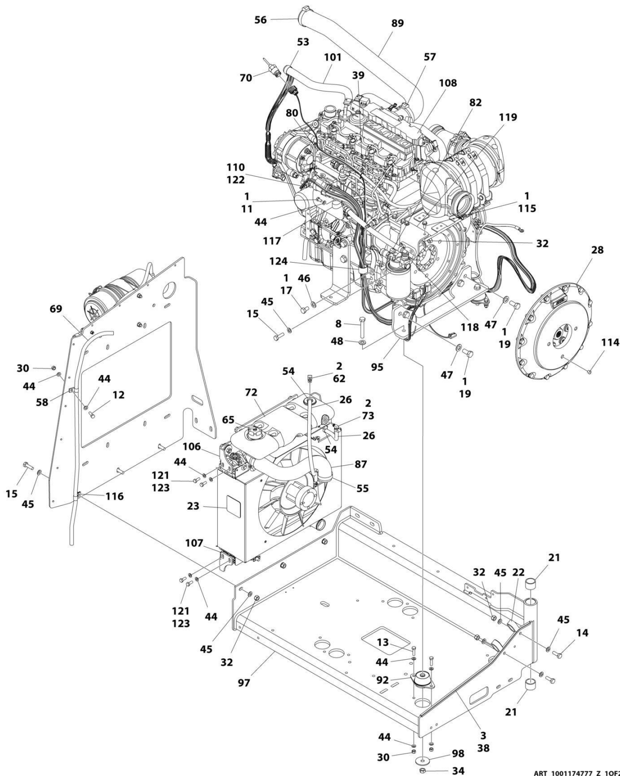
FIGURE 3-14. DEUTZ D2.9L4 ENGINE ASSEMBLY (WITH ARCTIC PACKAGE)
