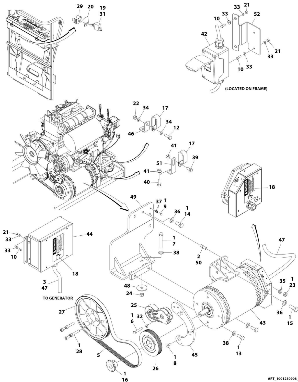
FIGURE 3-45. 4000W/50HZ GENERATOR INSTALLATION - DEUTZ D2011 ENGINES
