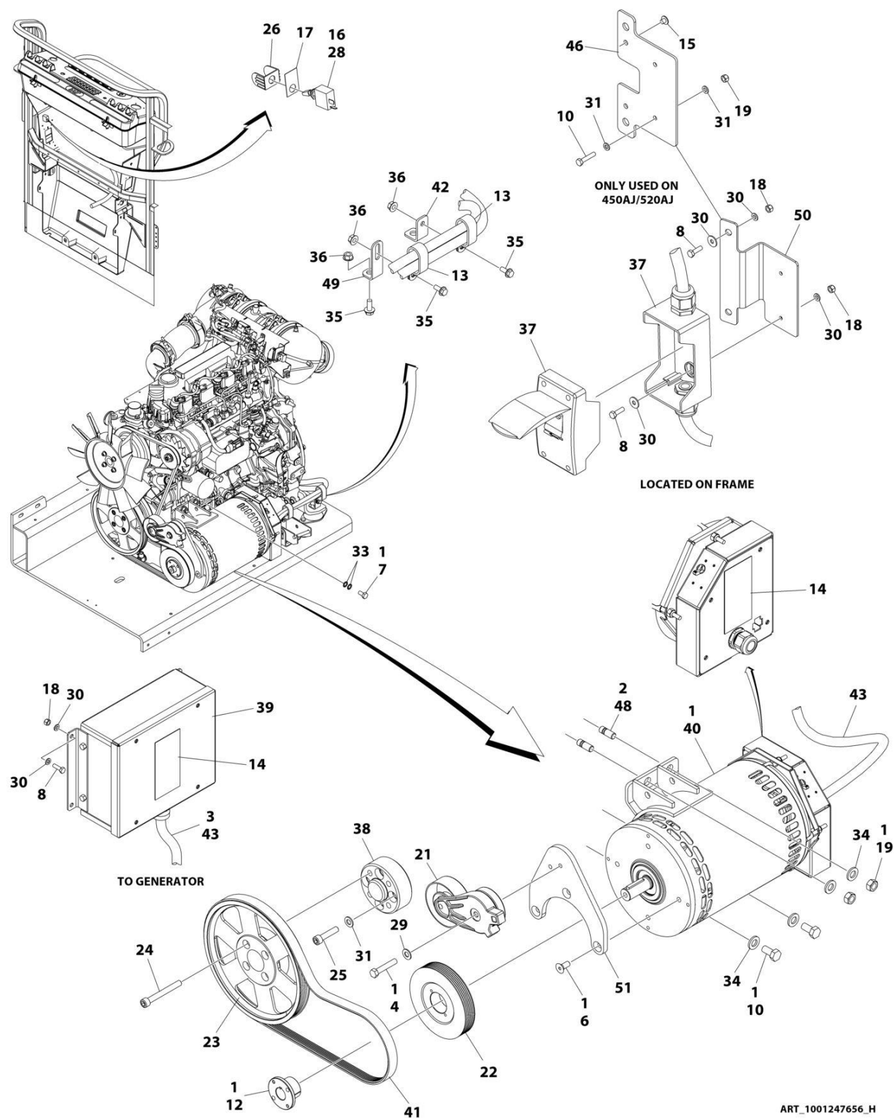
FIGURE 3-48. 4000W/50HZ GENERATOR INSTALLATION (DEUTZ D2.9L4 (STAGE V) ENGINES)
