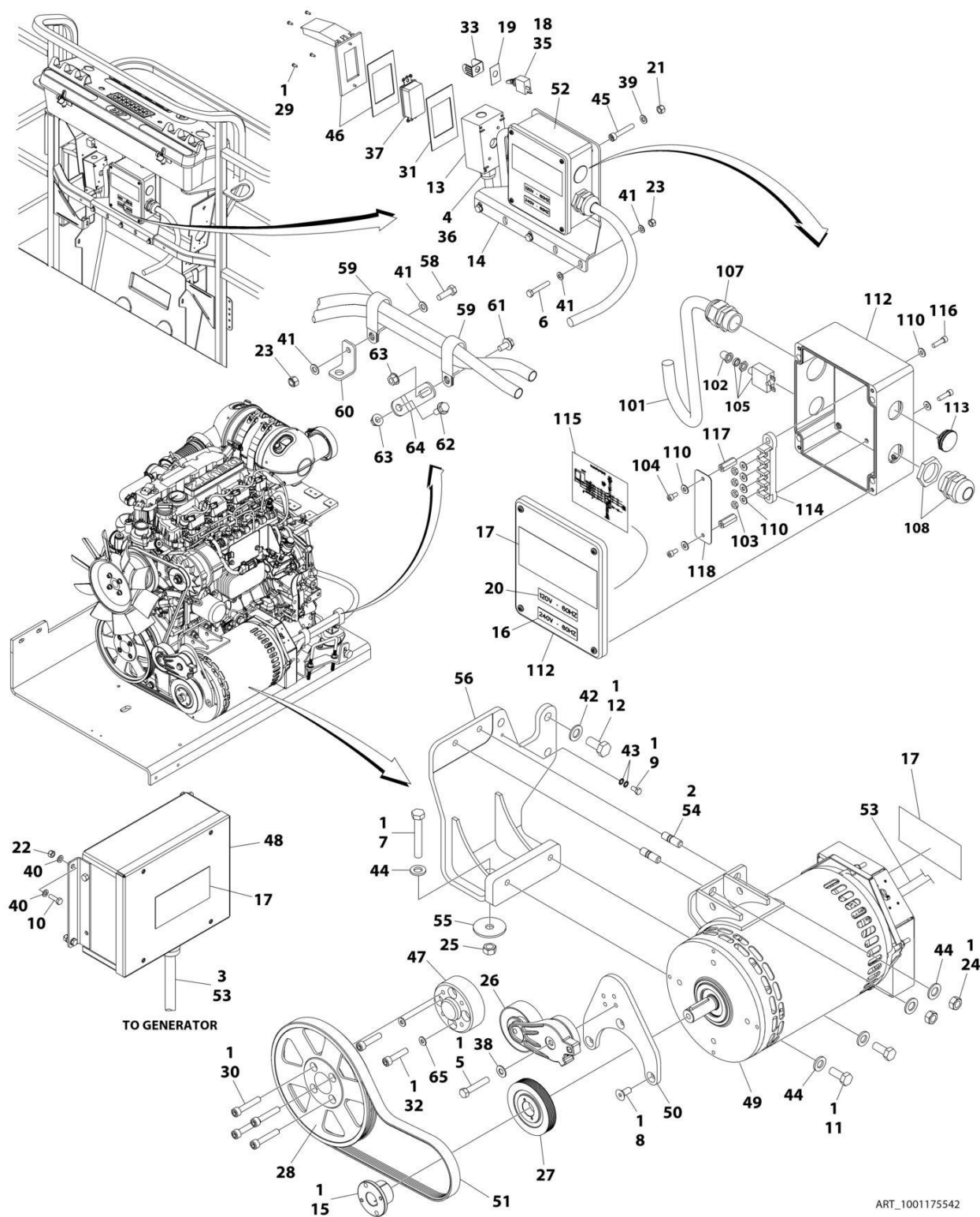
FIGURE 3-47. 4000W/60HZ GENERATOR INSTALLATION - DEUTZ D2.9L4 ENGINES
