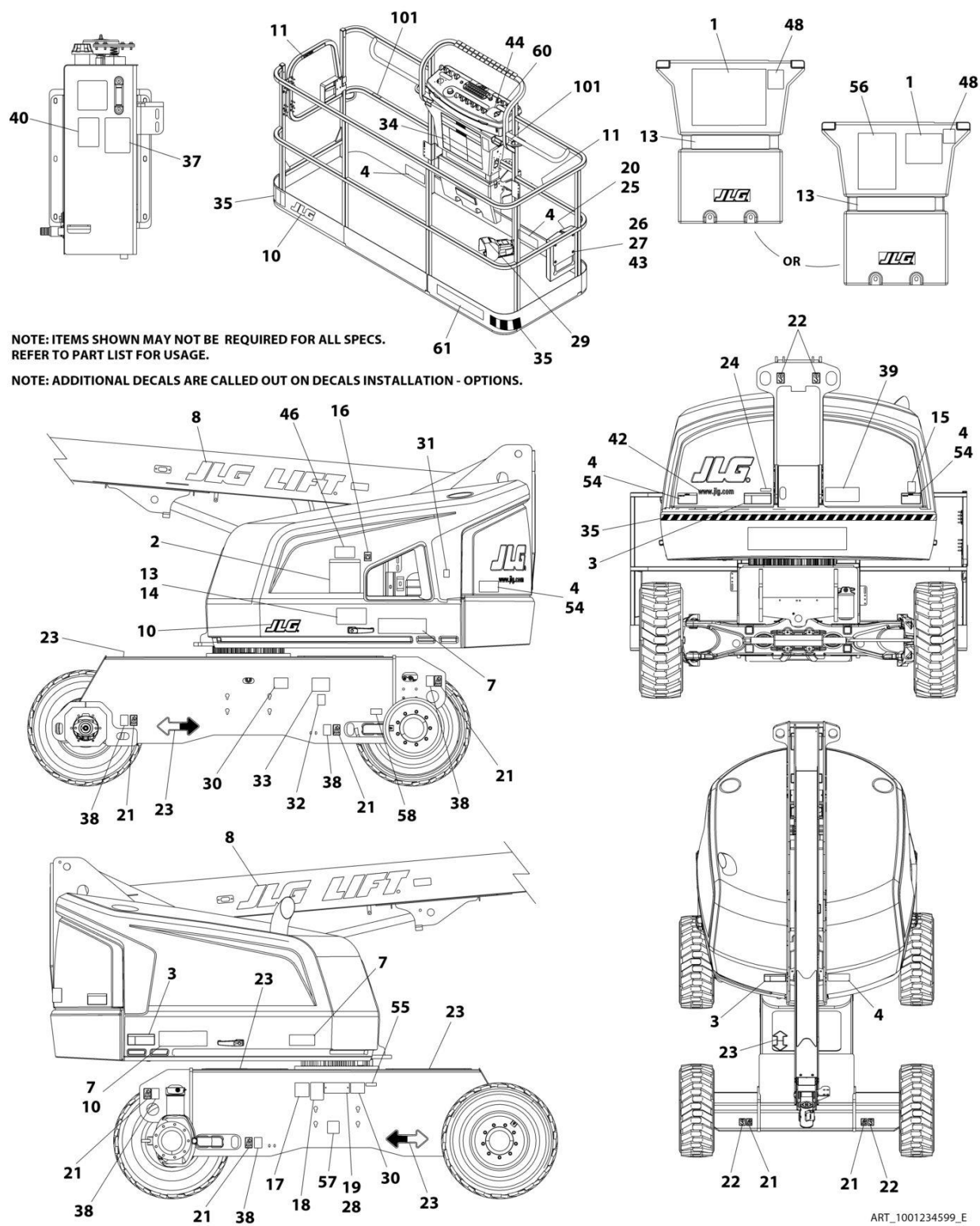
FIGURE 9-1. DECAL INSTALLATION - ANSI SPECS (DIESEL MACHINES)
