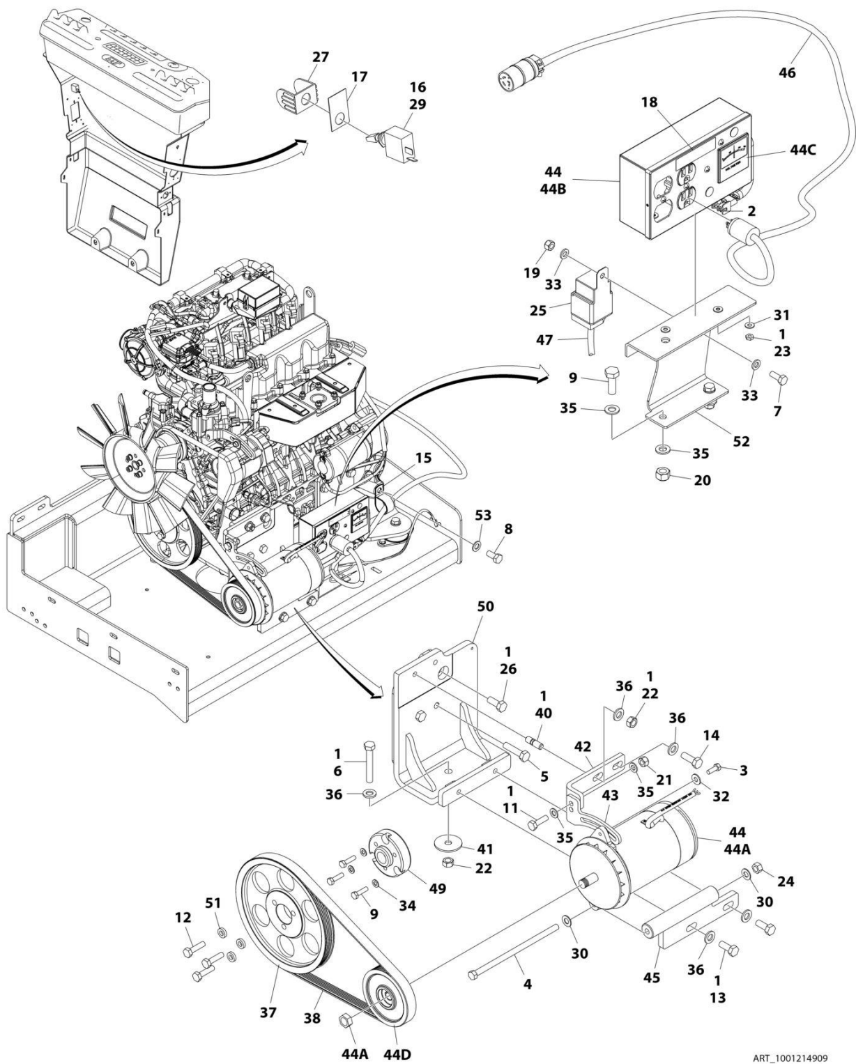
FIGURE 3-44. 2500W/110V/60HZ GENERATOR INSTALLATION - KUBOTA ENGINES
