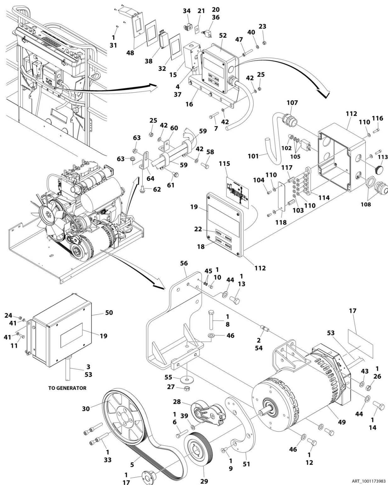
FIGURE 3-46. 4000W/60HZ GENERATOR INSTALLATION - DEUTZ D2011 ENGINES
