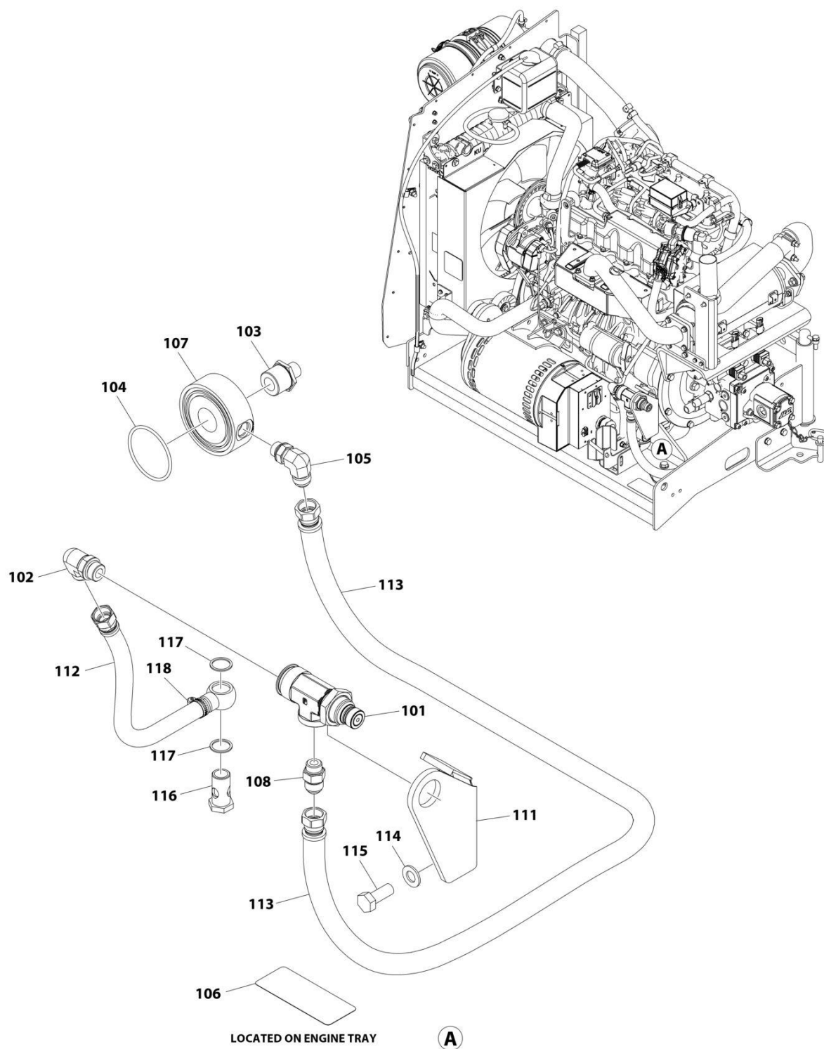
FIGURE 3-1. QUICKFIT OIL DRAIN INSTALLATION (KUBOTA) (SN 03000305081 to Present, Including , Excluding 0300305086 and 0300305088)
