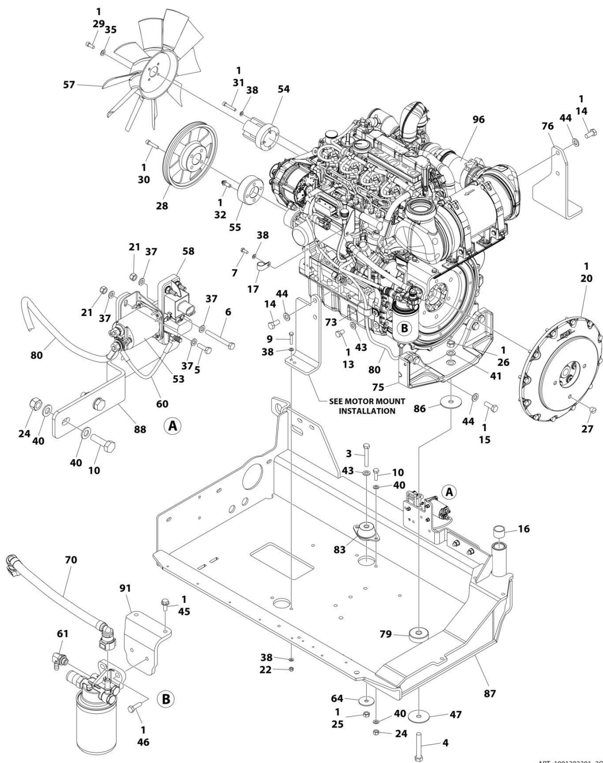
FIGURE 3-17. DEUTZ TD2.9L4 EMR5 ENGINE ASSEMBLY
