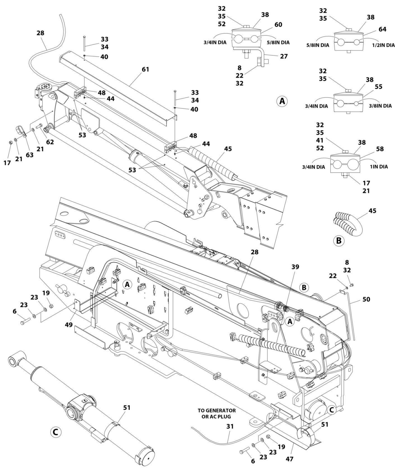
FIGURE 8-27. AC CABLES AND CLAMPS INSTALLATION - WITH 4000W/50HZ GENERATOR (ANSI EXPORT, AUSTRALIAN AND CE SPECS) (SN 0300292972 to Present)
