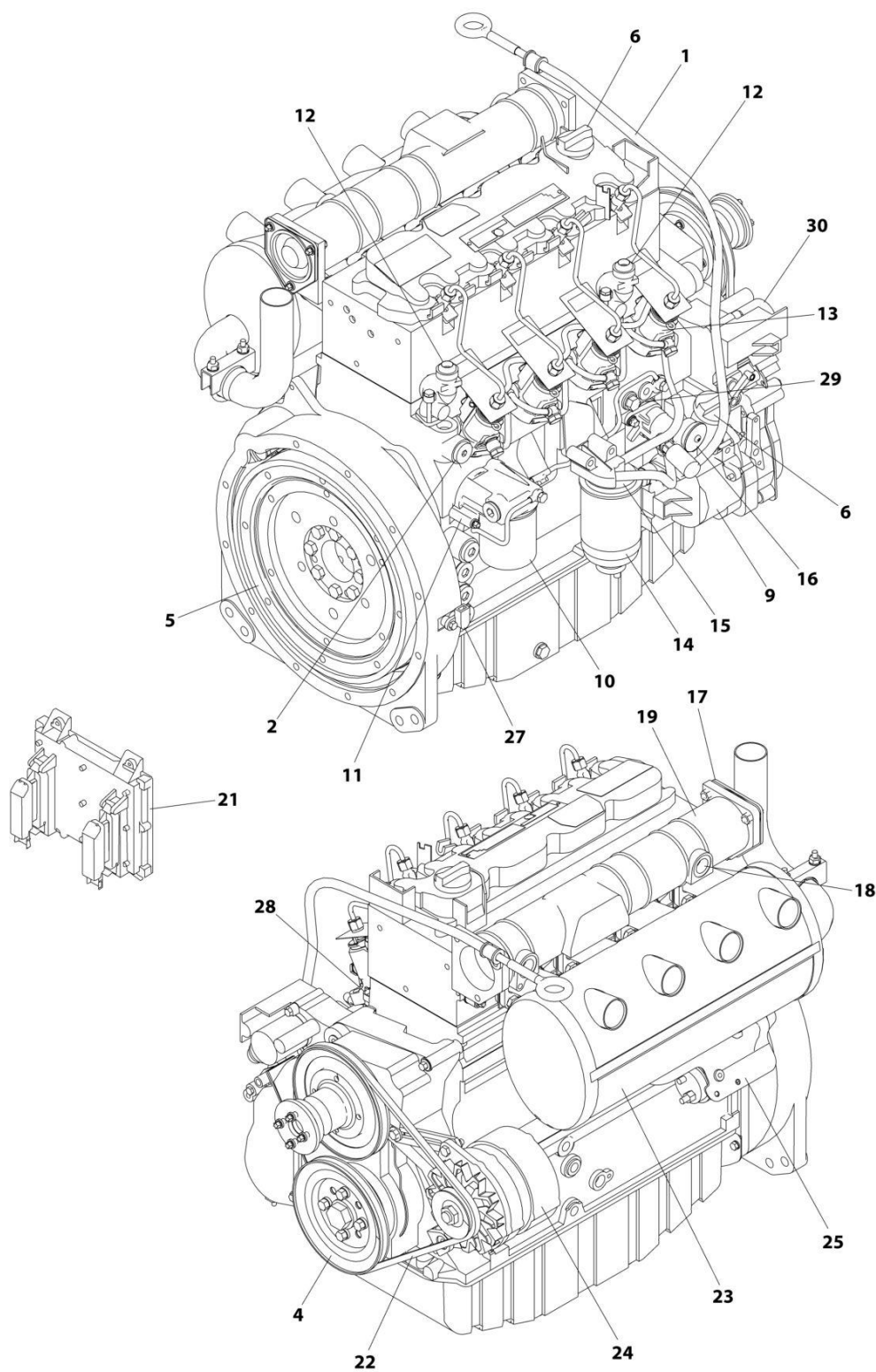
FIGURE 3-4. DEUTZ D2011 ENGINE COMPONENTS
