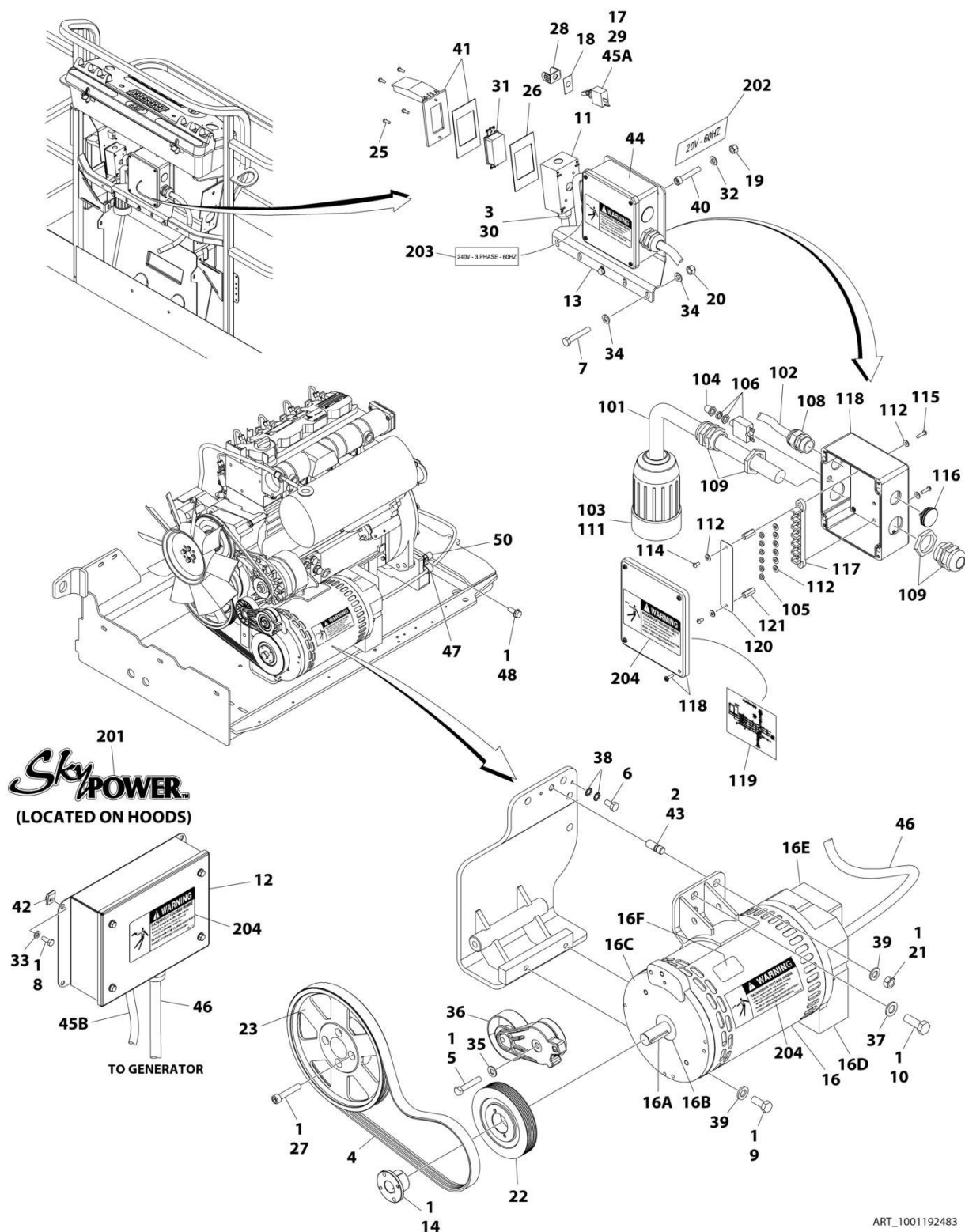
FIGURE 3-45. 7500W SKYPOWER GENERATOR INSTALLATION - 110/60HZ (DEUTZ D2011 ENGINES) (OPTIONAL)
