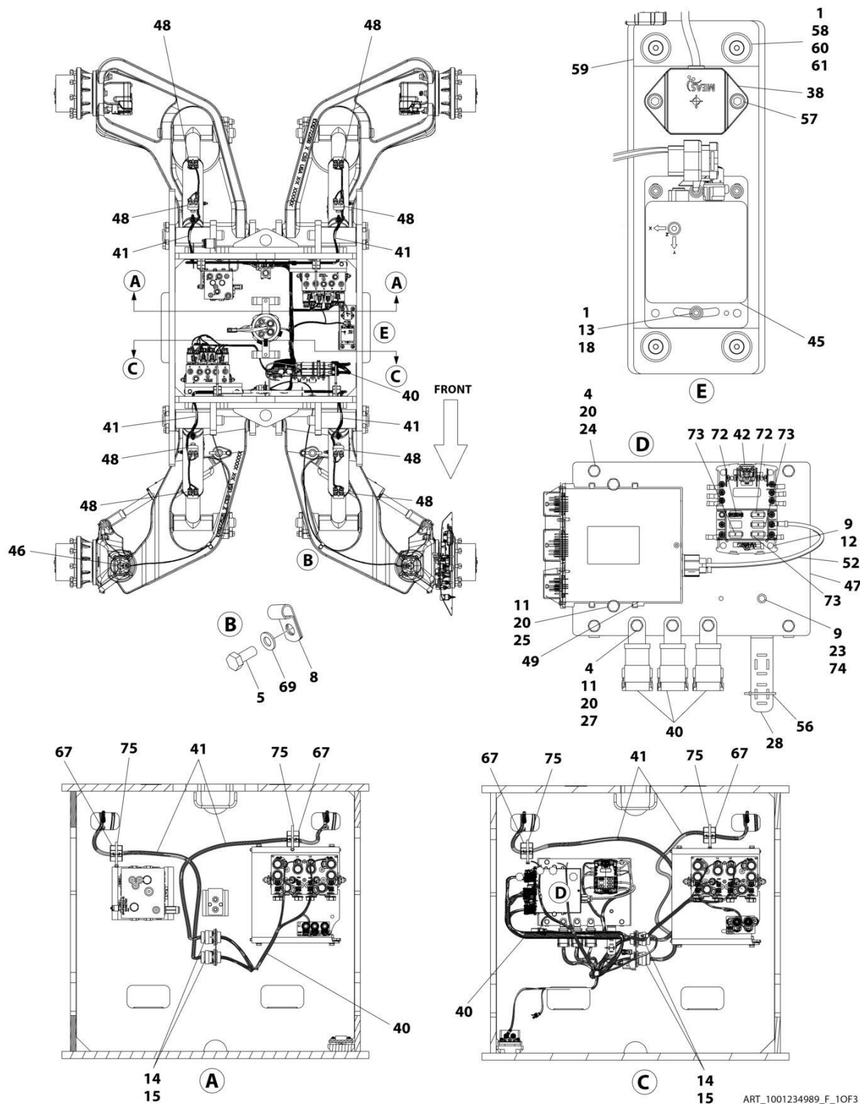
FIGURE 8-3. ELECTRICAL INSTALLATION (DEUTZ D2011 & DEUTZ DT2.9L4 ENGINES) (SN 0300311240 to Present)
