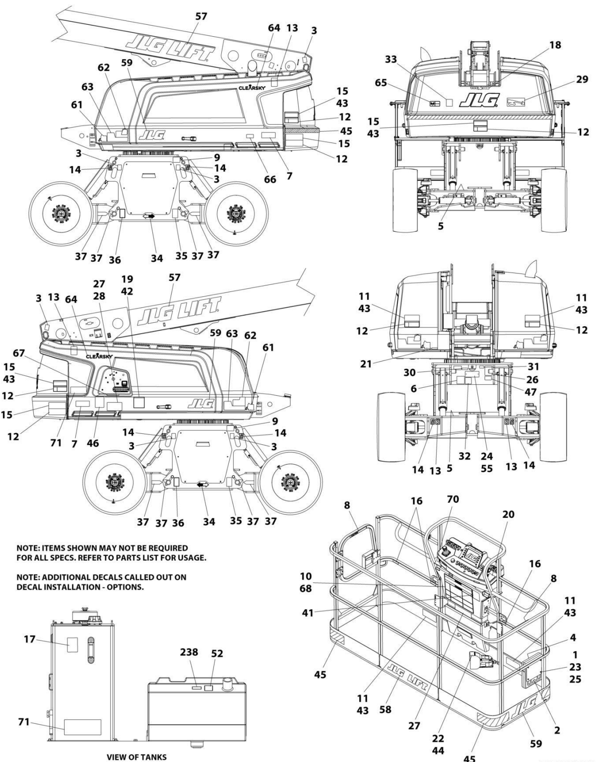
FIGURE 9-10. DECAL INSTALLATION (CE SPECS - ENGLISH LANGUAGE)
