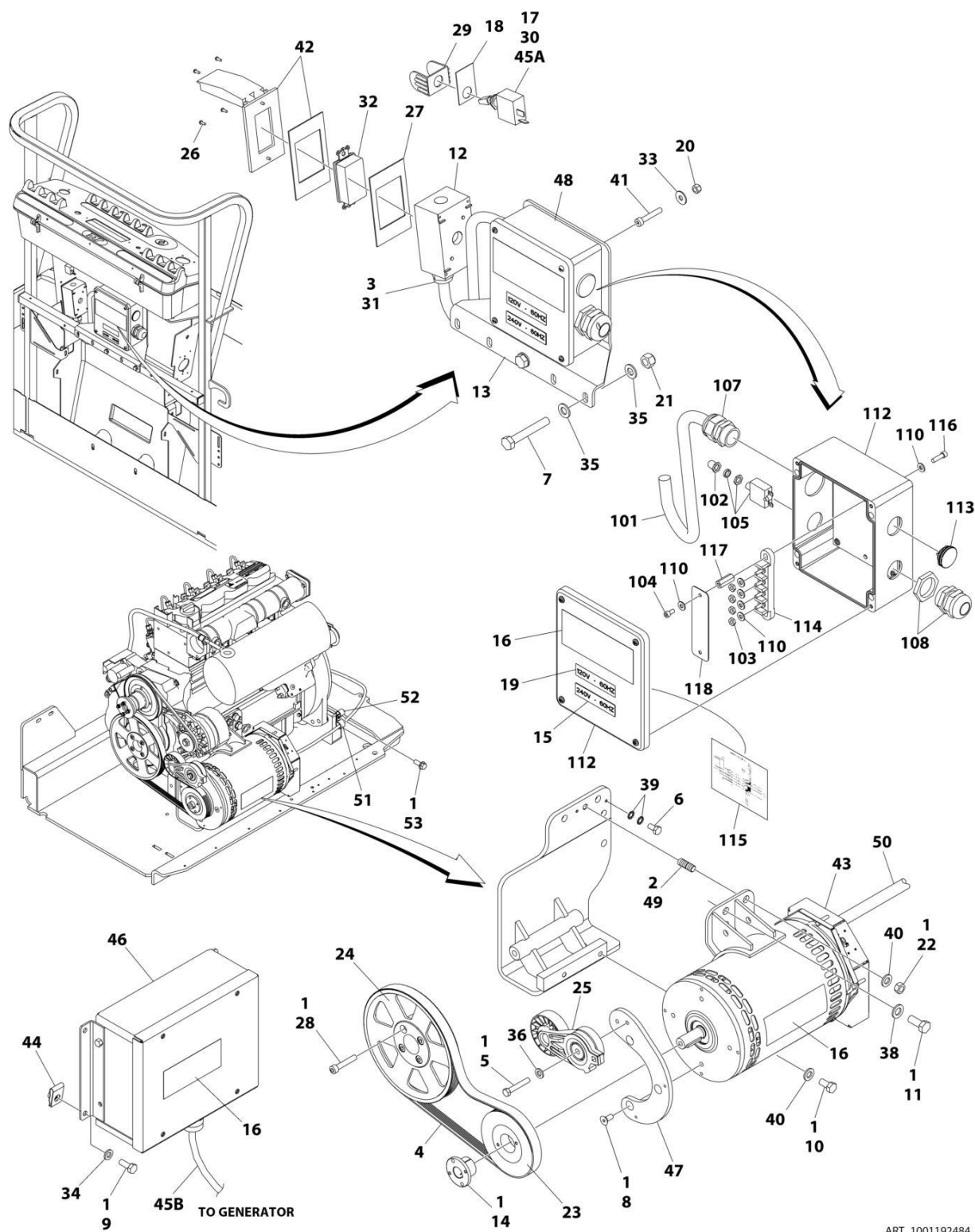
FIGURE 3-41. 4000W GENERATOR INSTALLATION - 110V/60HZ (DEUTZ D2011 ENGINES) (OPTIONAL)
