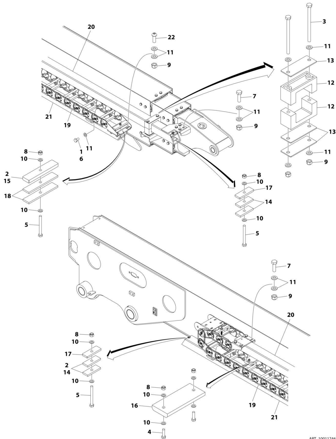
FIGURE 4-7. POWER TRACK INSTALLATION
