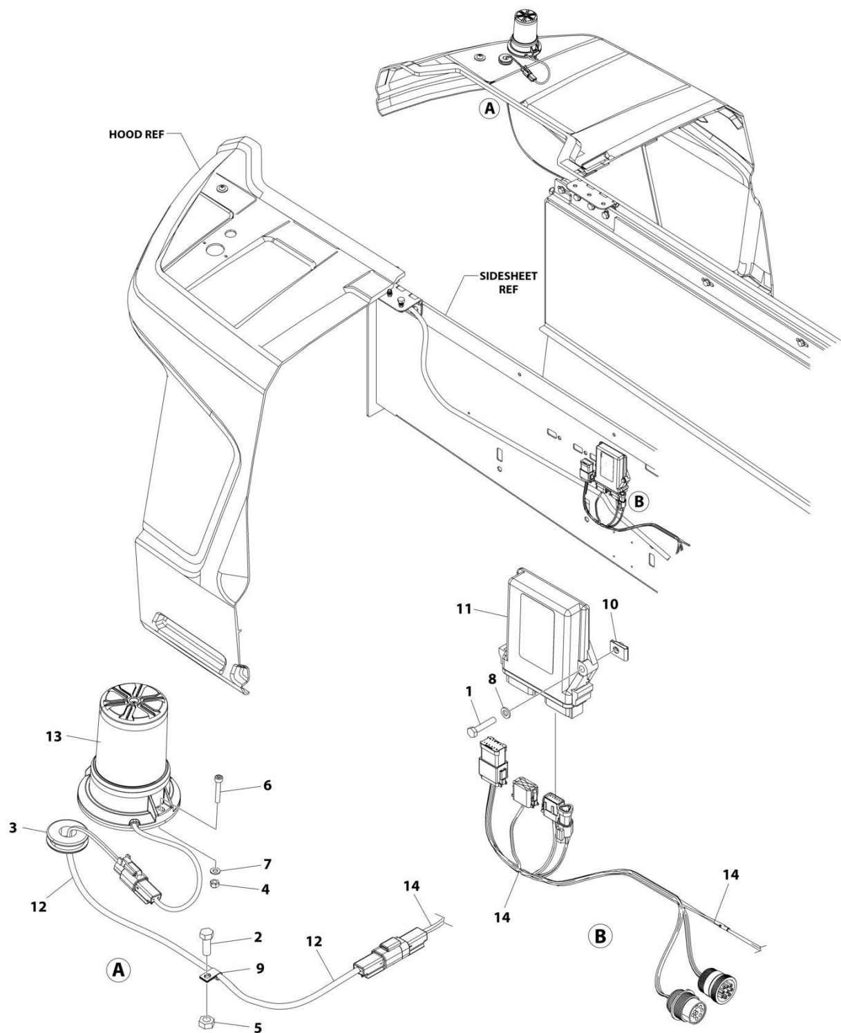
FIGURE 2-22. STROBE LIGHT INSTALLATION - RED (OPTIONAL)
