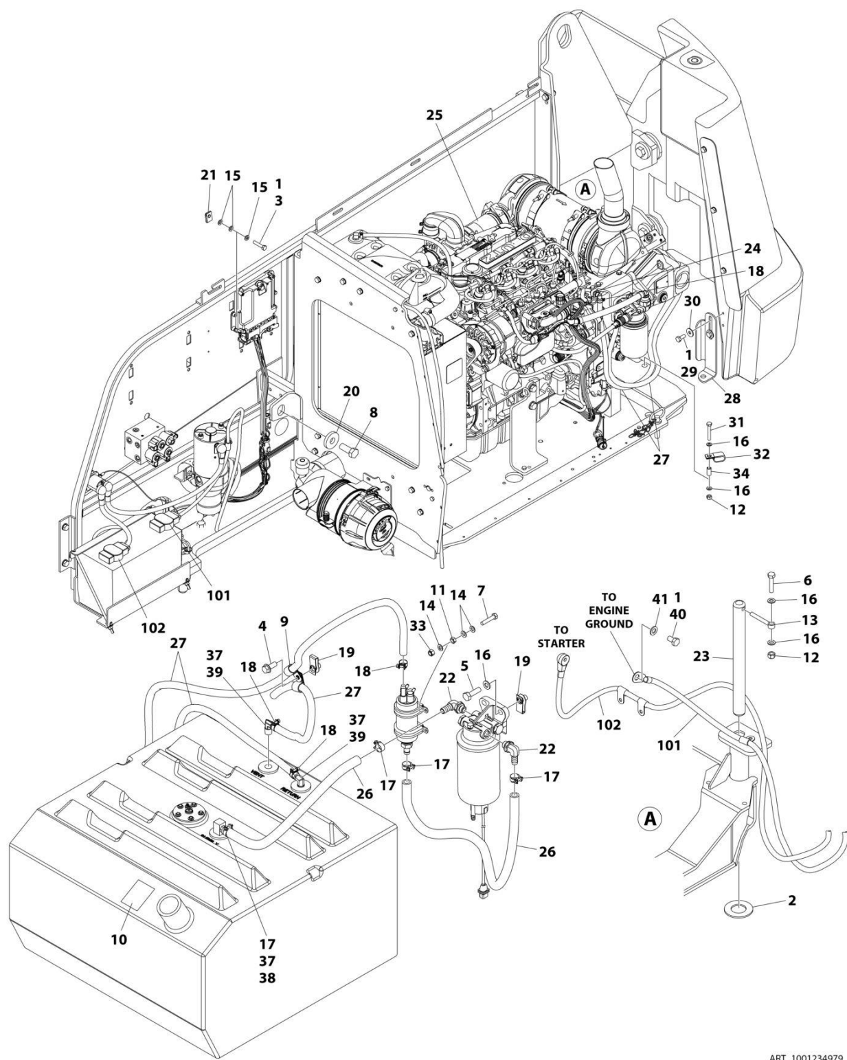
FIGURE 3-9. DEUTZ TD2.9L4 EMR4 ENGINE INSTALLATION
