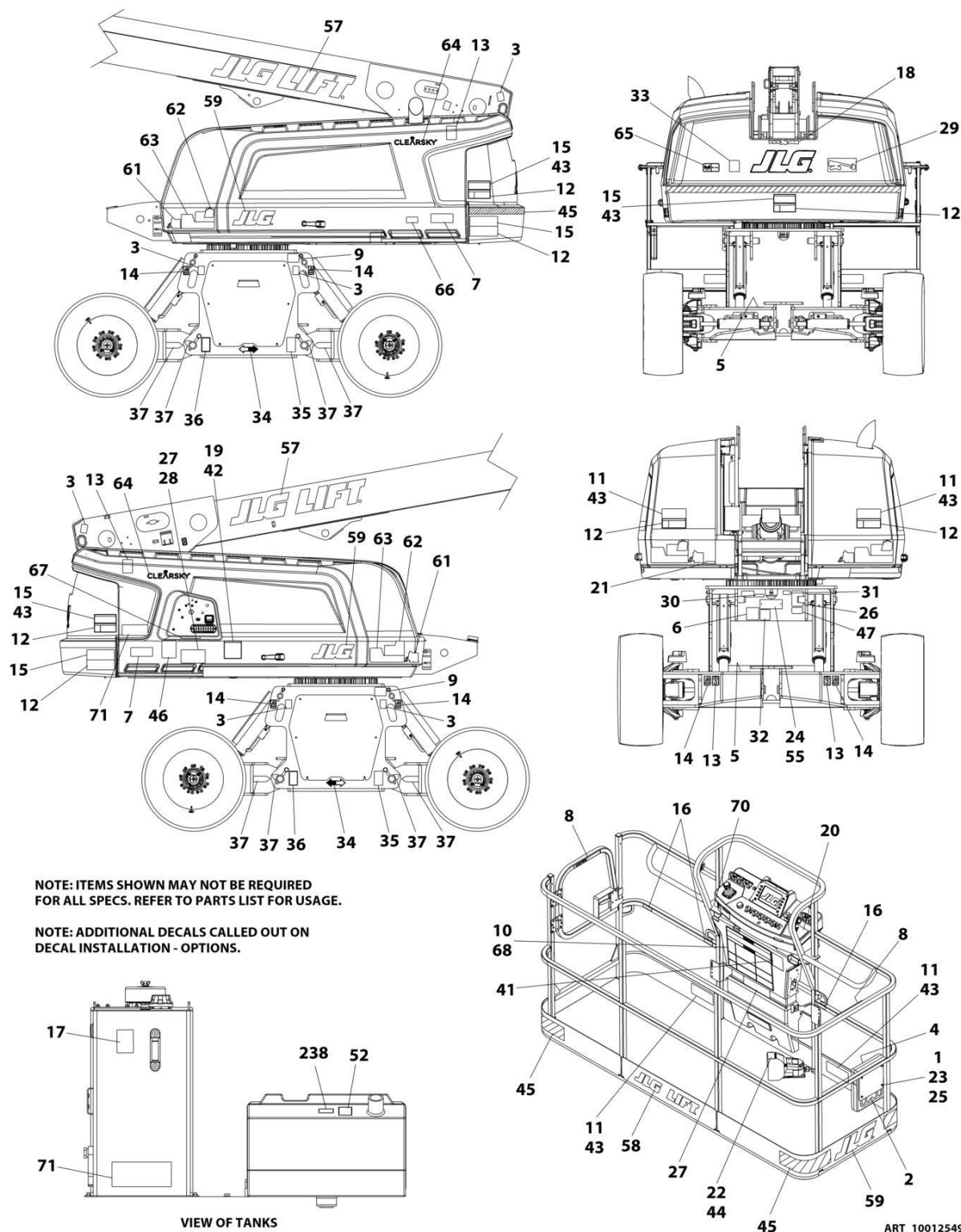
FIGURE 9-8. DECAL INSTALLATION (LATIN AMERICAN SPECS - SPANISH/ENGLISH LANGUAGES)
