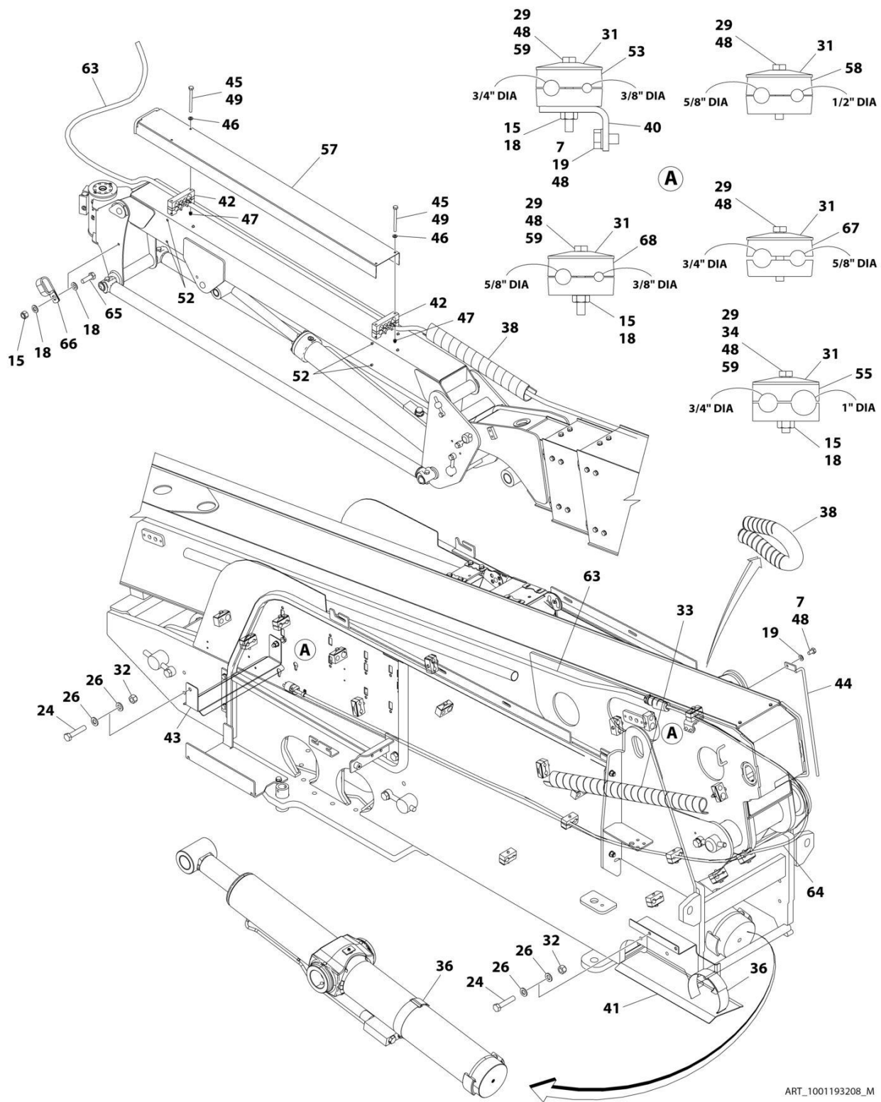
FIGURE 8-22. AC CABLES AND CLAMPS INSTALLATION - WITHOUT GENERATOR (ANSI, CSA AND JAPANESE SPECS) (Prior to SN 0300292972)
