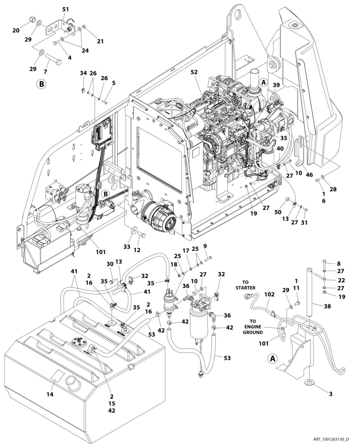
FIGURE 3-5. DEUTZ TD2.2L3 (STAGE V) ENGINE INSTALLATION
