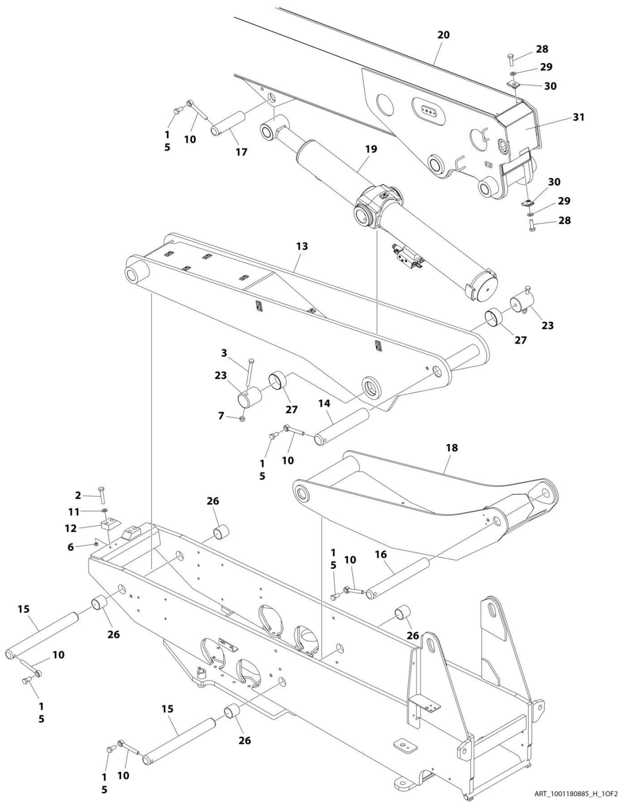
FIGURE 4-1. BOOM INSTALLATION
