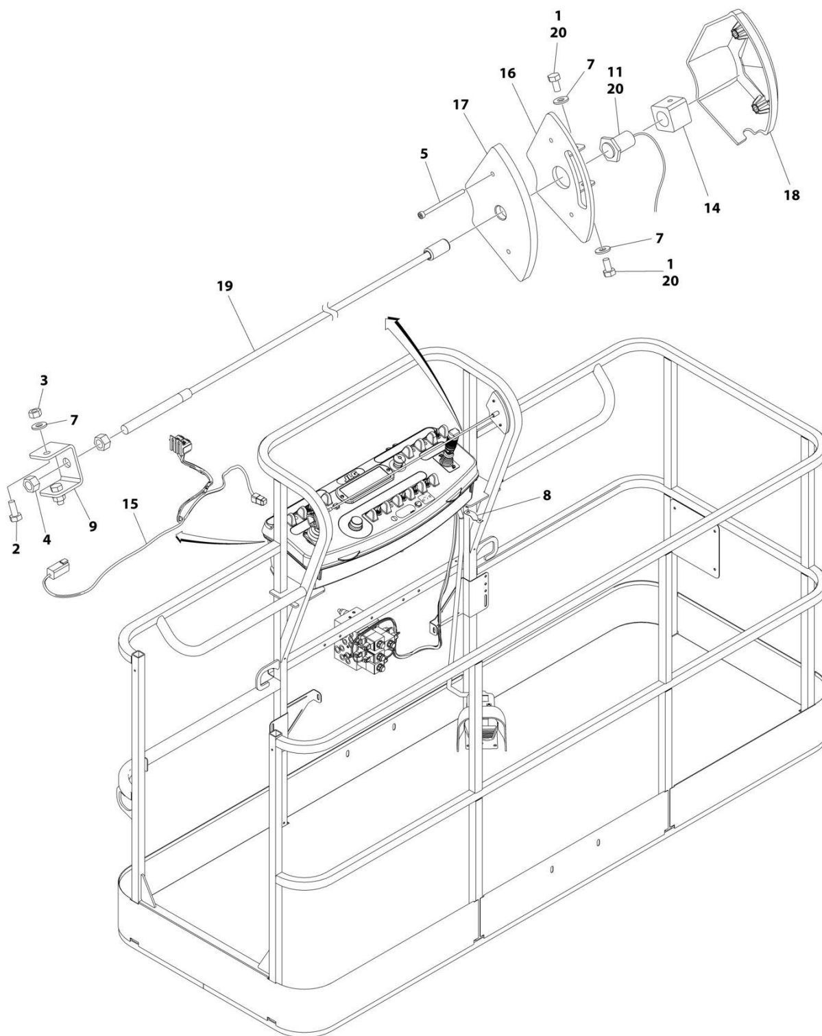
FIGURE 5-24. SKYLINE INSTALLATION
