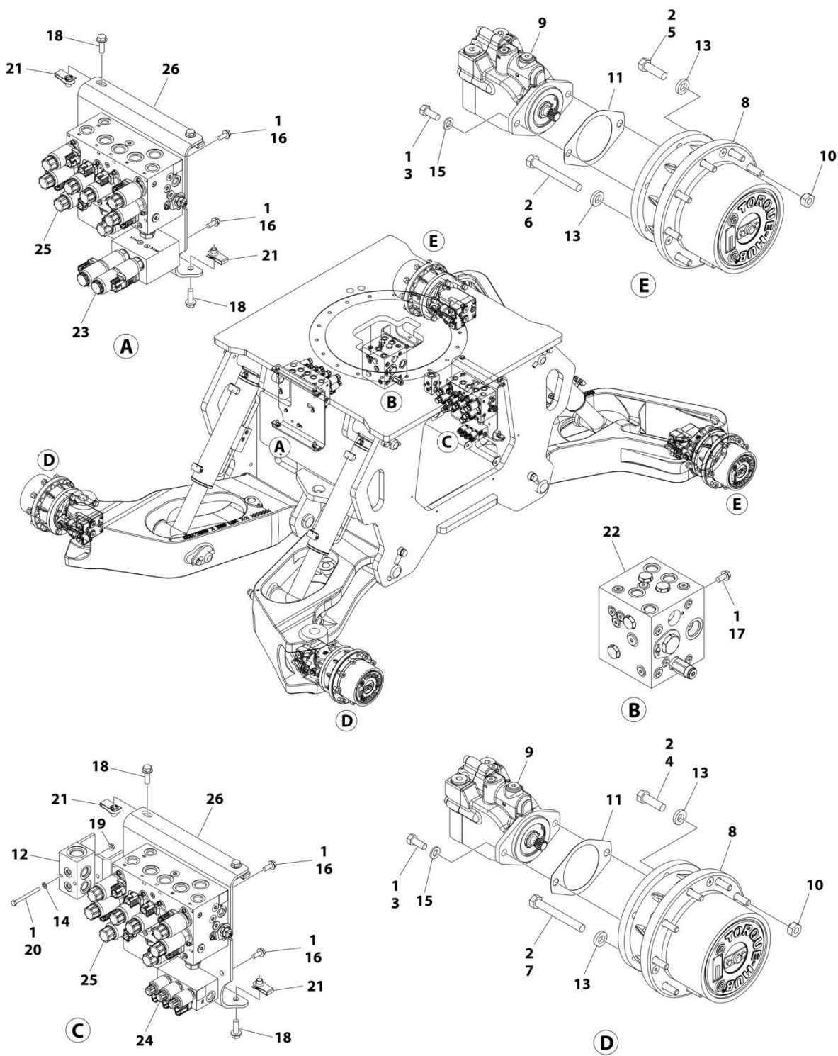
FIGURE 1-3. WHEEL DRIVE INSTALLATION
