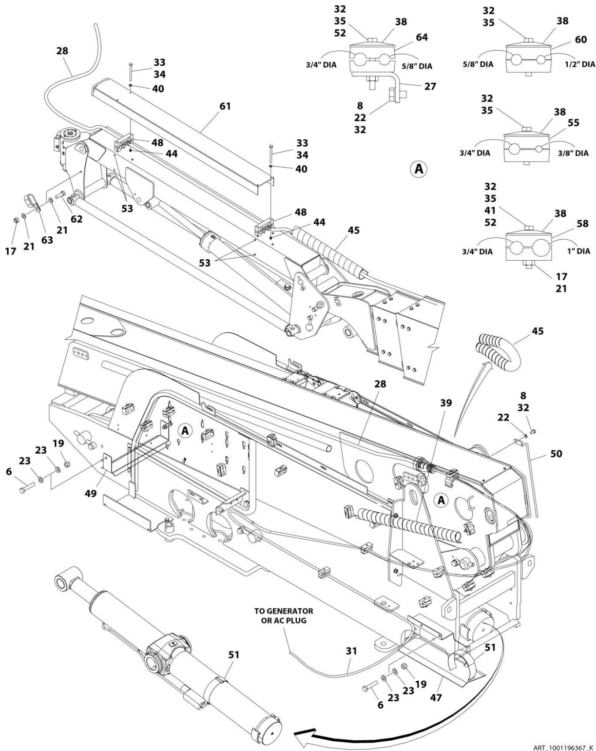
FIGURE 8-25. AC CABLES AND CLAMPS INSTALLATION - WITH 2500W GENERATOR (ALL SPECS EXCEPT AUSTRALIAN & CE SPECS)
