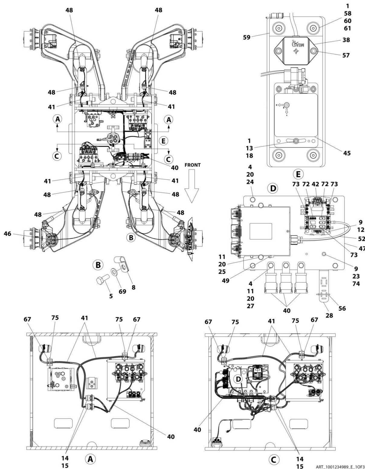
FIGURE 8-2. ELECTRICAL INSTALLATION (DEUTZ D2011 & DEUTZ DT2.9L4 ENGINES) (Prior to SN 0300311240)
