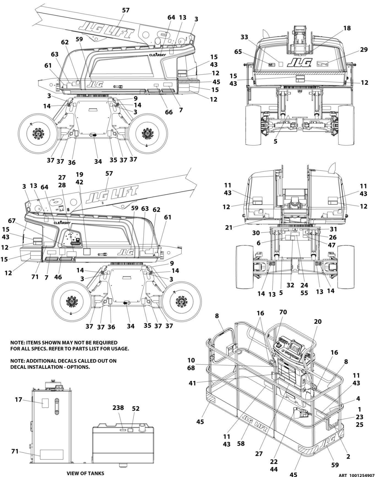
FIGURE 9-7. DECAL INSTALLATION (KOREAN SPECS - KOREAN/ENGLISH LANGUAGES)
