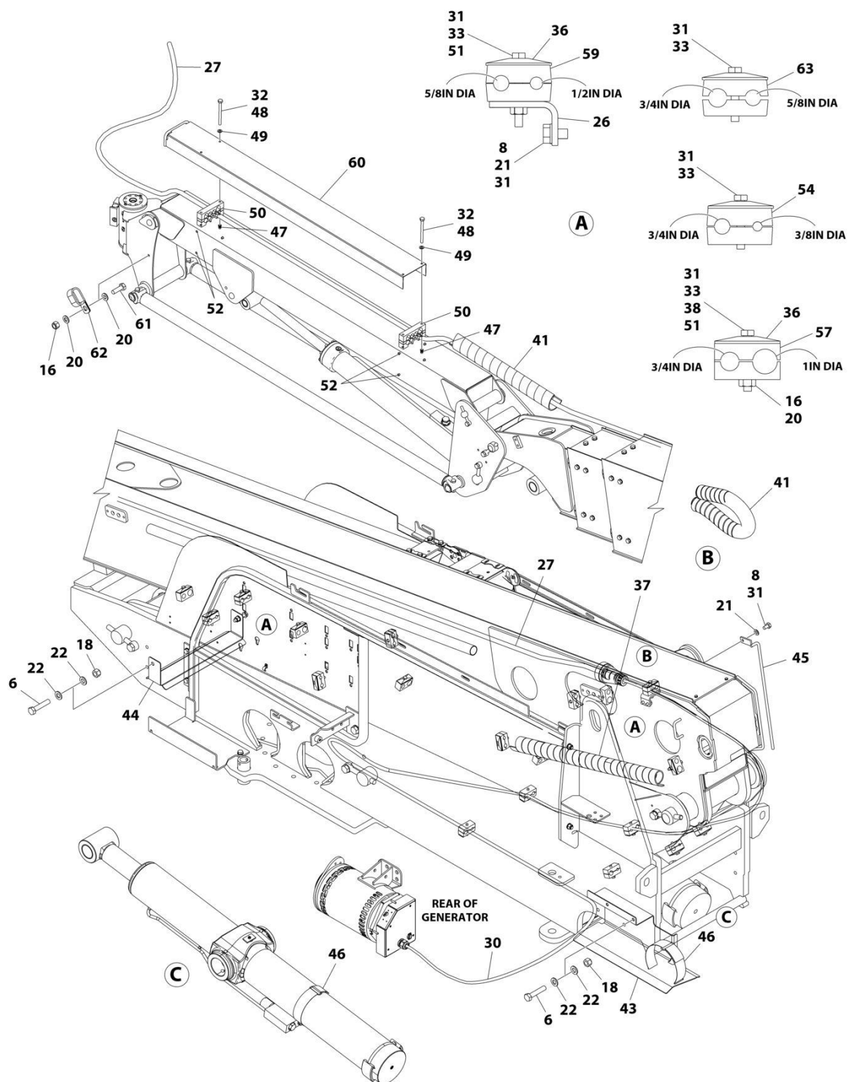
FIGURE 8-29. AC CABLES AND CLAMPS INSTALLATION - WITH 4000W/60HZ GENERATOR (ALL SPECS EXCEPT AUSTRALIAN & CE SPECS) (SN 0300292972 to Present)
