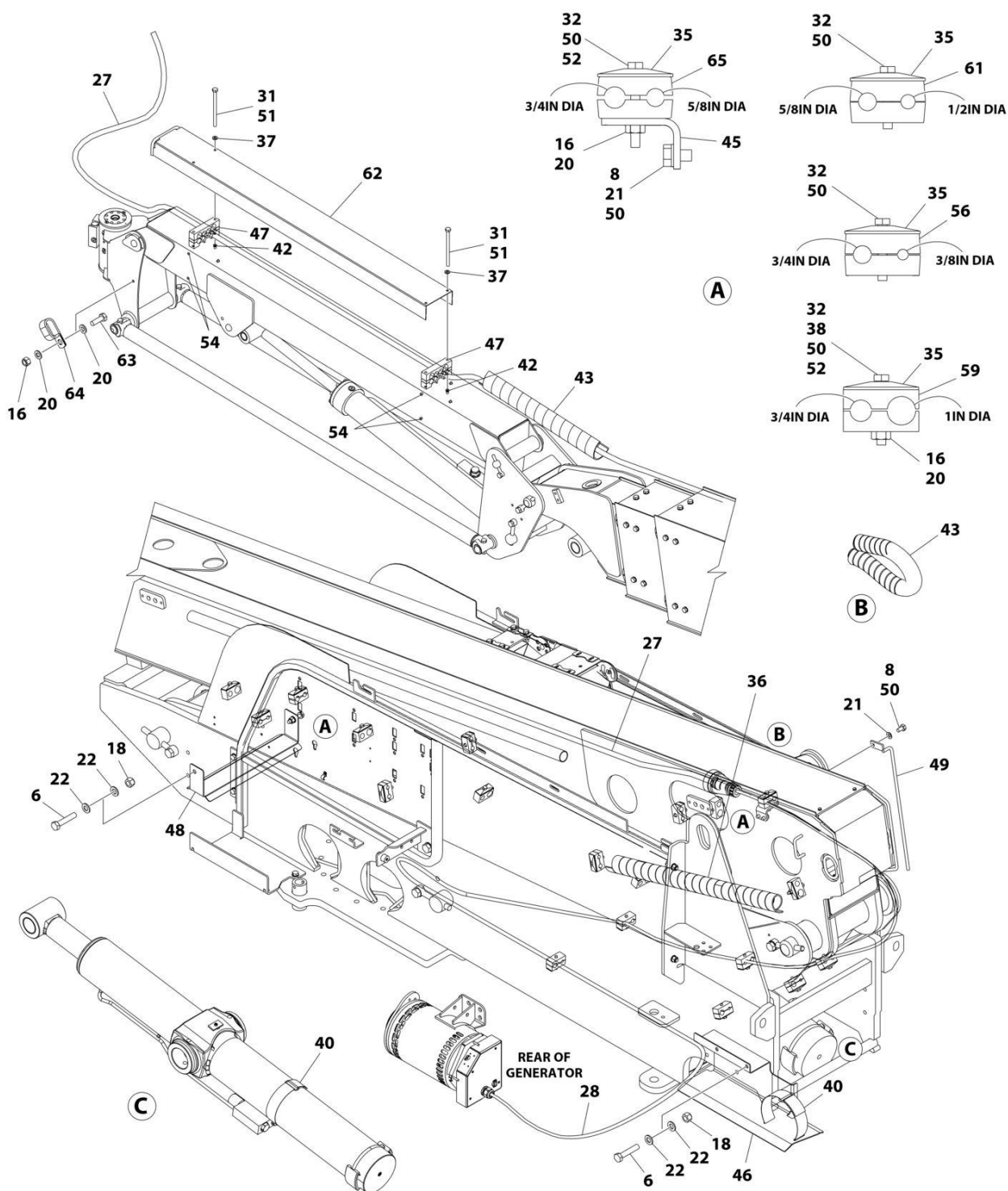
FIGURE 8-31. AC CABLES AND CLAMPS INSTALLATION - WITH 7500W SKYPOWER GENERATOR (SN 0300292972 to Present)
