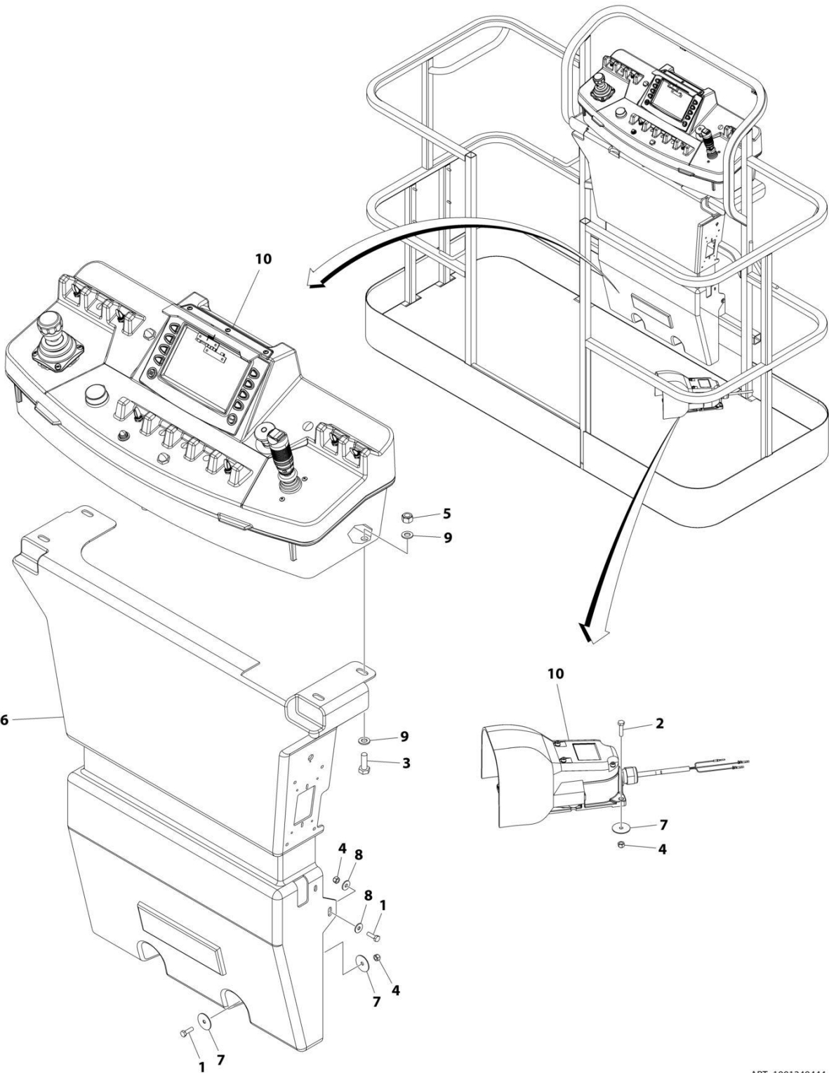
FIGURE 5-15. PLATFORM CONSOLE AND FOOTSWITCH INSTALLATION
