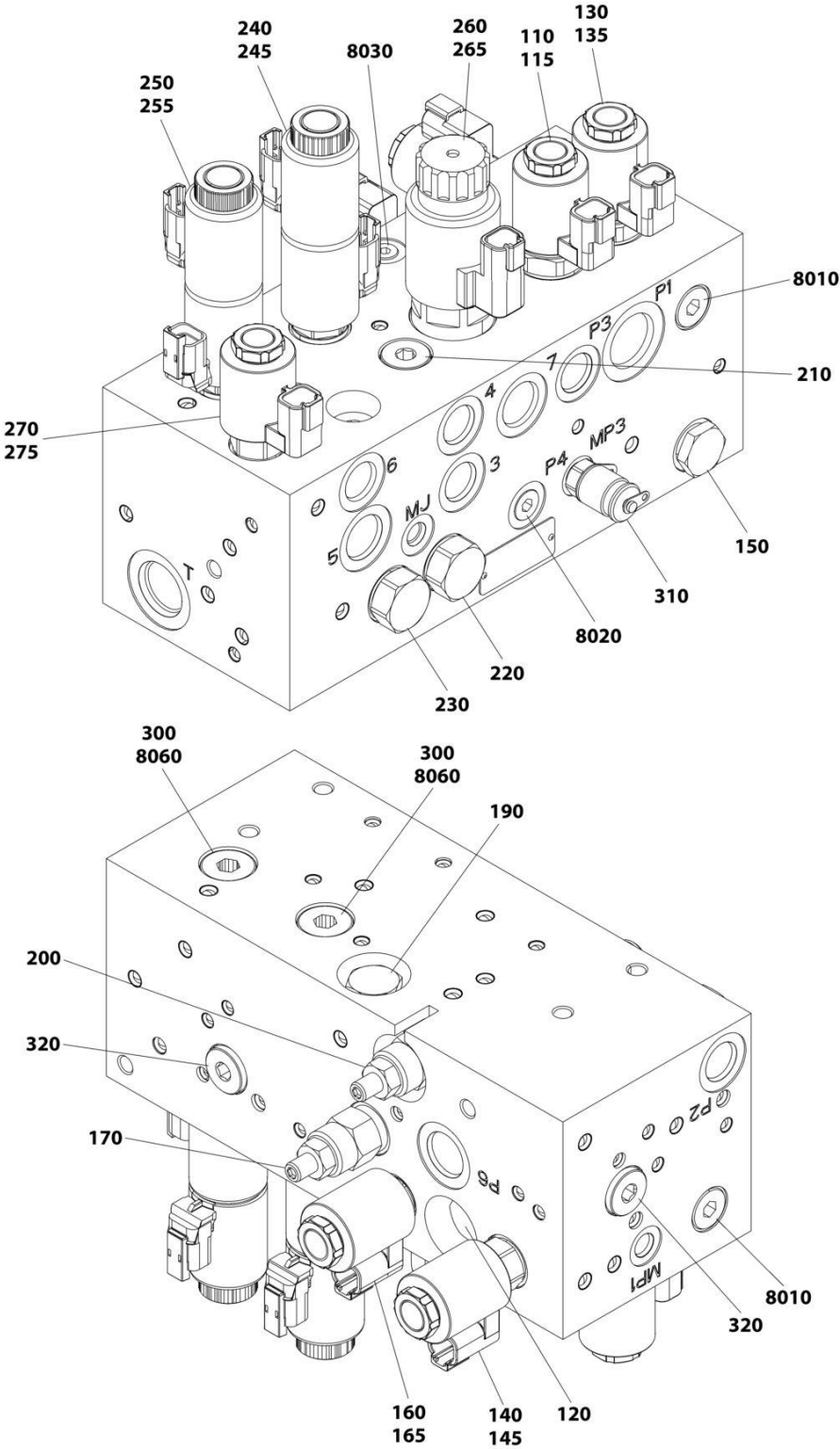
FIGURE 2-2. MAIN CONTROL VALVE ASSEMBLY
