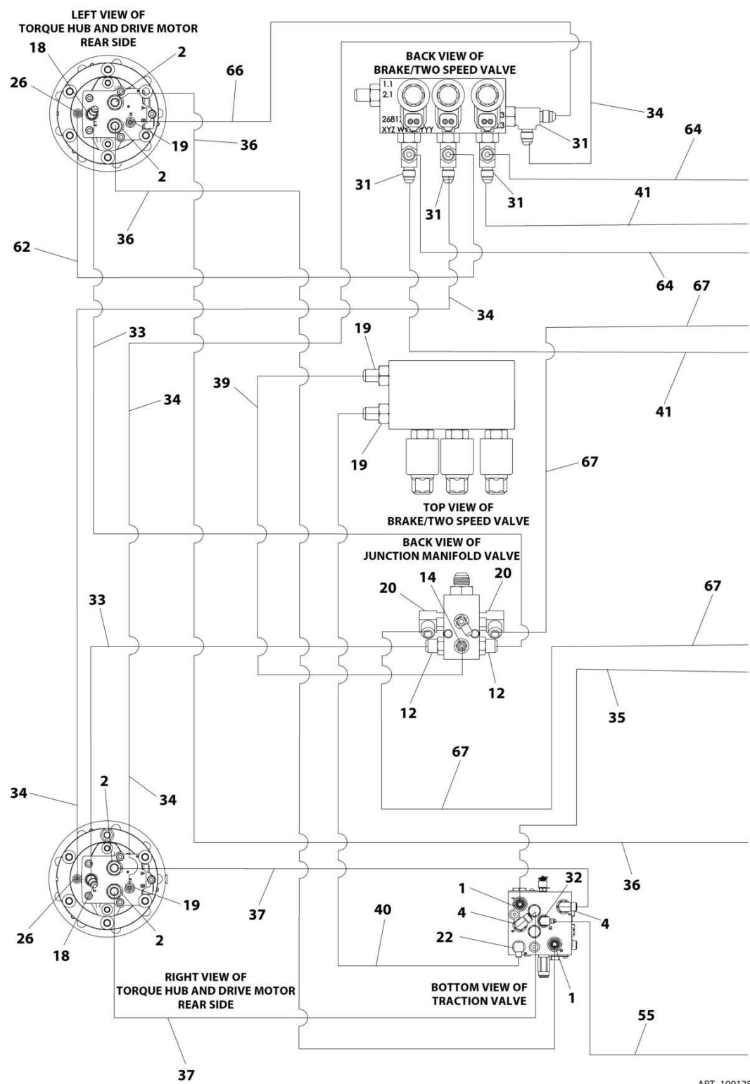
FIGURE 7-2. HYDRAULIC DIAGRAM - CHASSIS
