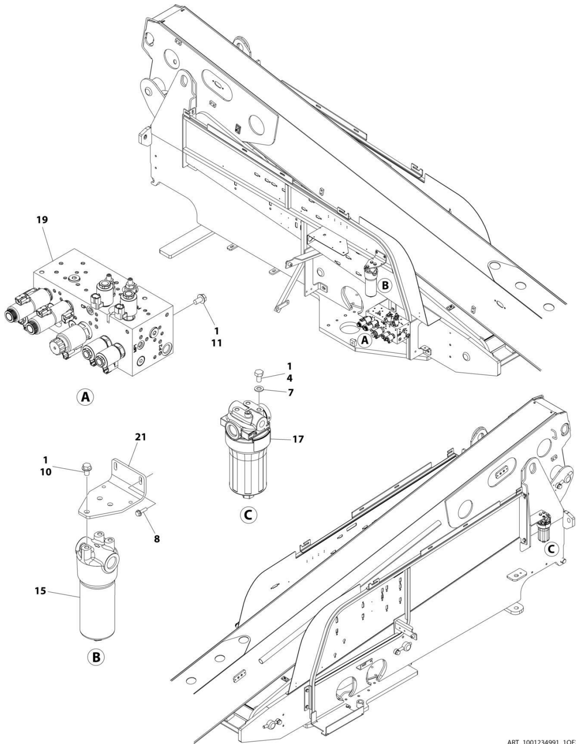
FIGURE 2-1. VALVE INSTALLATION
