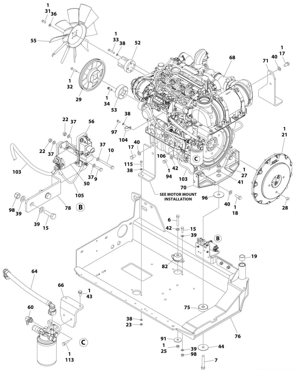
FIGURE 3-12. DEUTZ TD2.9L4 EMR4 ENGINE ASSEMBLY
