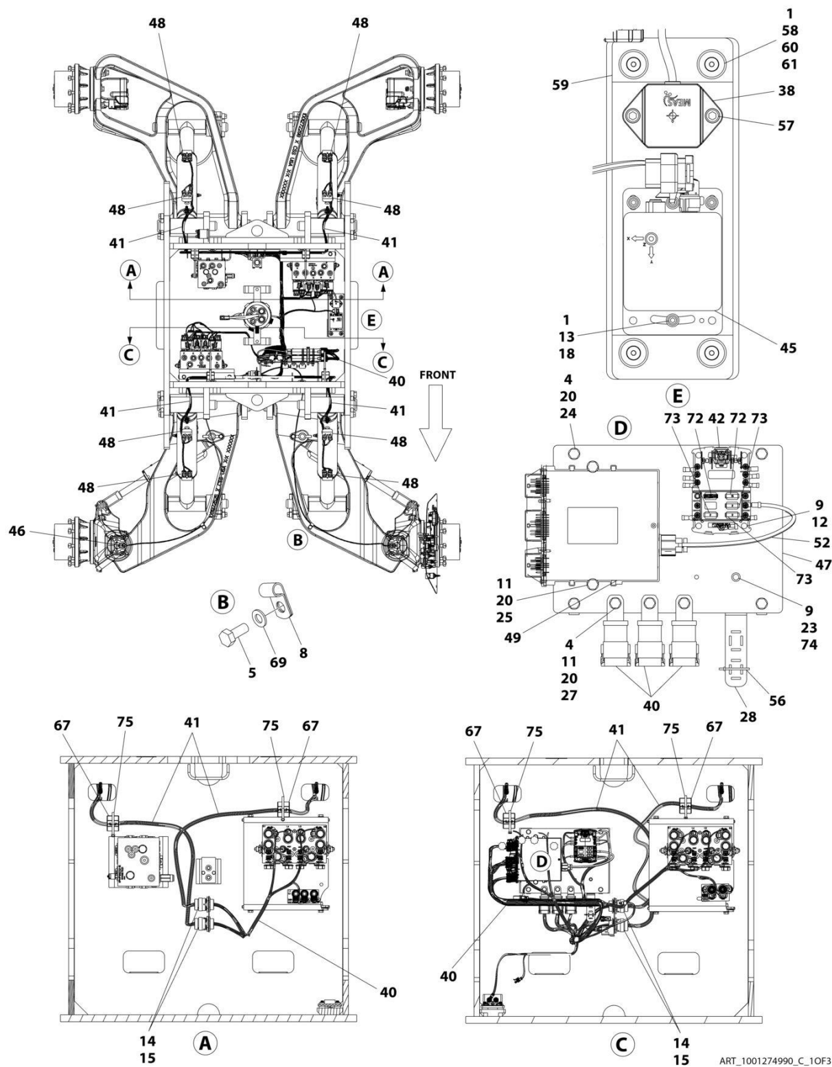
FIGURE 8-4. ELECTRICAL INSTALLATION (DEUTZ DT2.2L3 - STAGE V ENGINES) (Prior to SN 0300311240)
