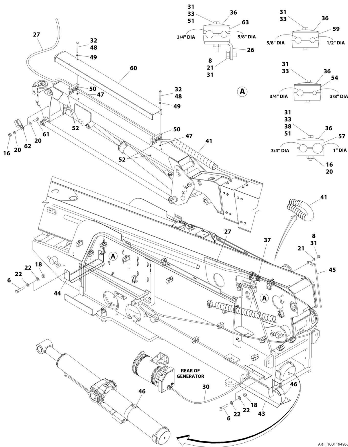
FIGURE 8-28. AC CABLES AND CLAMPS INSTALLATION - WITH 4000W/60HZ GENERATOR (ALL SPECS EXCEPT AUSTRALIAN & CE SPECS) (Prior to SN 0300292972)
