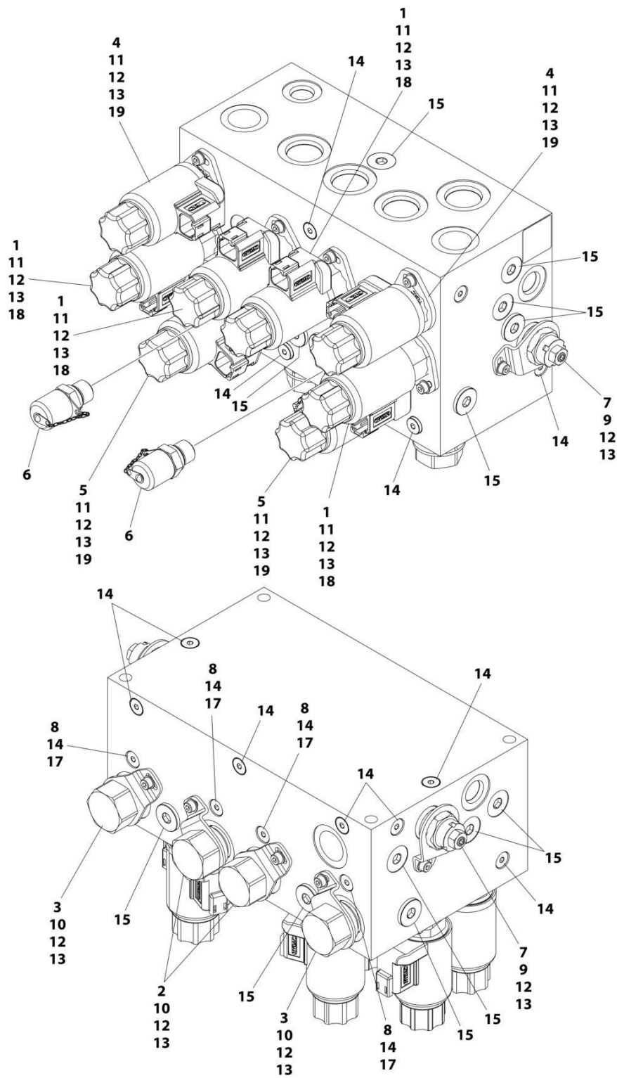
FIGURE 1-6. AXLE CONTROL VALVE ASSEMBLY
