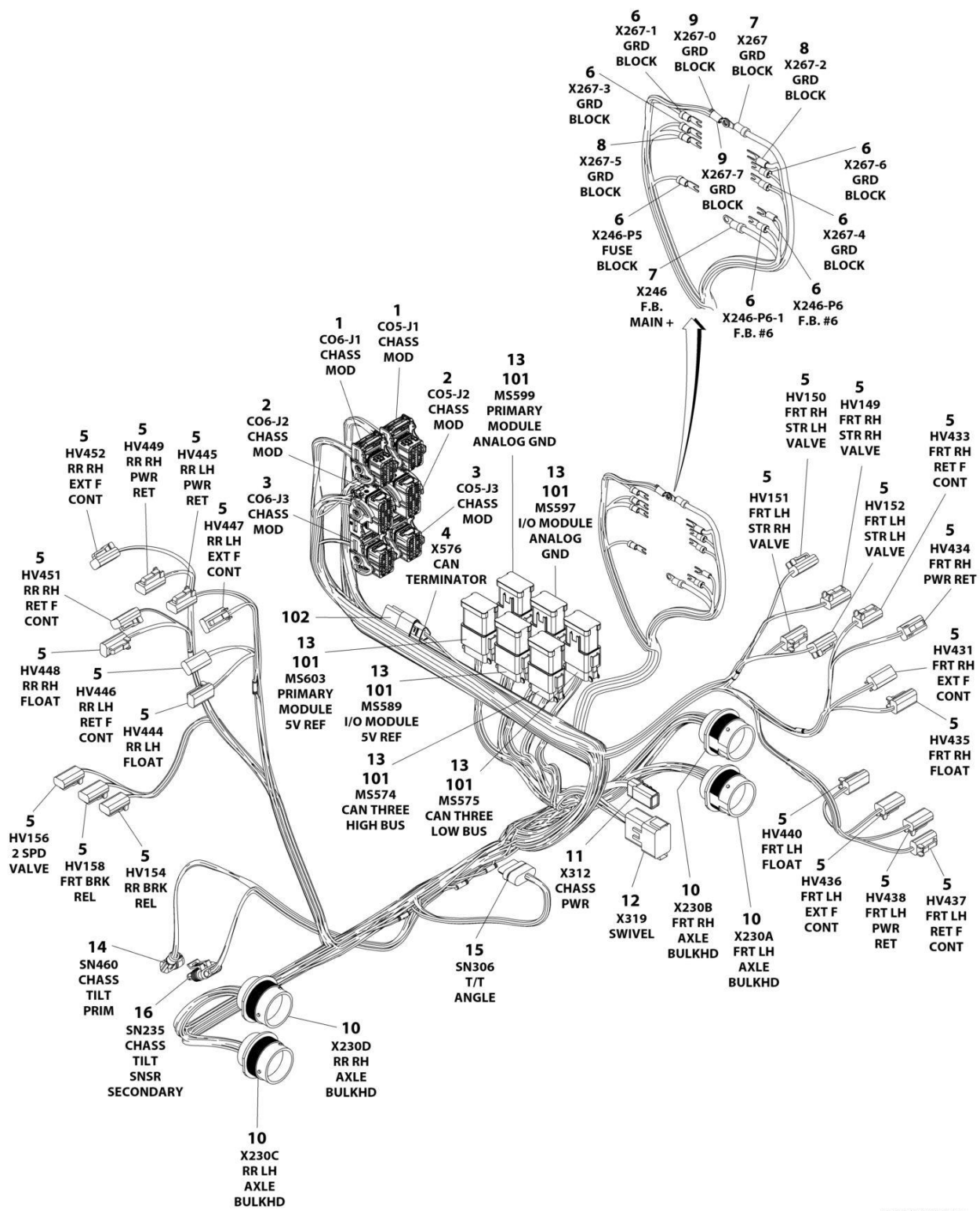
FIGURE 8-42. CHASSIS HARNESS
