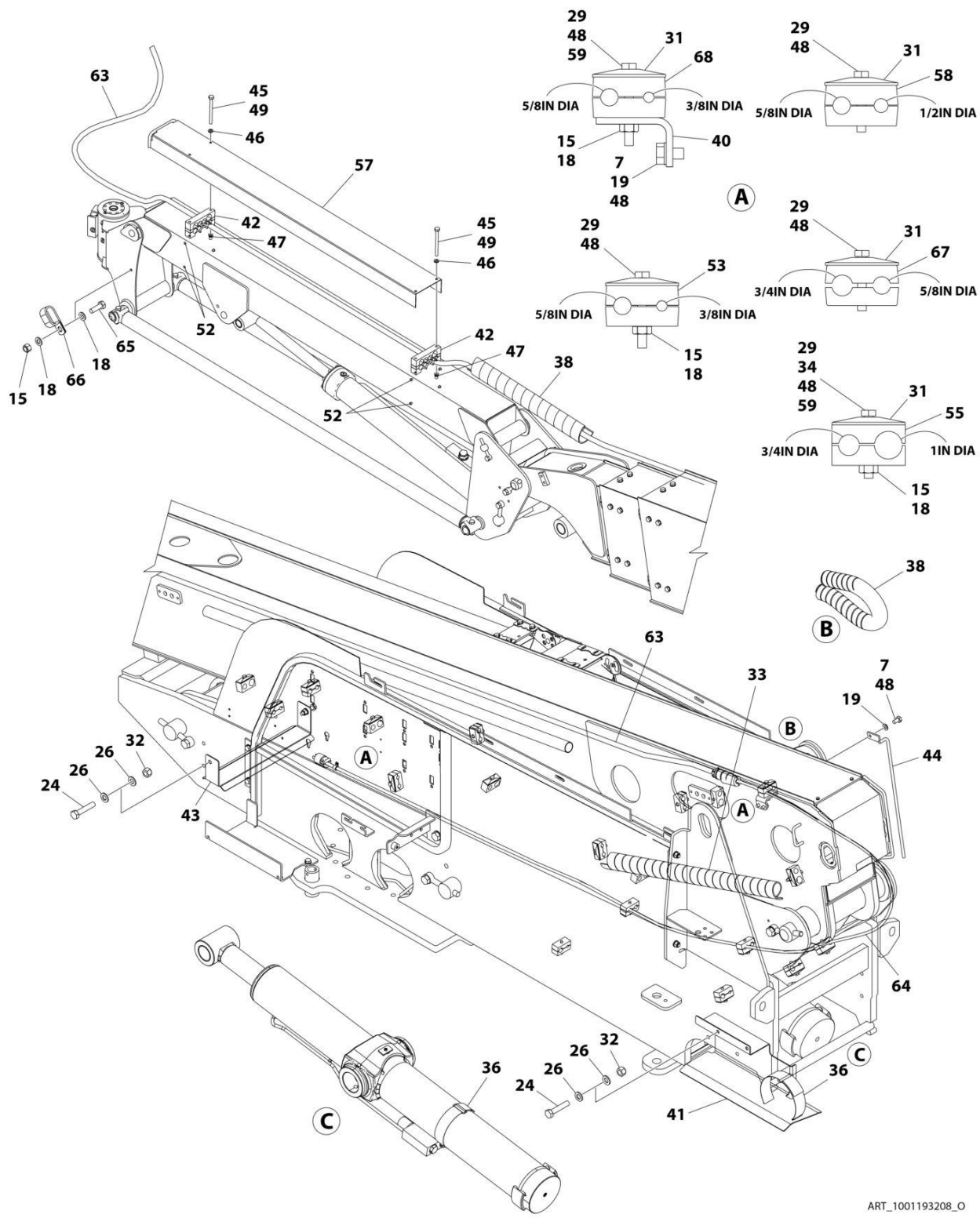
FIGURE 8-23. AC CABLES AND CLAMPS INSTALLATION - WITHOUT GENERATOR (ANSI, CSA AND JAPANESE SPECS) (SN 0300292972 to Present)
