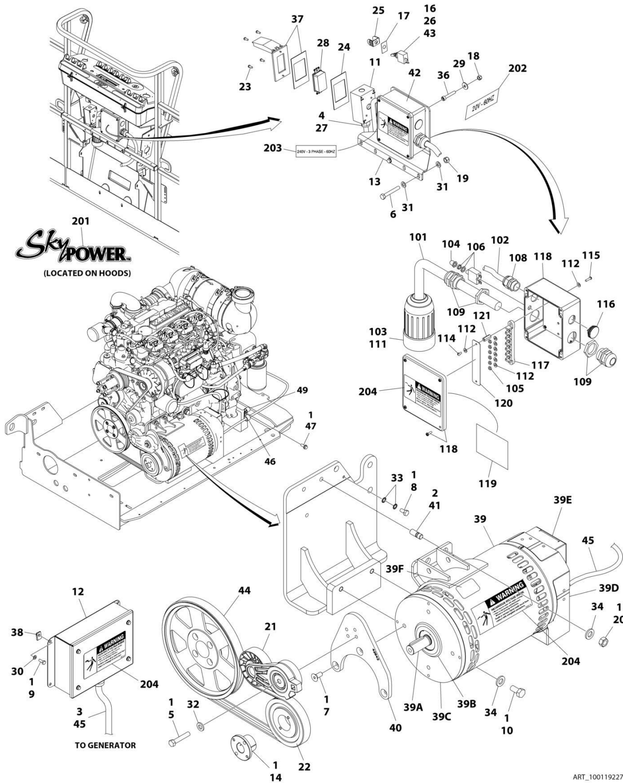
FIGURE 3-46. 7500W SKYPOWER GENERATOR INSTALLATION - 110V/60HZ (DEUTZ TD2.9L4 ENGINES) (OPTIONAL)
