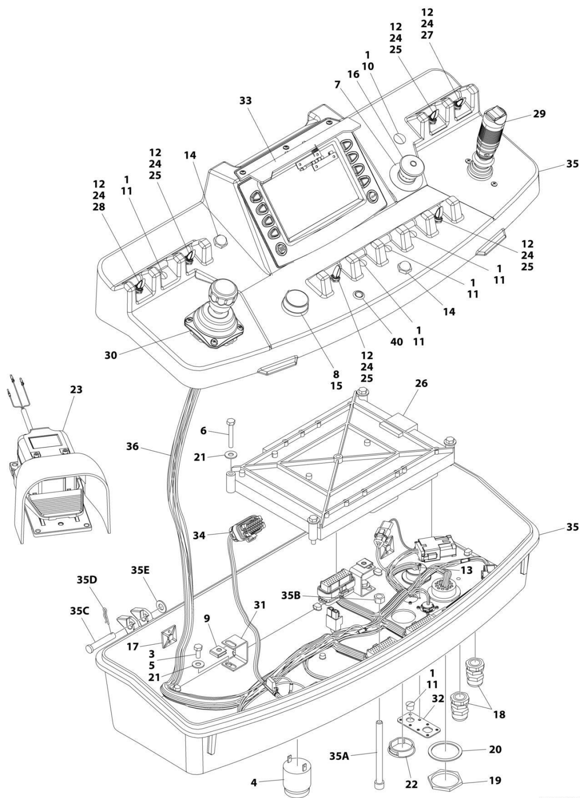
FIGURE 5-16. CONSOLE BOX ASSEMBLY
