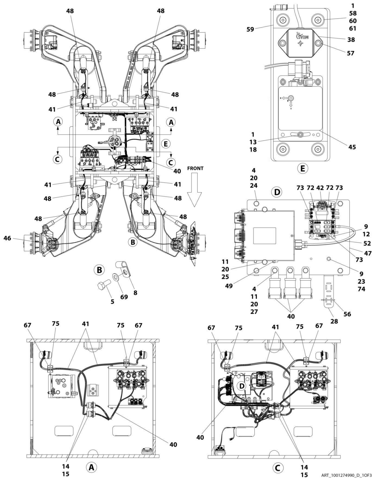
FIGURE 8-5. ELECTRICAL INSTALLATION (DEUTZ DT2.2L3 - STAGE V ENGINES) (SN 0300311240 to Present)
