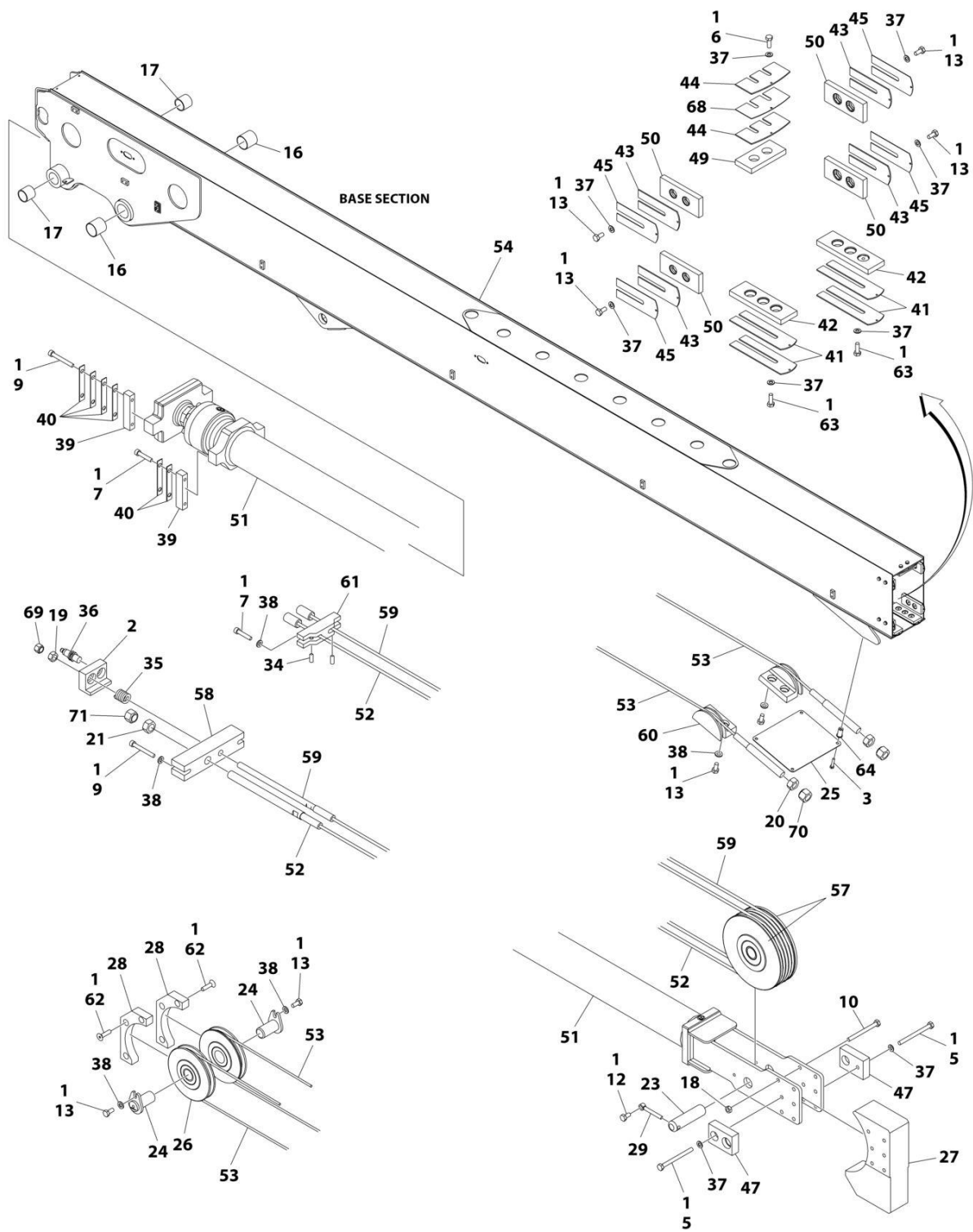
FIGURE 4-2. BOOM ASSEMBLY
