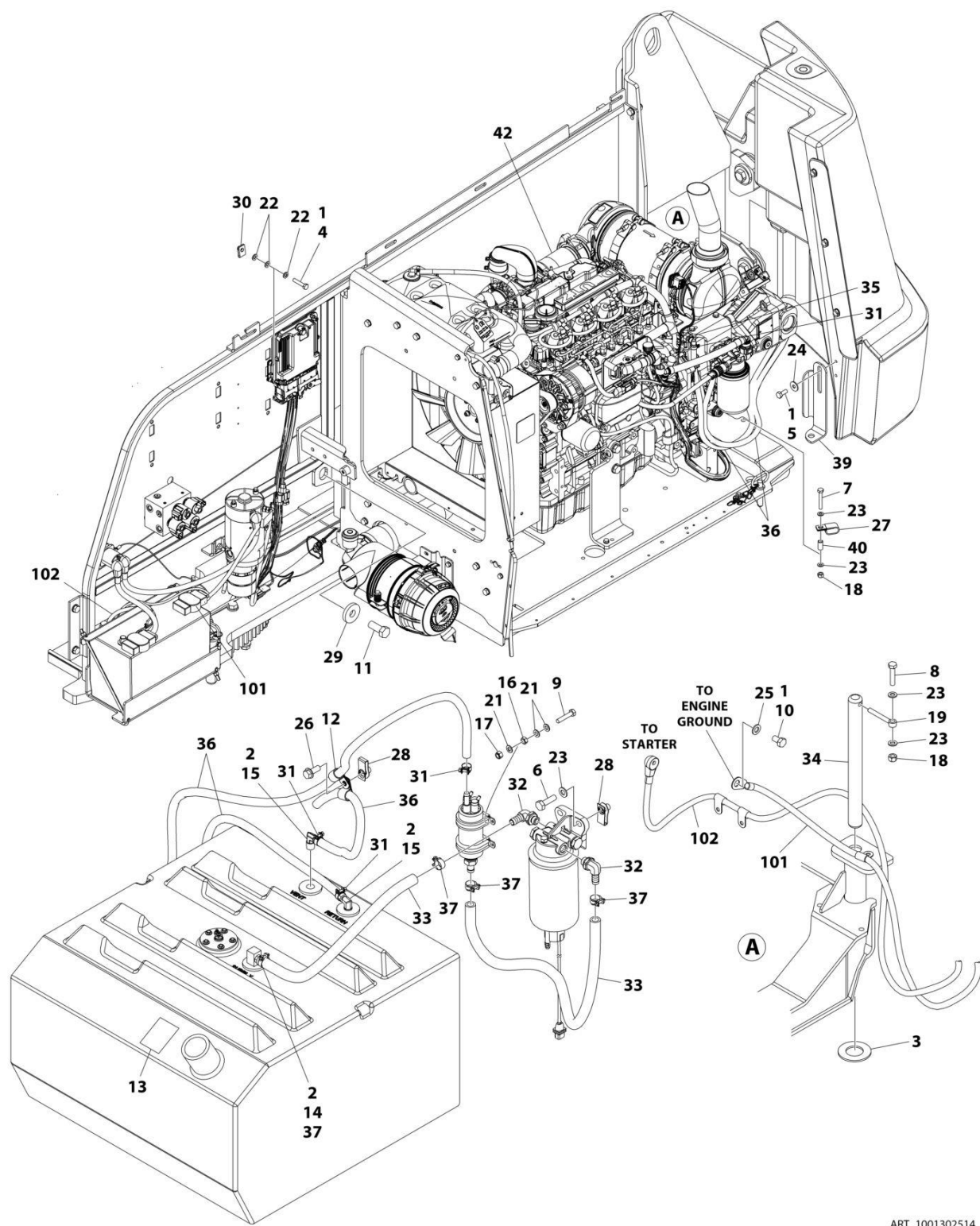
FIGURE 3-14. DEUTZ TD2.9L4 EMR5 ENGINE INSTALLATION
