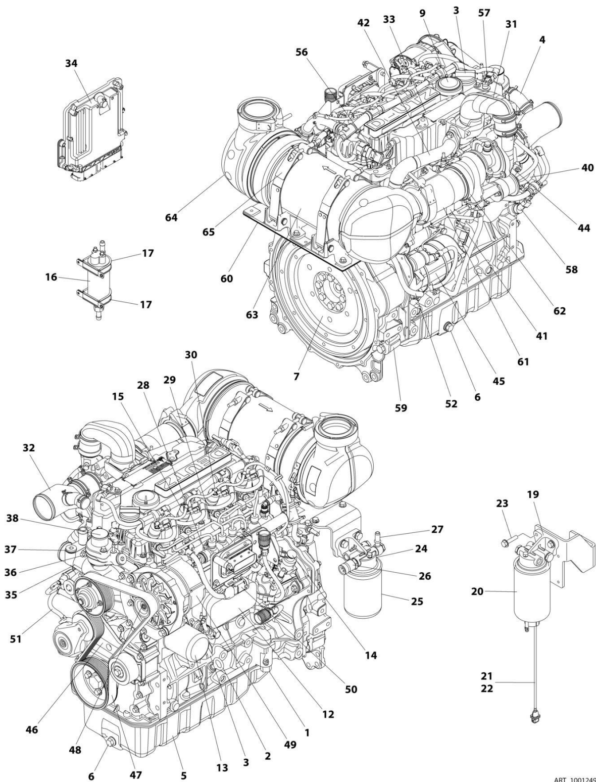
FIGURE 3-13. DEUTZ TD2.9L4 EMR4 ENGINE COMPONENTS
