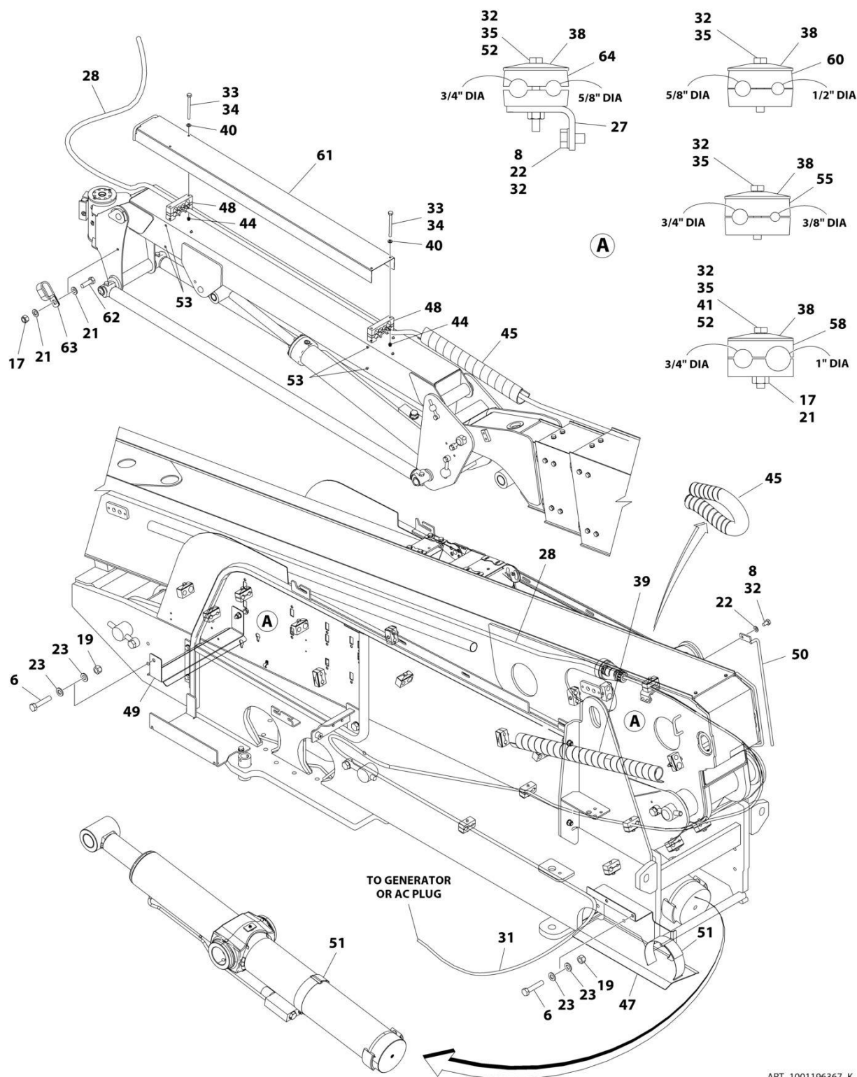
FIGURE 8-26. AC CABLES AND CLAMPS INSTALLATION - WITH 4000W/50HZ GENERATOR (ANSI EXPORT, AUSTRALIAN AND CE SPECS) (Prior to SN 0300292972)
