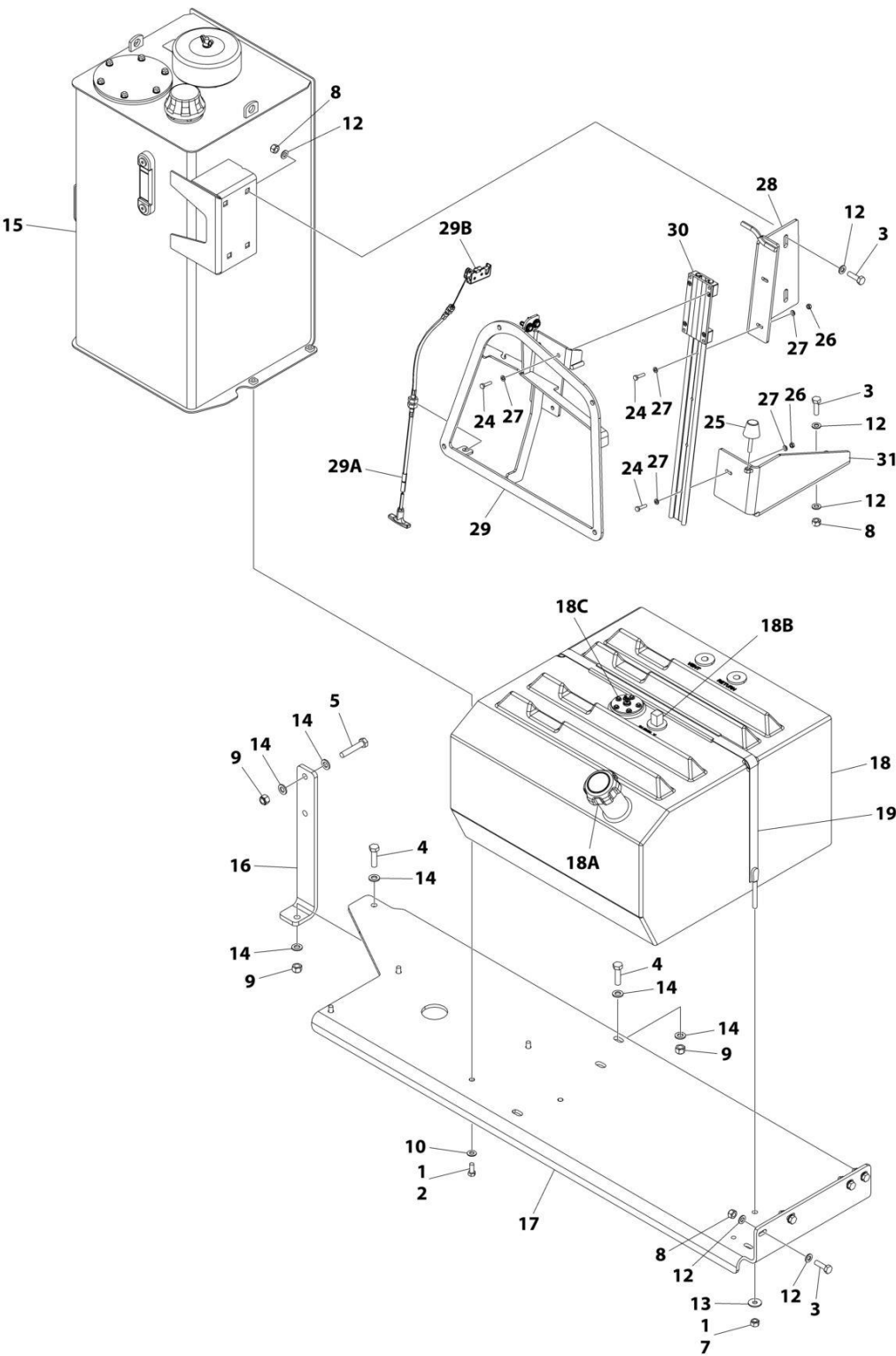
FIGURE 2-9. TANKS INSTALLATION (WITH HELGESEN HYDRAULIC TANK)
