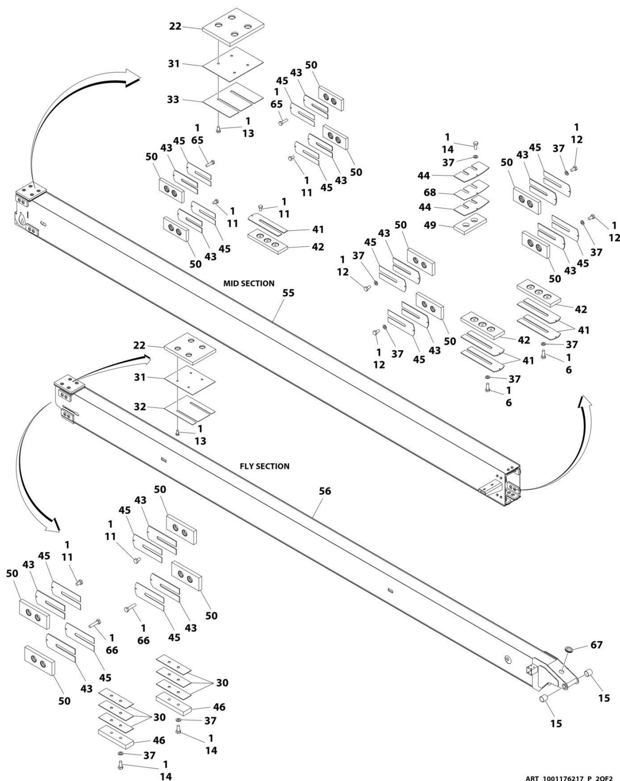
FIGURE 4-3. BOOM ASSEMBLY
