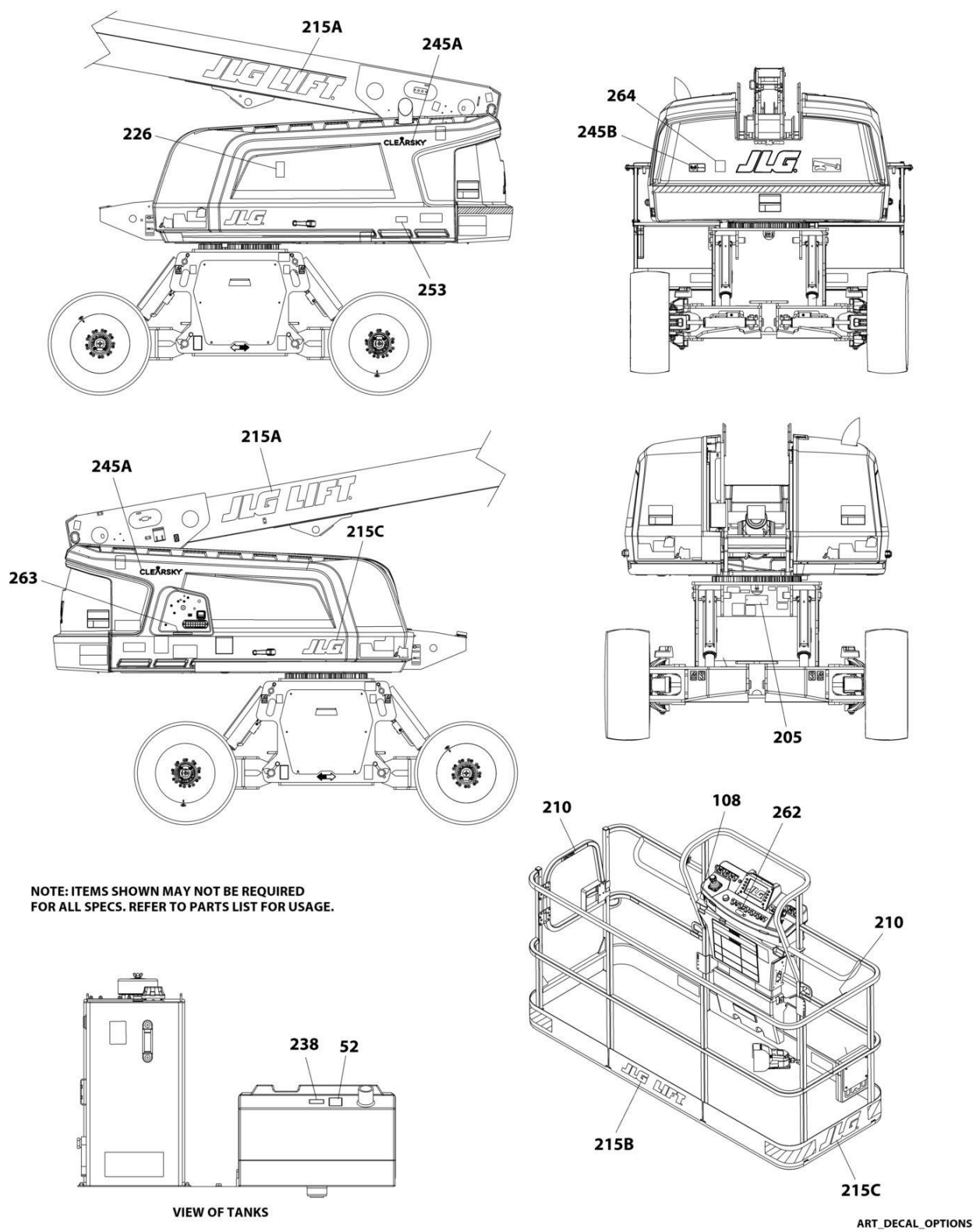
FIGURE 9-12. DECALS INSTALLATION - OPTIONS
