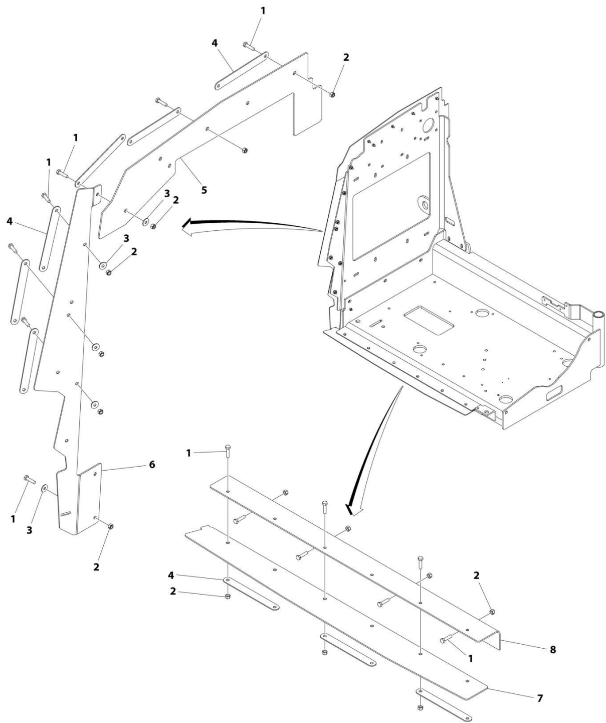
FIGURE 3-35. ENGINE HOOD Baffles INSTALLATION - ABS HOODS (DEUTZ D2.2L3 STAGE V ENGINES)
