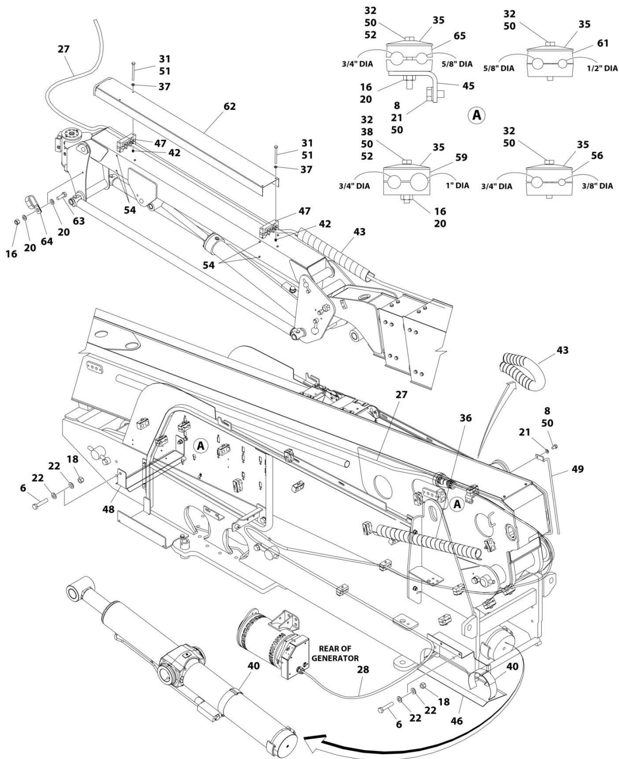
FIGURE 8-30. AC CABLES AND CLAMPS INSTALLATION - WITH 7500W SKYPOWER GENERATOR (Prior to SN 0300292972)
