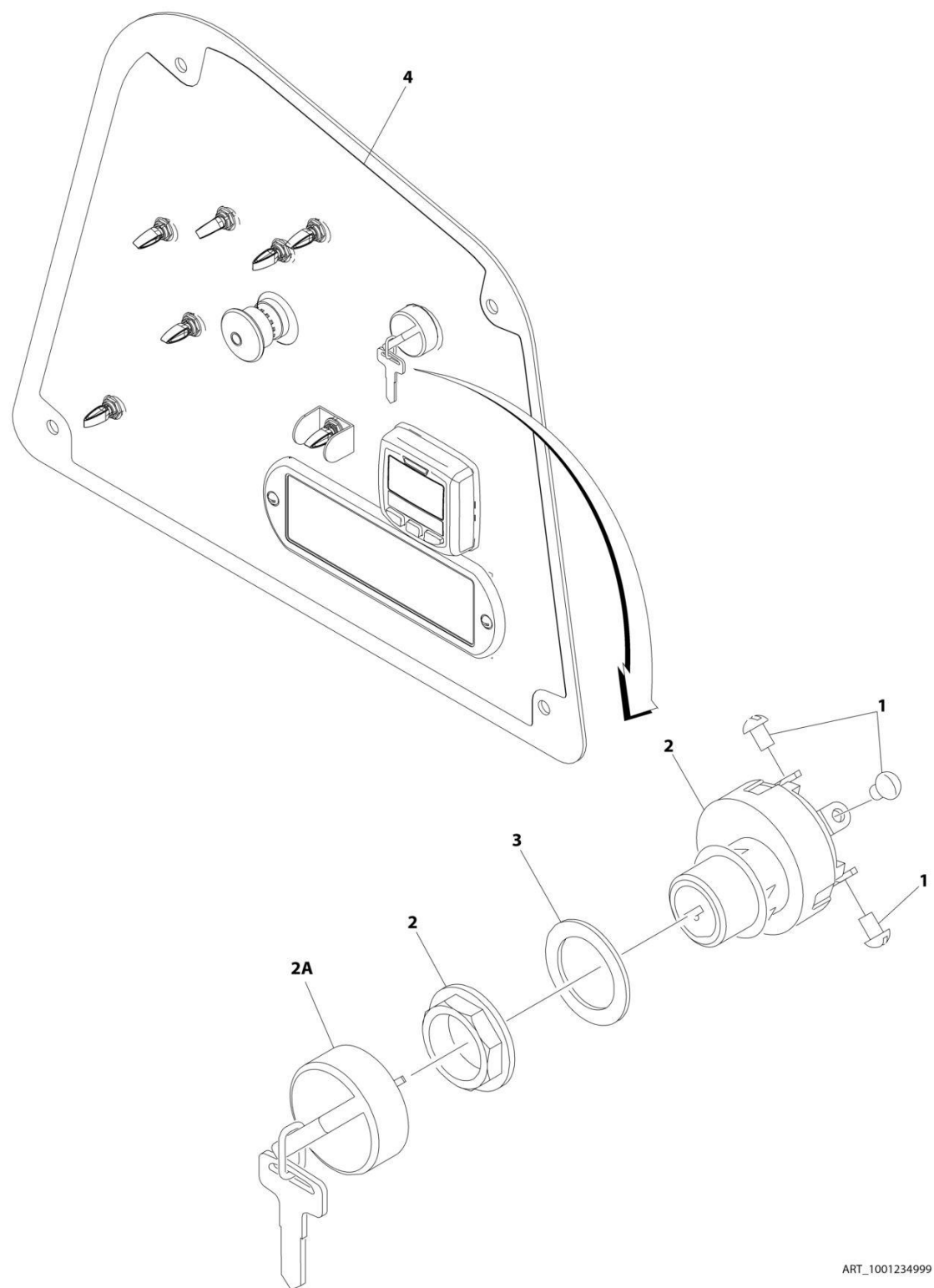
FIGURE 2-17. KEYSWITCH INSTALLATION (ALL SPECS EXCEPT CE SPECS)
