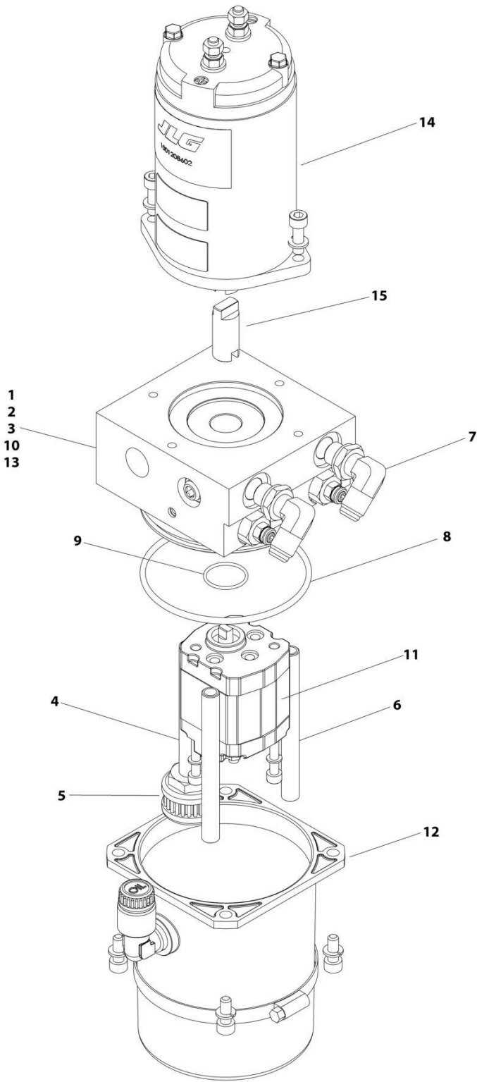
FIGURE 4-8. PUMP ASSEMBLY - POWER TRAY
