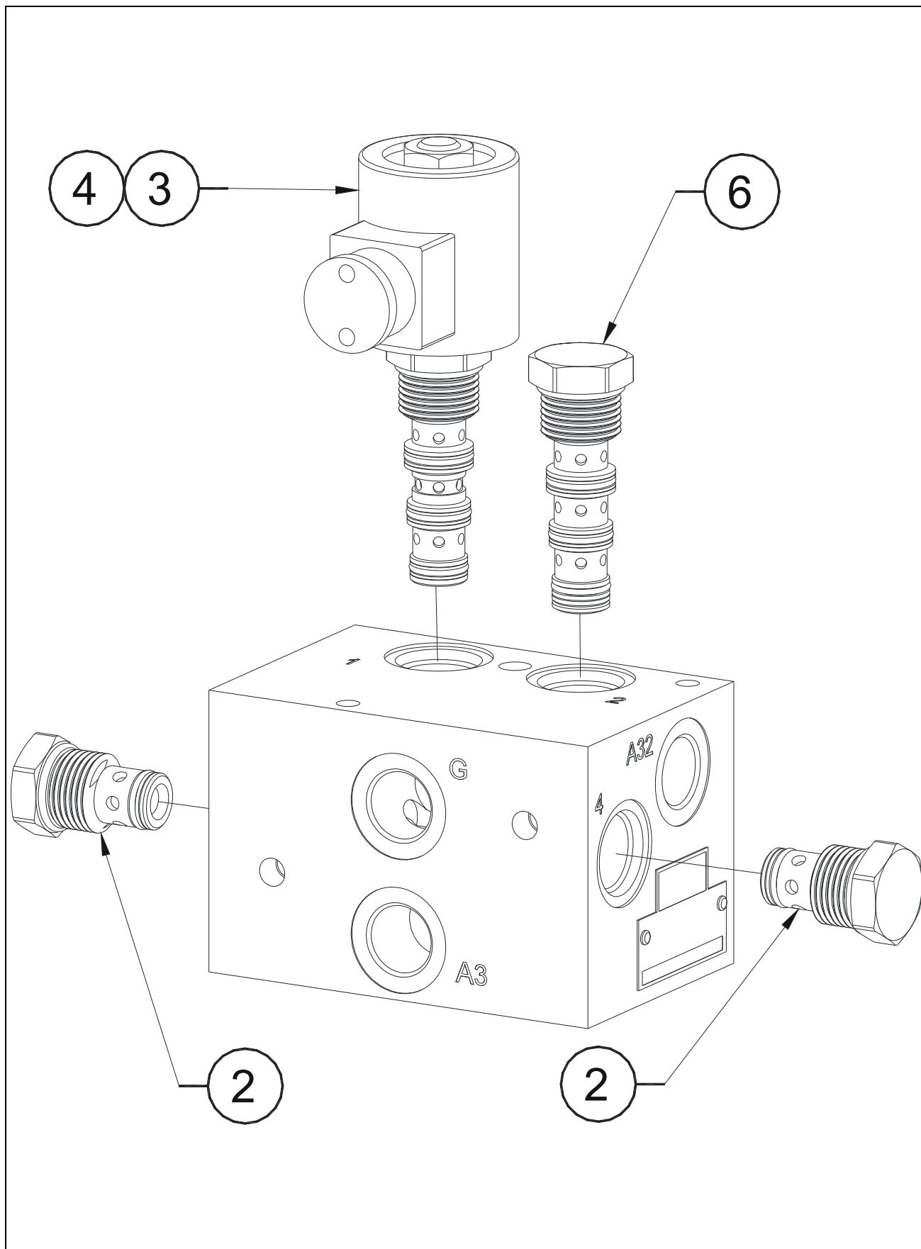
FIGURE 4-1-9-1. DIFFLOCK MANIFOLD / BLOCK DIFFERENTIEL
