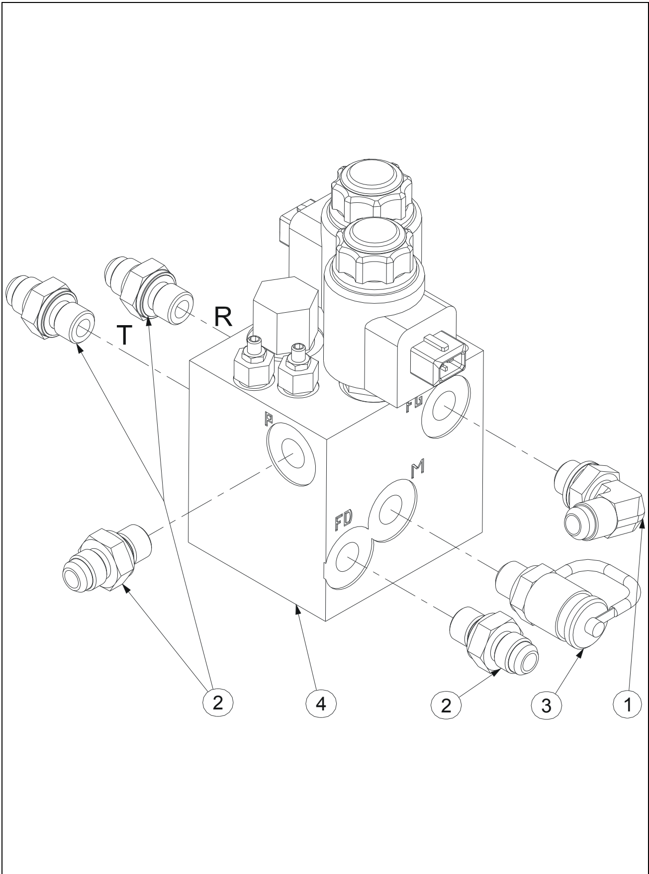
FIGURE 4-1-3. BRAKE MANIFOLD ASSEMBLY / ASSEMBLAGE BLOC FREINAGE
