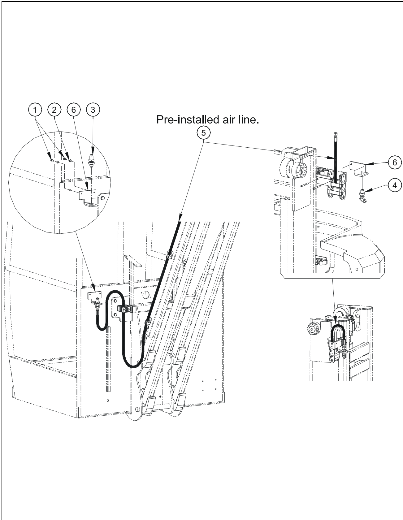
FIGURE 8-3. E26MJ #A300026057 TO PRESENT / A MAINTENANT & E18MJ #A300018037 TO PRESENT / A MAINTENANT AIR LINE INSTALL / INSTALLATION AIR COMPRIME
