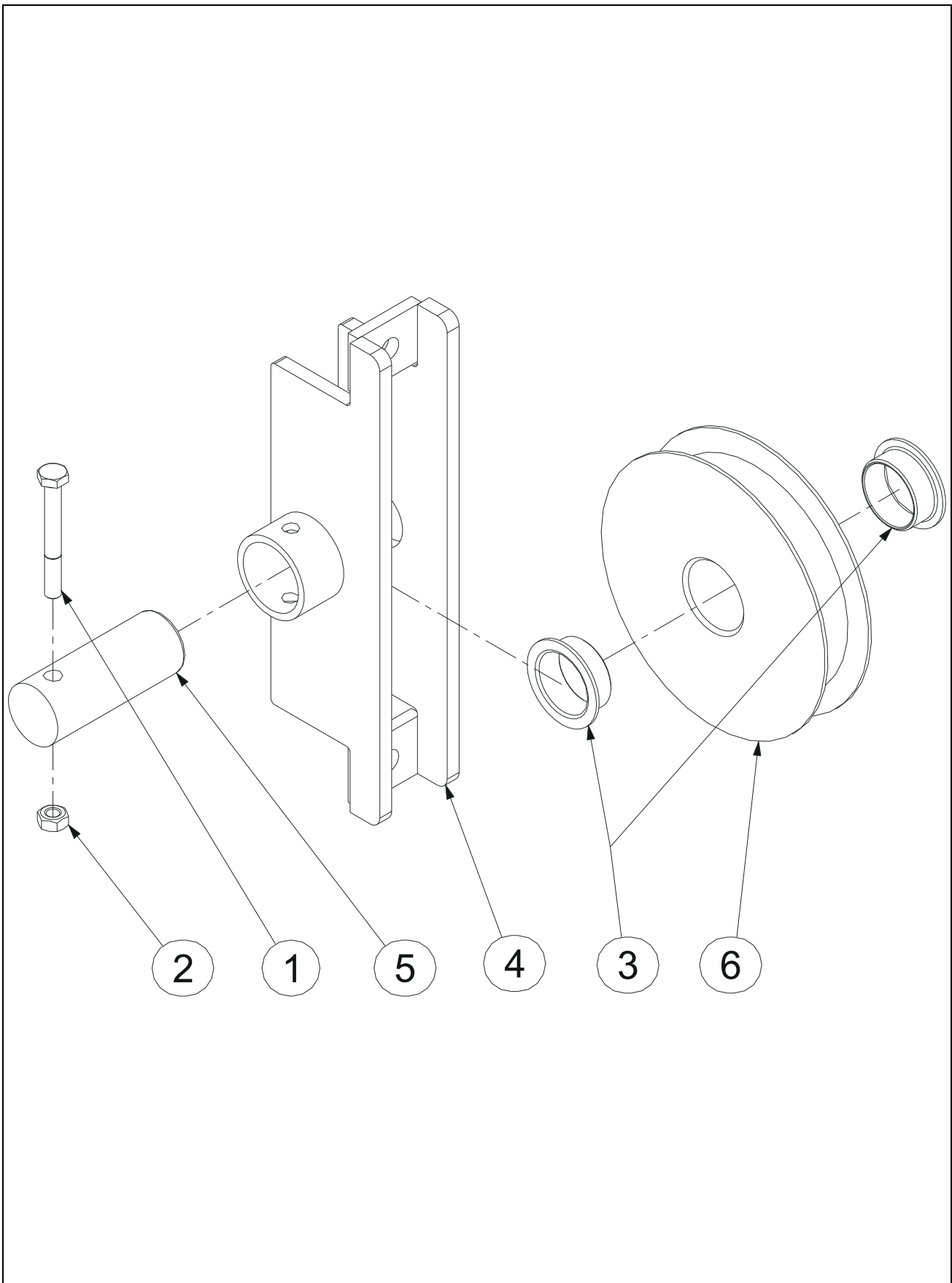
FIGURE 3-4. LL10-44 PULEY ASSEMBLY / ASSEMBLAGE SUPPORT POULIE
