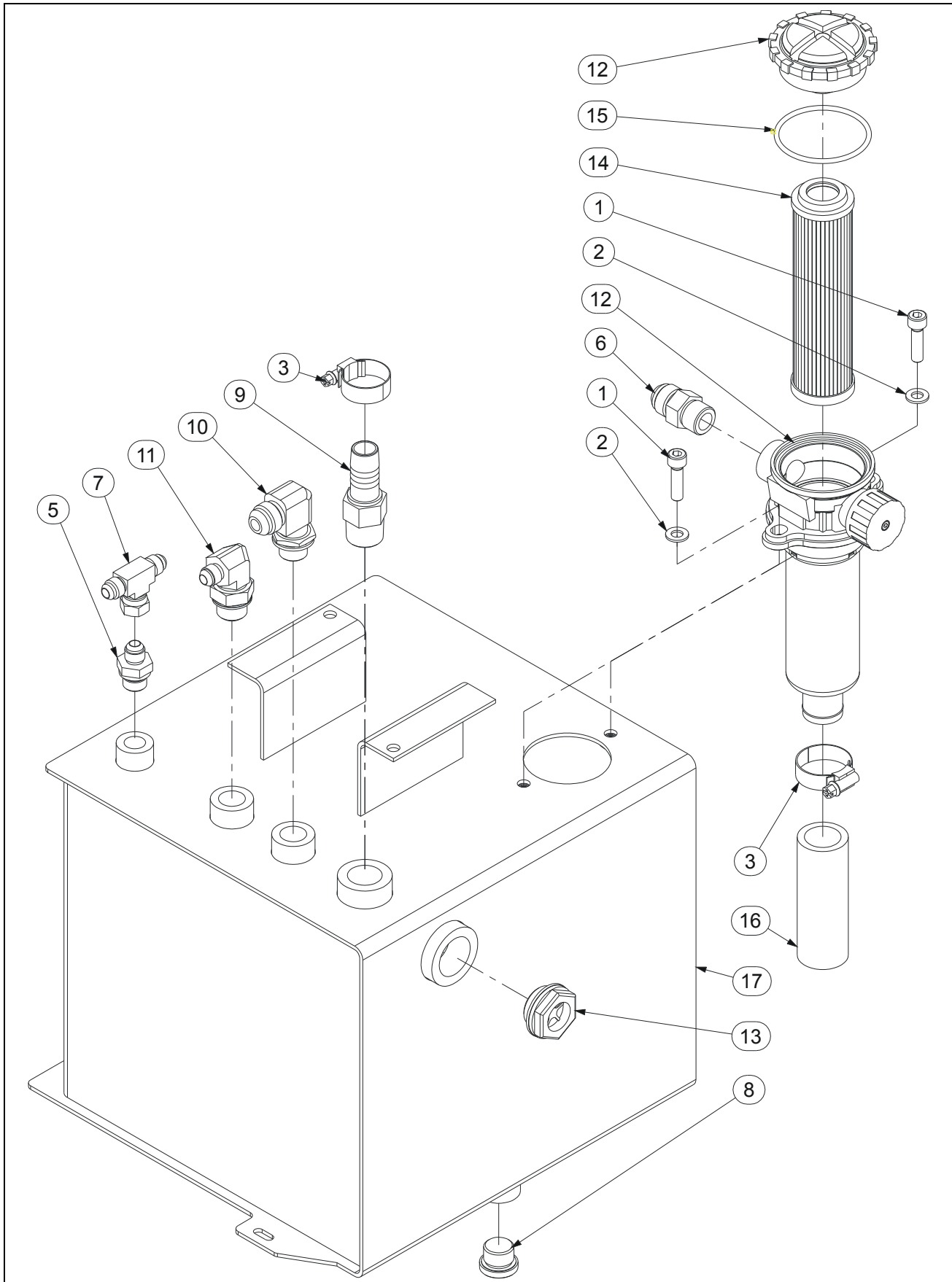
FIGURE 4-1-6. RESERVOIR ASSEMBLY / ASSEMBLAGE RESERVOIR
