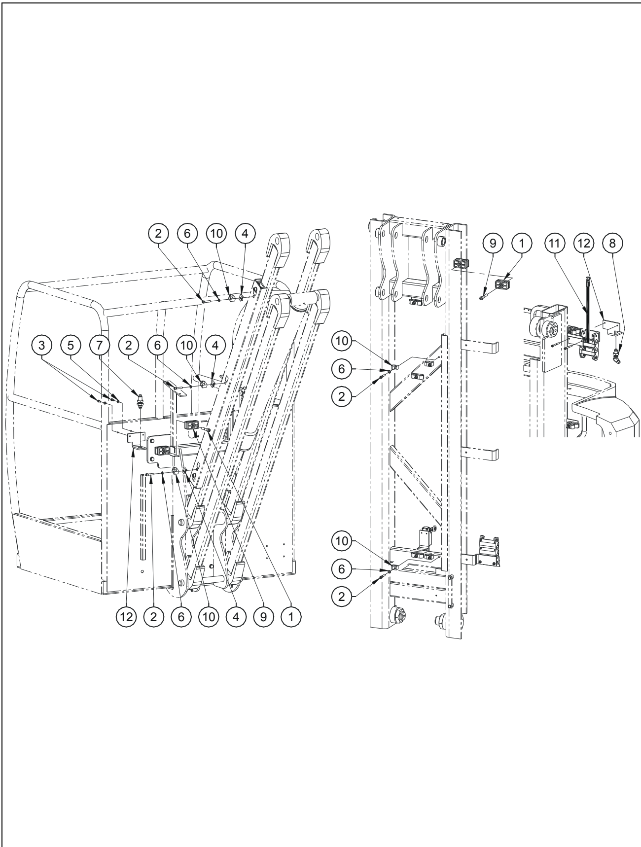
FIGURE 8-2. PRIOR / AVANT E26MJ #A300026057 AIR LINE INSTALL / INSTALLATION AIR COMPRIME
