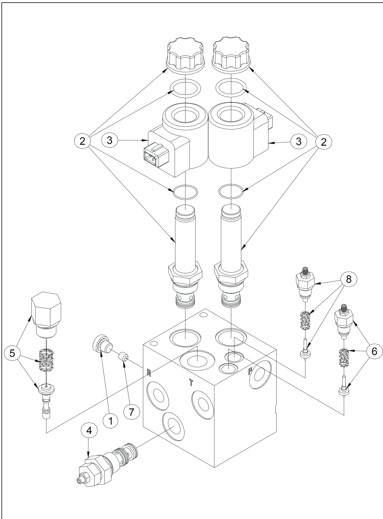
FIGURE 4-1-3-1. BRAKE MANIFOLD / BLOC FREINAGE
