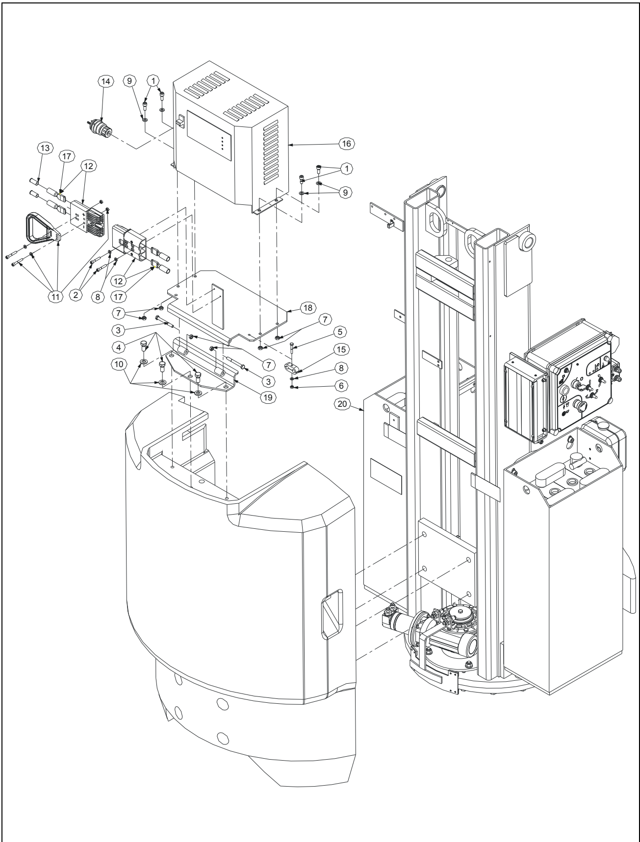
FIGURE 6-2. LOW FREQUENCY CHARGER INSTALL / INSTALLATION CHARGEUR BASSE FREQUENCE
