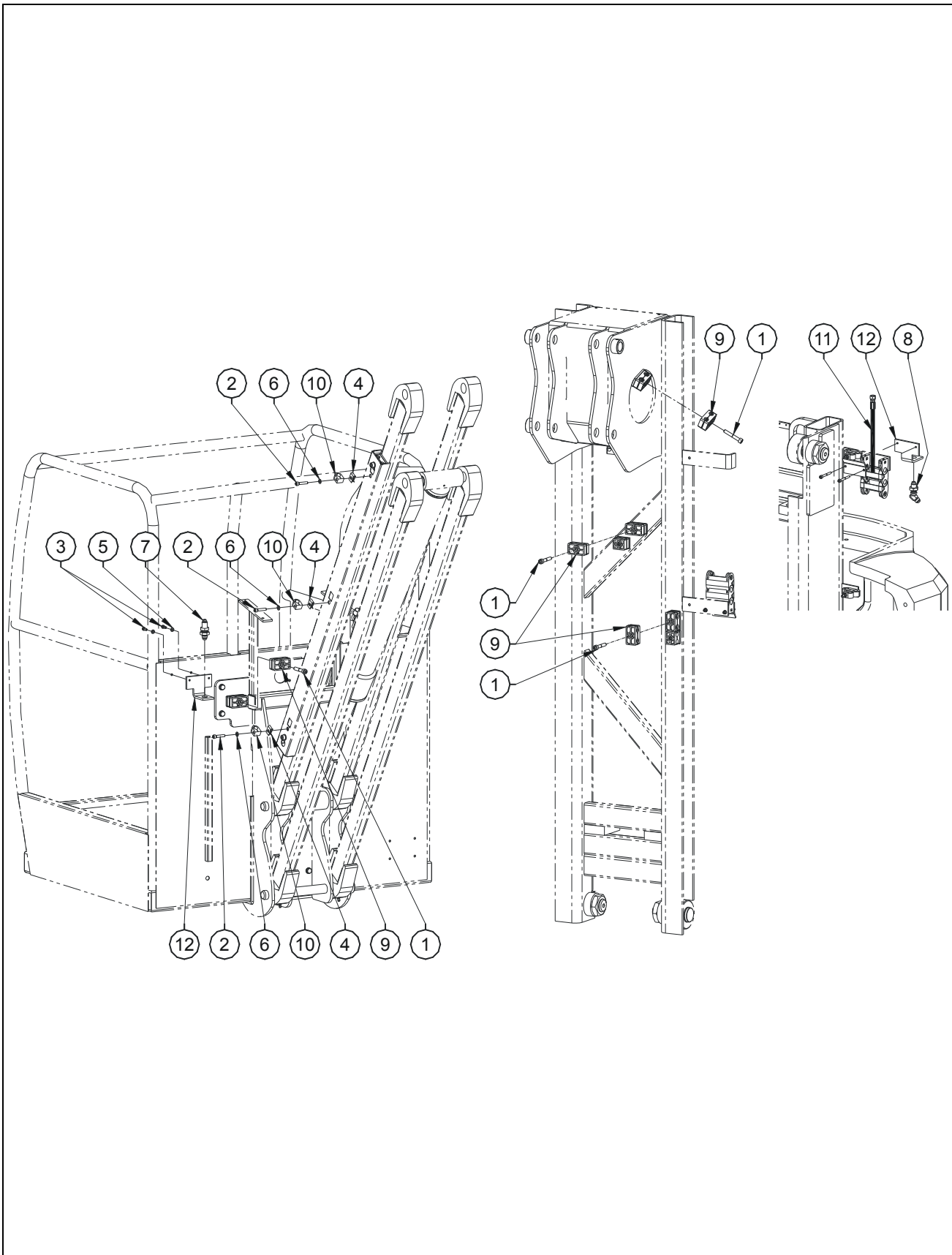
FIGURE 8-1. PRIOR / AVANT E18MJ #A300018037 AIR LINE INSTALL / INSTALLATION AIR COMPRIME
