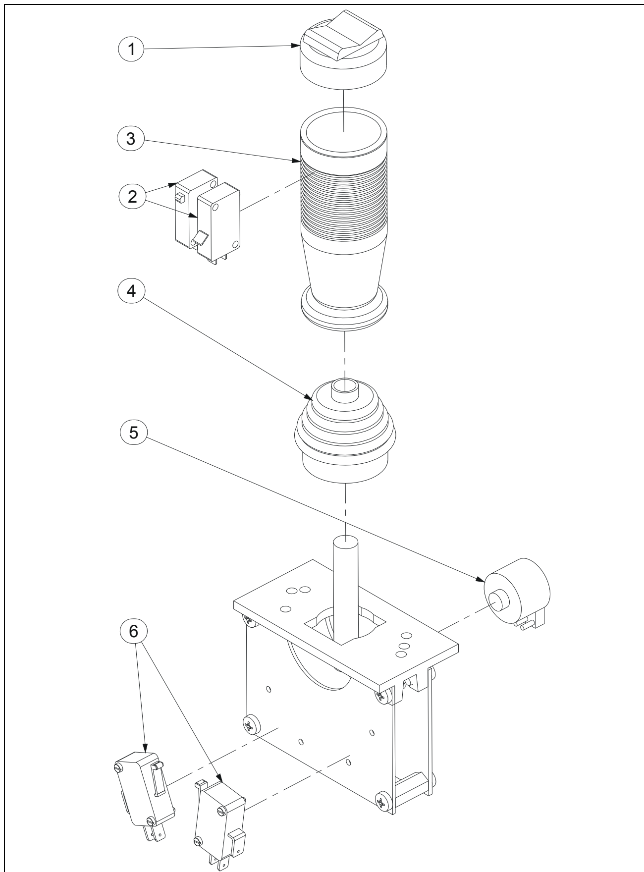
FIGURE 2-3-5-3.JOYSTICK COMPONENTS / COMPOSANTS MANIPULATEUR
