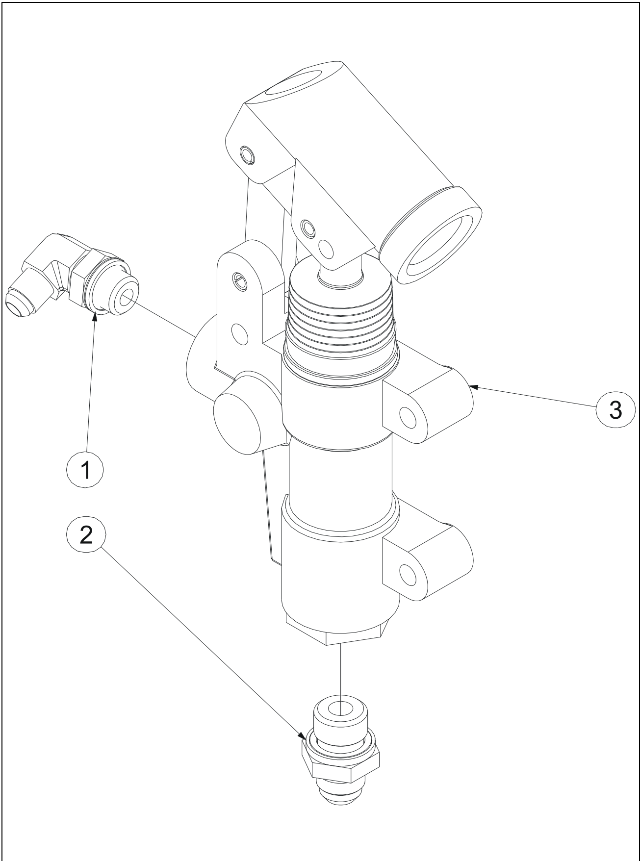
FIGURE 4-1-5. HAND PUMP ASSEMBLY / ASSEMBLAGE POMPE A MAIN
