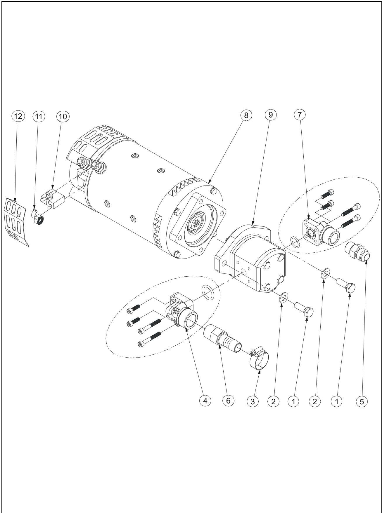
FIGURE 4-1-1. 5.2cc/rev POWER UNIT INSTALL / INSTALLATION CENTRALE 5.2cm 3 /tr
