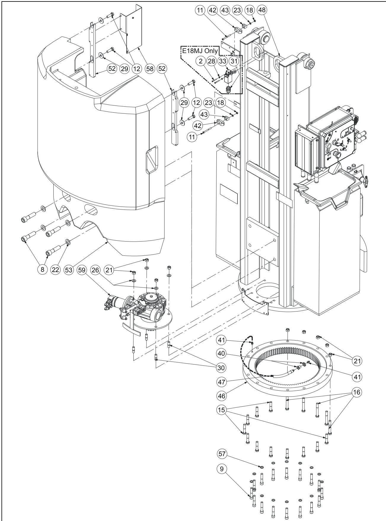
FIGURE 3-3. MAST 1 ASSEMBLY / ASSEMBLAGE MAT 1
