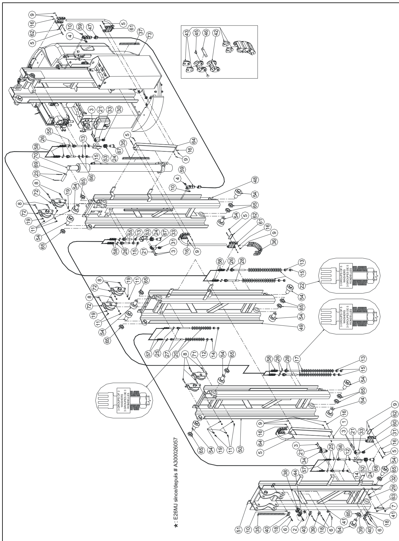
FIGURE 3-2. E26MJ MASTS ASSEMBLY / ASSEMBLAGE MATS E26MJ
