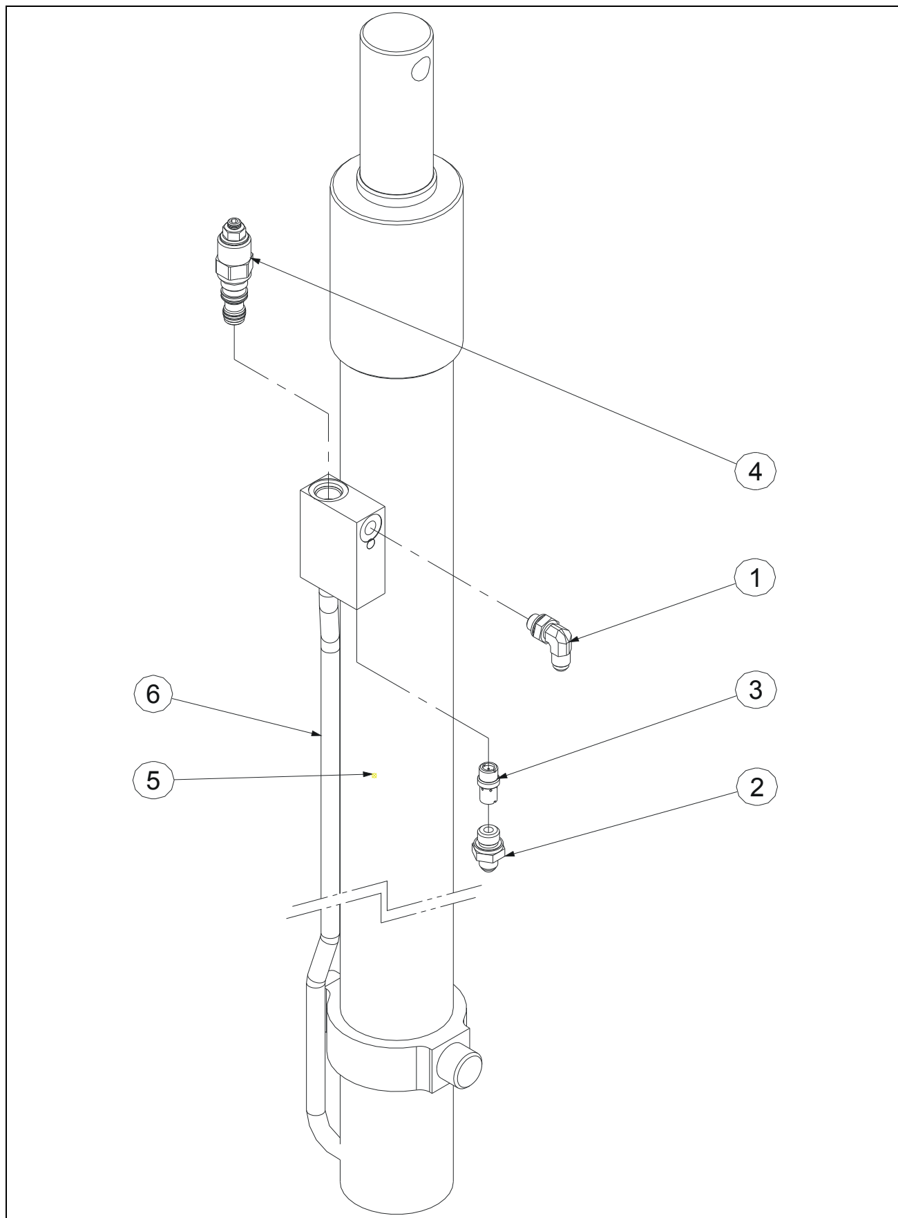
FIGURE 3-6. MAST CYLINDER ASSEMBLY / ASSEMBLAGE VERIN DE MAT
