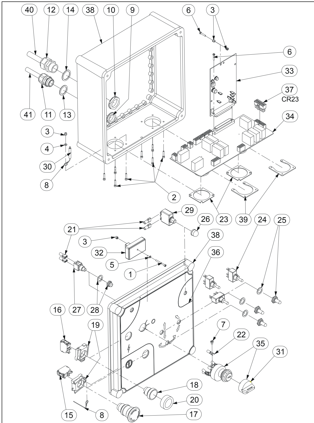
FIGURE 2-3-3.LOWER CONTROL BOX ASSEMBLY / ASSEMBLAGE BOITIER BAS
