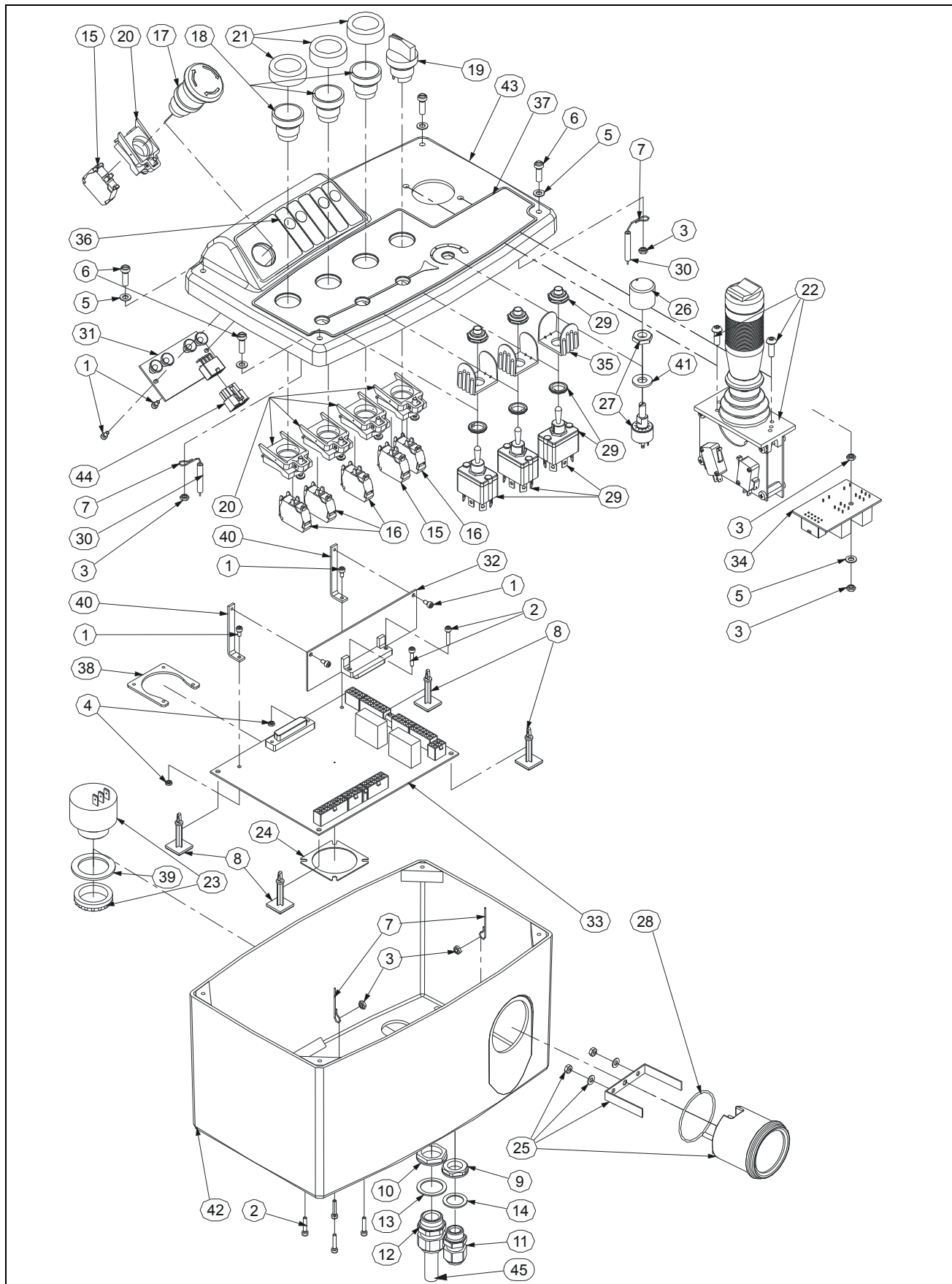
FIGURE 2-3-4.S/N PRIOR / AVANT E18MJ #A300018047 & E26MJ #A300026073 UCB
