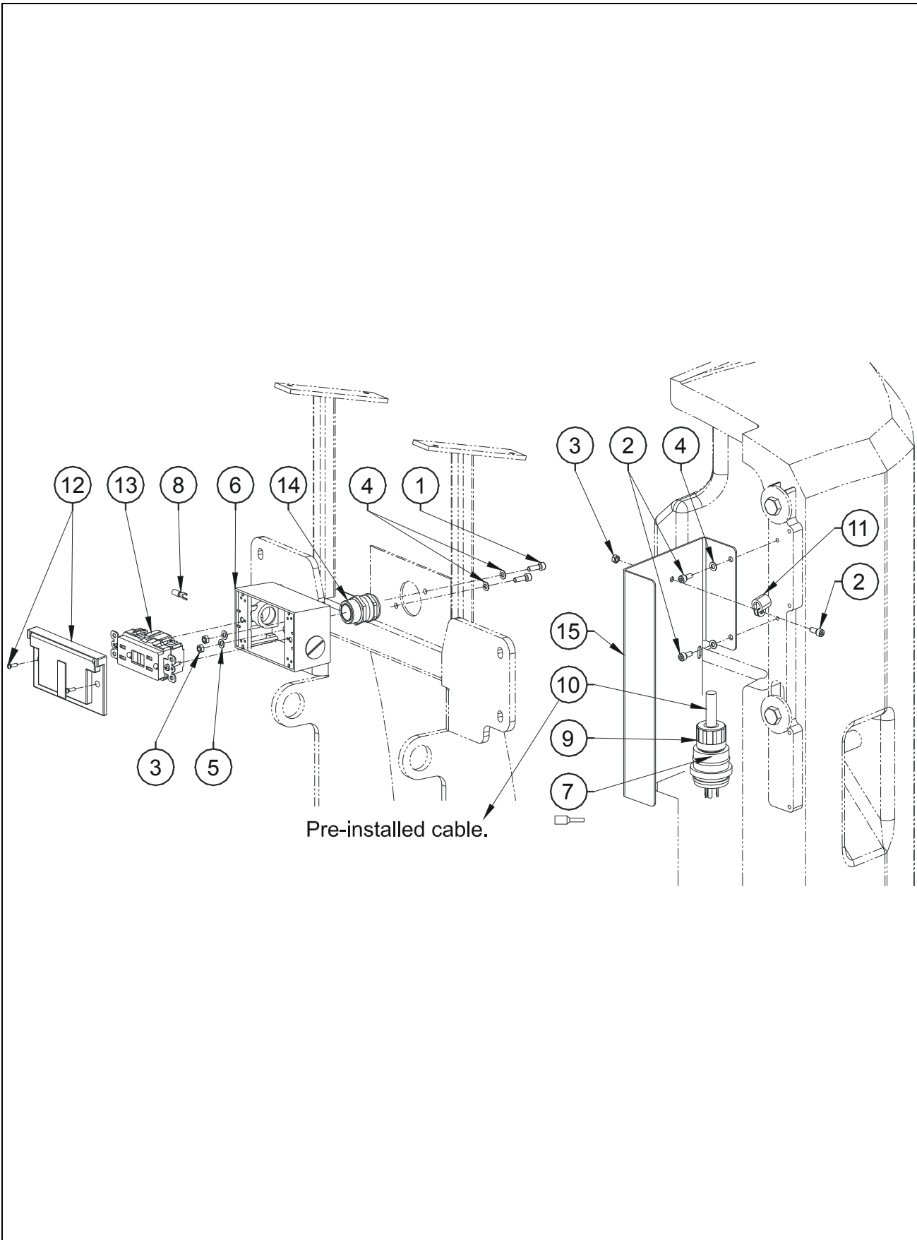
FIGURE 8-6. 115V US PLATFORM SOCKET INSTALL / INSTALLATION PRISE US 115V
