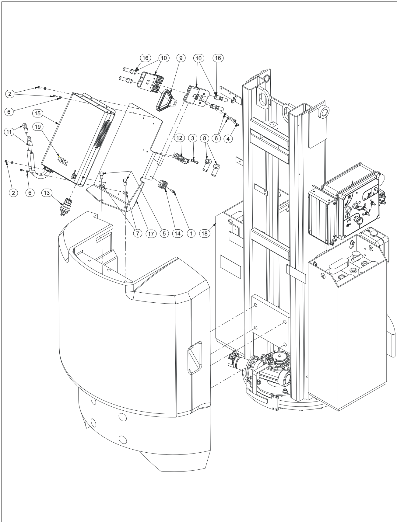
FIGURE 6-1. HIGH FREQUENCY CHARGER INSTALL / INSTALLATION CHARGEUR HAUTE FREQUENCE
