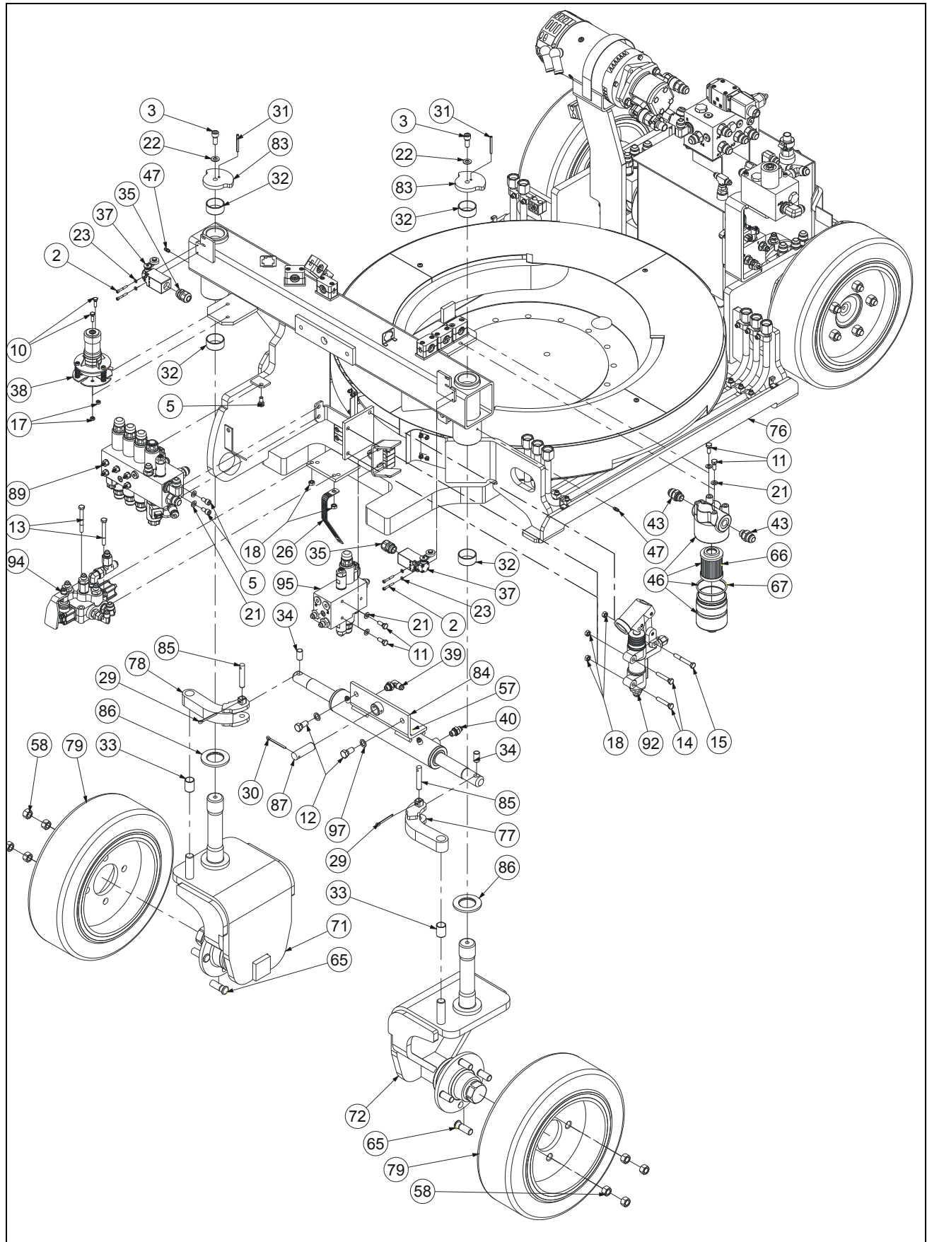
FIGURE 4-1. CHASSIS INSTALL / INSTALLATION CHASSIS
