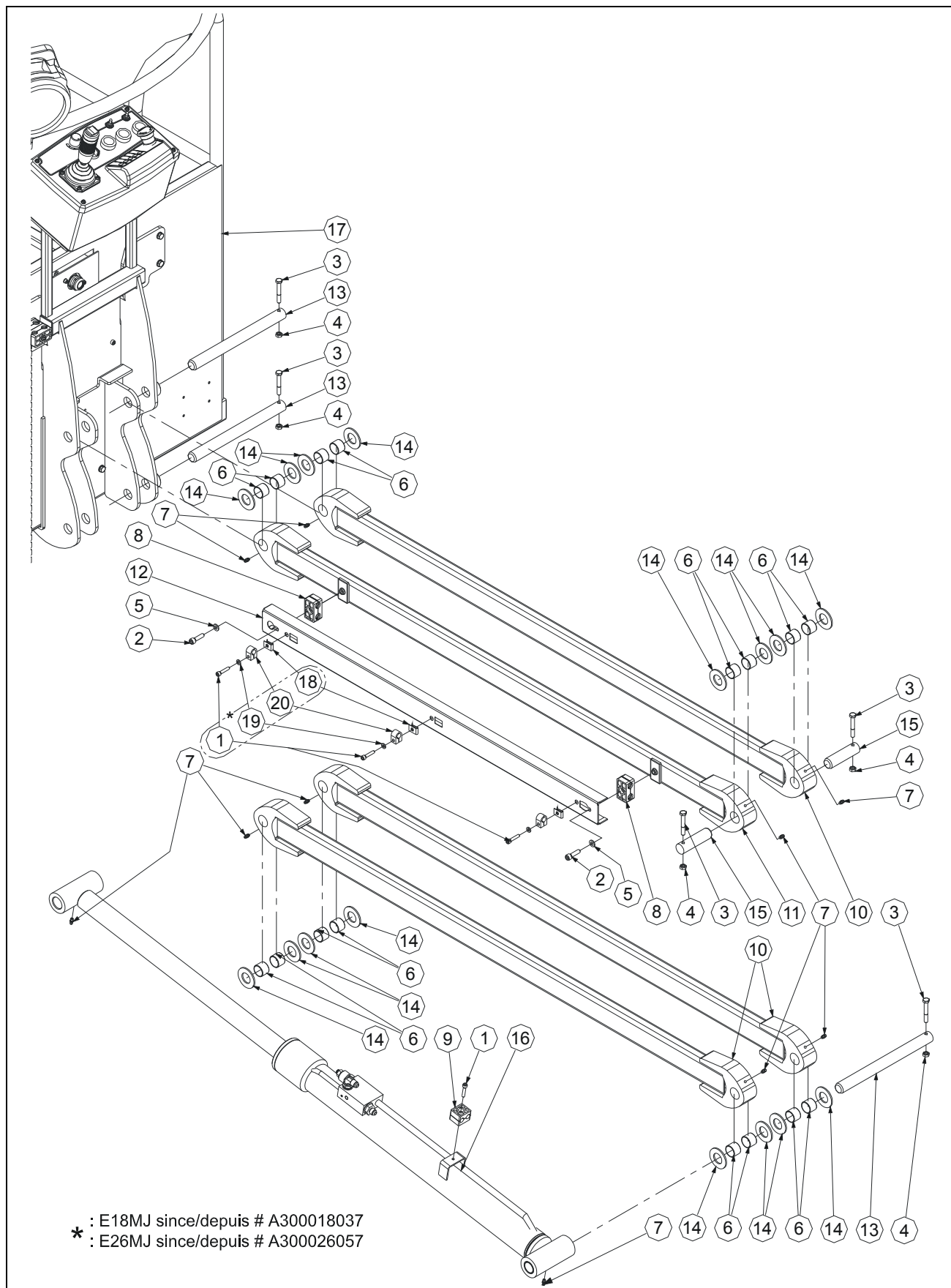
FIGURE 5-1. JIB INSTALL / INSTALLATION BRAS
