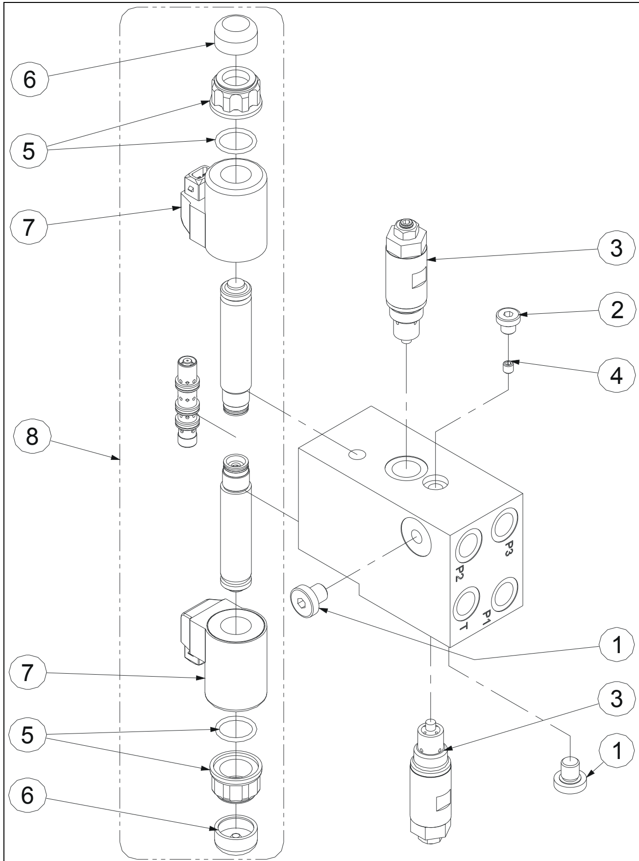
FIGURE 4-1-8-1. STEERING MANIFOLD / BLOC DIRECTION
