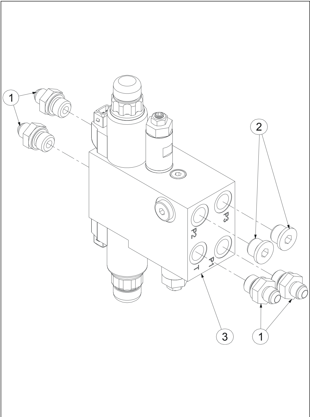
FIGURE 4-1-8. STEERING MANIFOLD ASSEMBLY / ASSEMBLAGE BLOC DIRECTION
