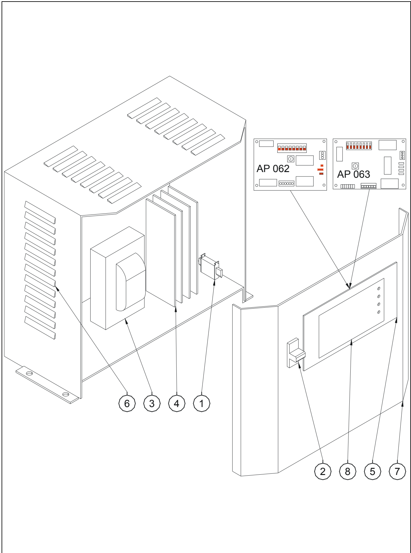
FIGURE 6-3. 115/230V 50A OLDHAM CHARGER / CHARGEUR OLDHAM
