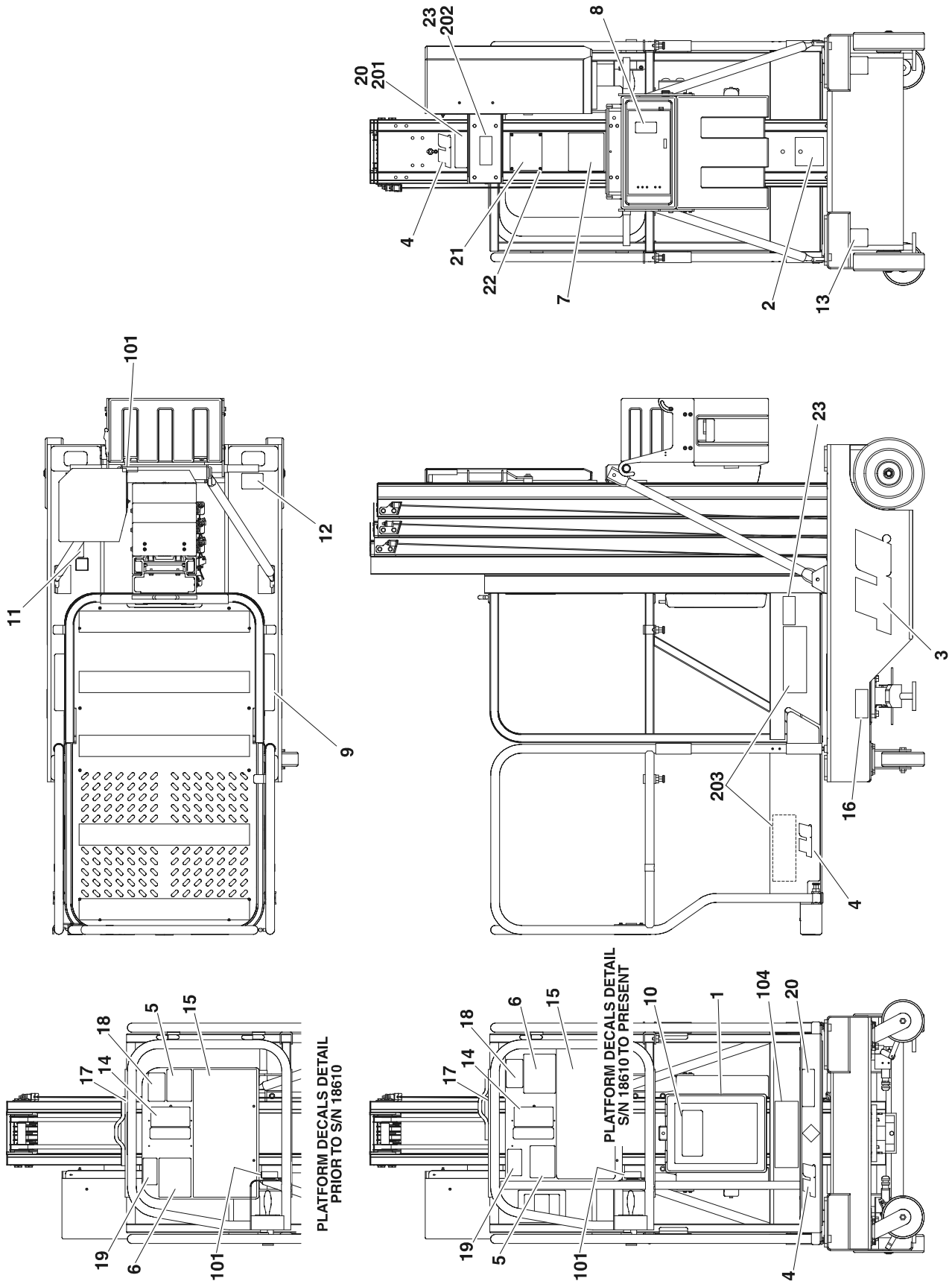
FIGURE 8-1. DECAL INSTALLATION
