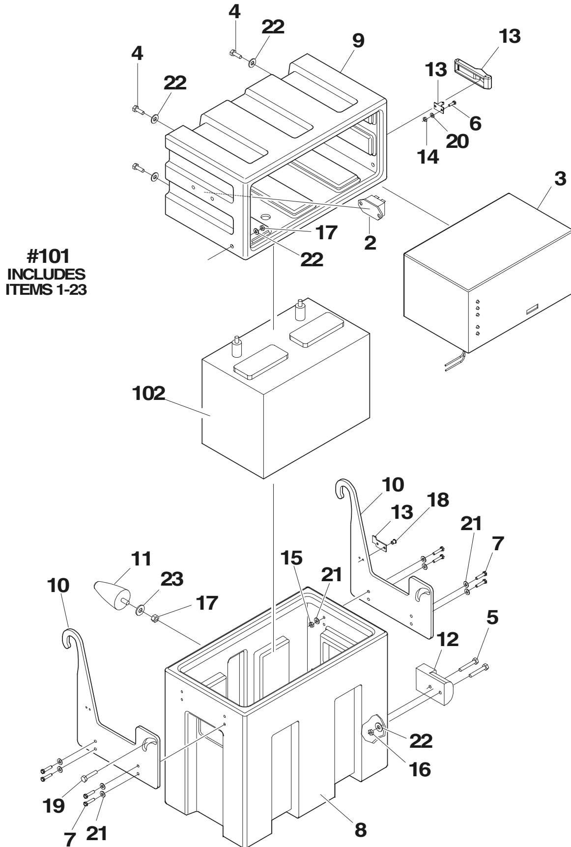
FIGURE 2-3. BATTERY CHARGER INSTALLATION
