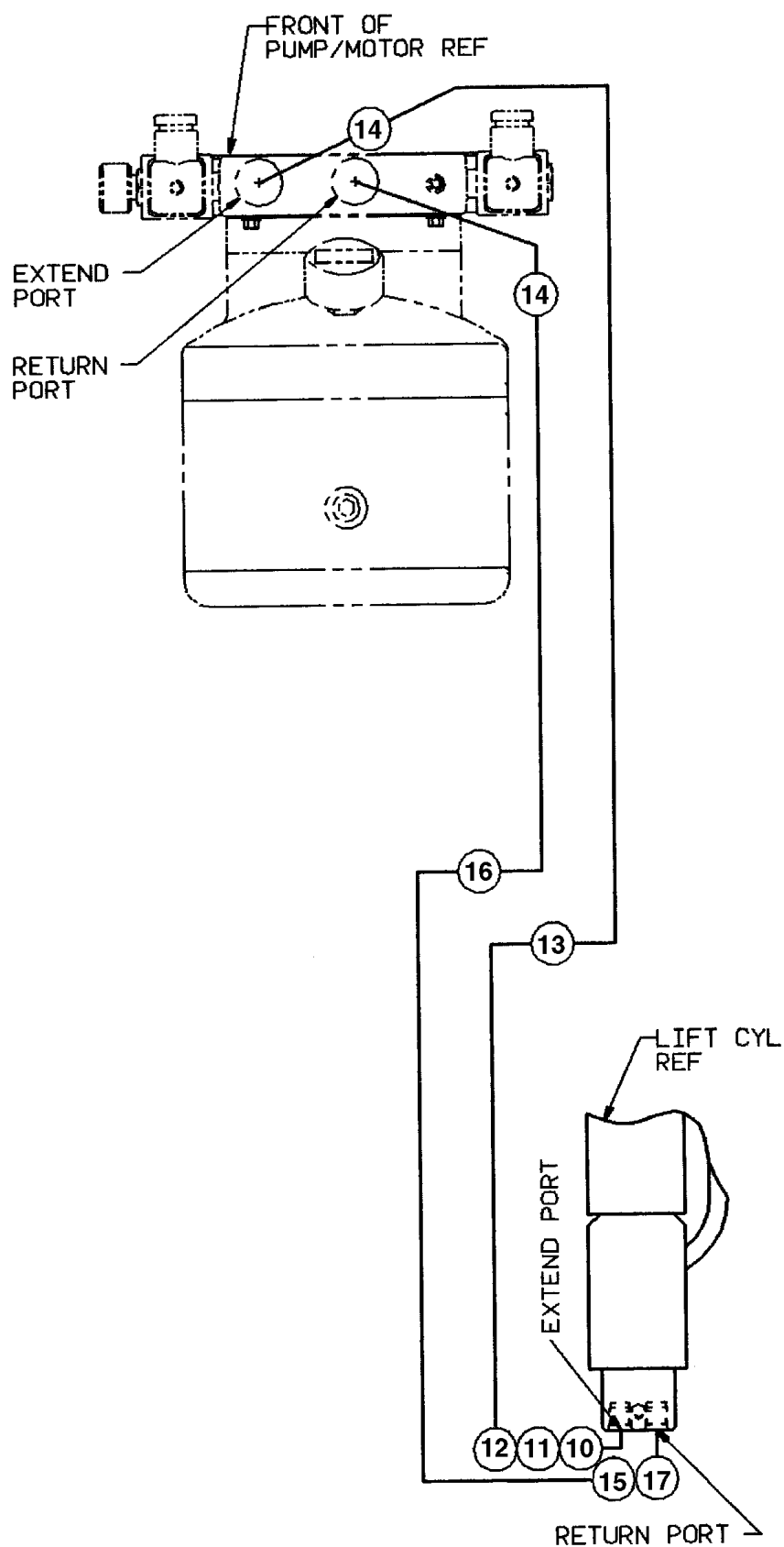
FIGURE 6-1. HYDRAULIC DIAGRAM
