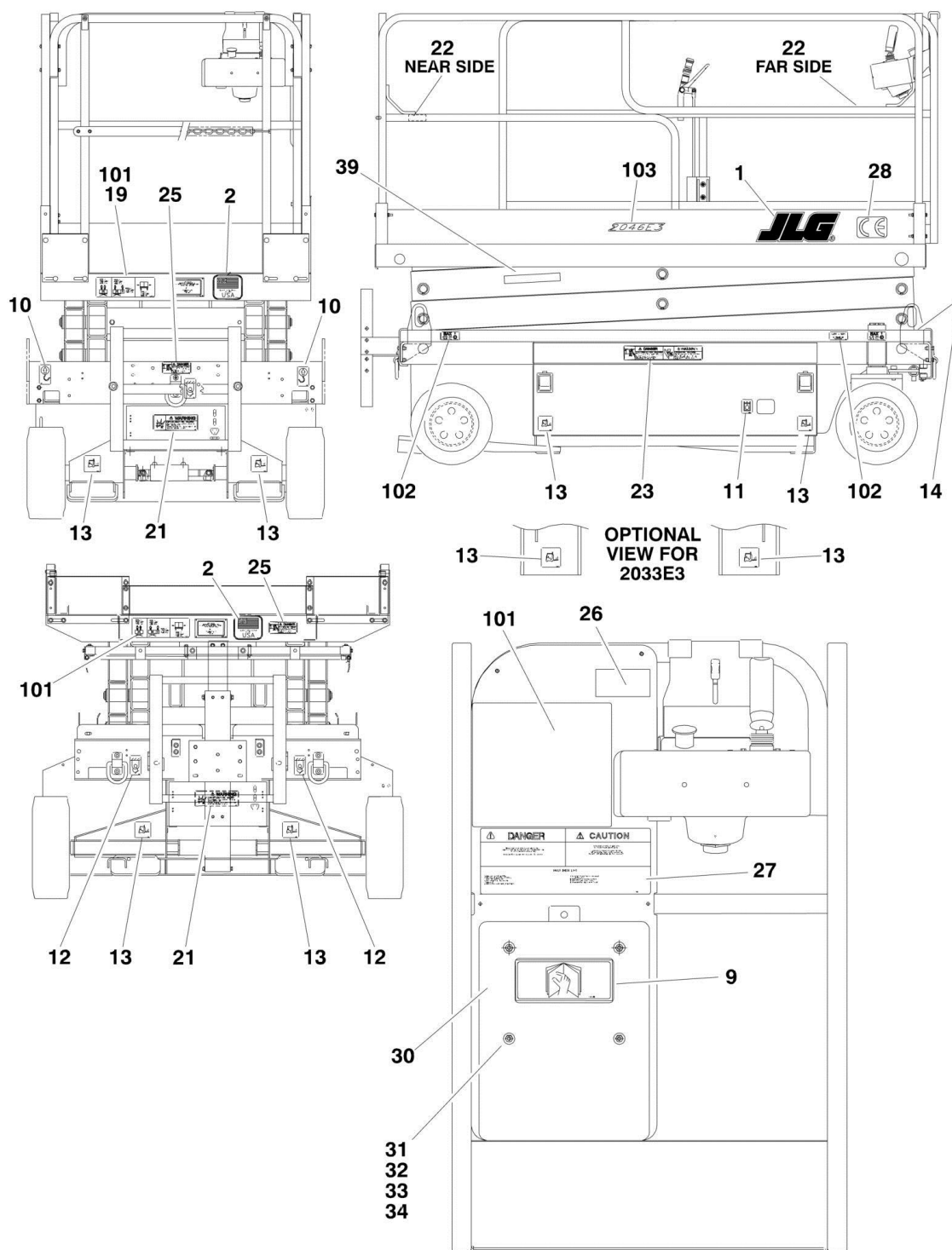
MACHINE WITH FIXED HANDRAILS
